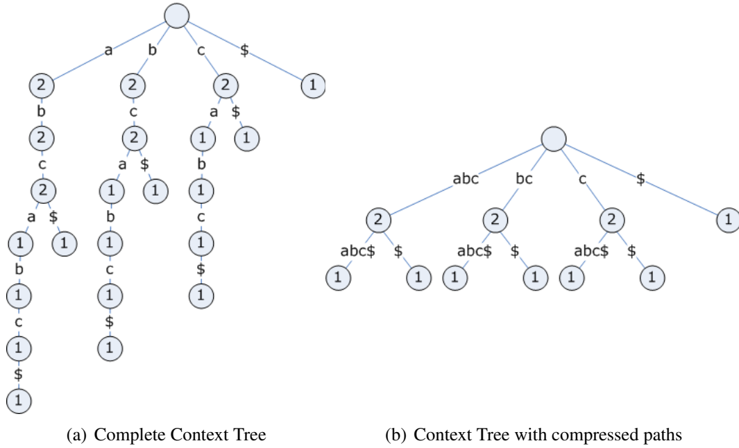
Figure 2.3: Context Trees for string "abcbabc$"
