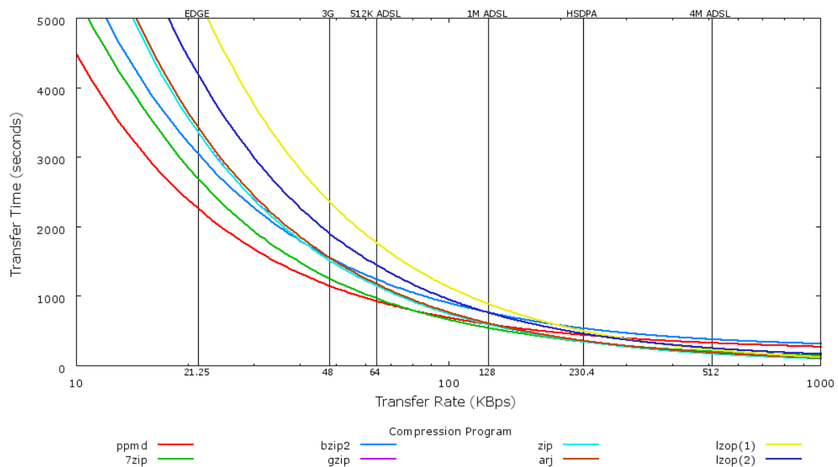
Figure 3.2: Lowest transfer times for all compression programs at transfer speed between 10 KBps and 1000 KBps
