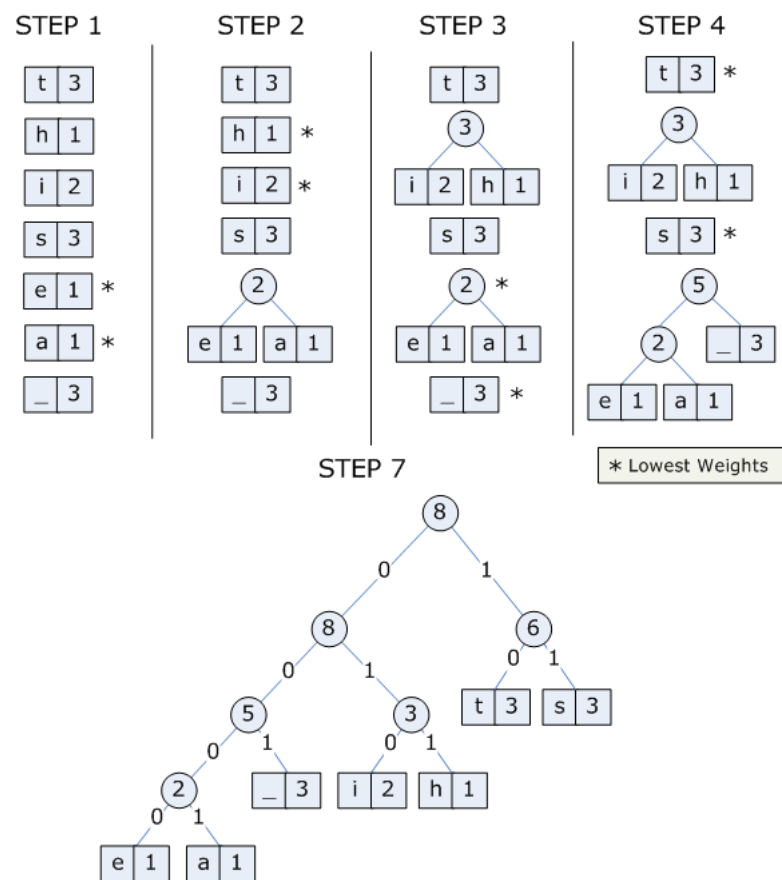
Figure 2.1: Huffman tree for the string "this is a test"
