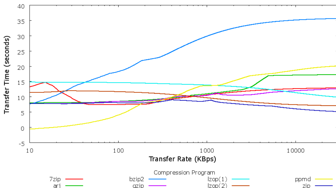
Figure 5.6: Average percentage improvement in the fastest transfer time by compression programs when using preprocessors
