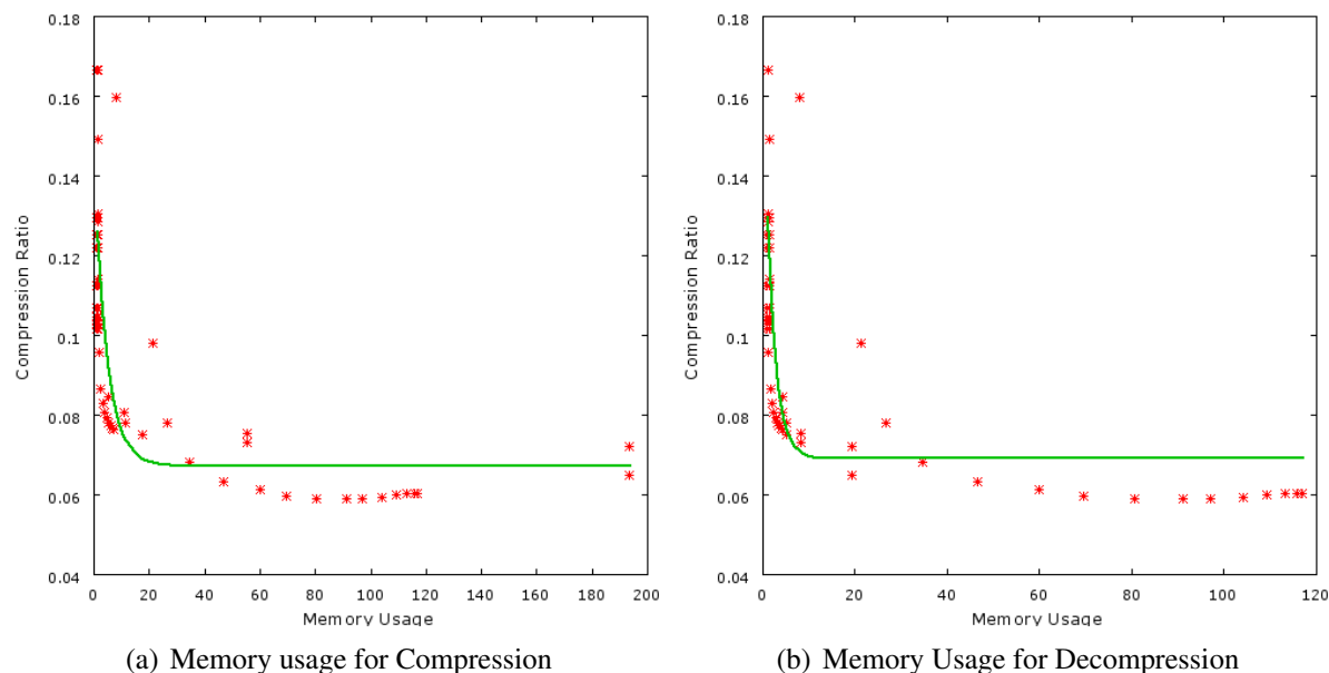
Figure 3.4: Compression Ratio versus Memory Utilisation for all compression levels of all compression programs
