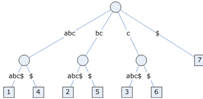
Figure 2.2: Suffix tree for the string "abcabc$"
