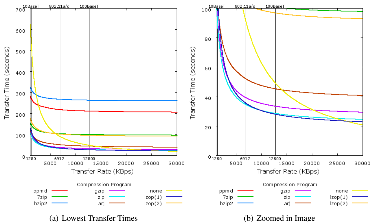
Figure 3.3: Lowest transfer times for all compression programs at transfer speed between 1000 KBps and 30000 KBps
