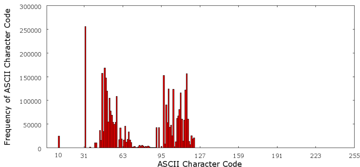
Figure 5.1: Character Distribution of the 3MB maillog file
