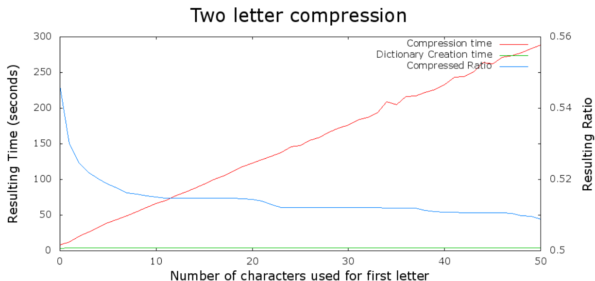
Figure 5.2: Compressed size and compression time for 3MB log file when using longer codes
