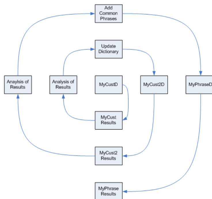
Figure 6.1: Spiral model for developing final custom dictionary
