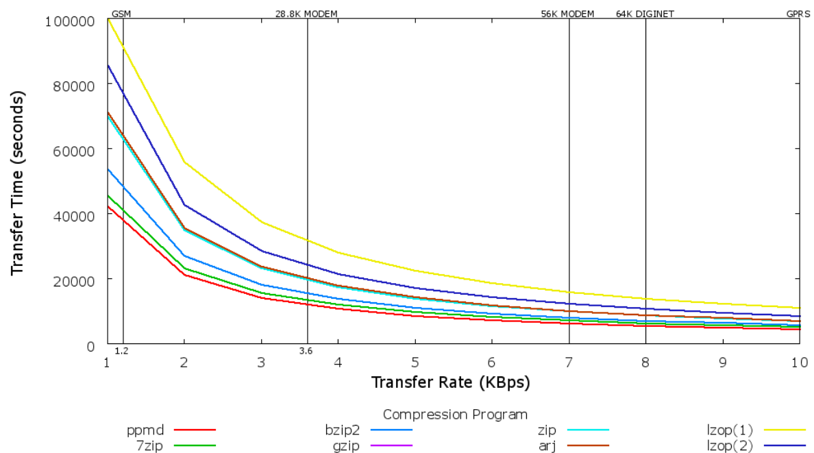
Figure 3.1: Lowest transfer times for all compression programs at transfer speed between 1 KBps and 10 KBps
