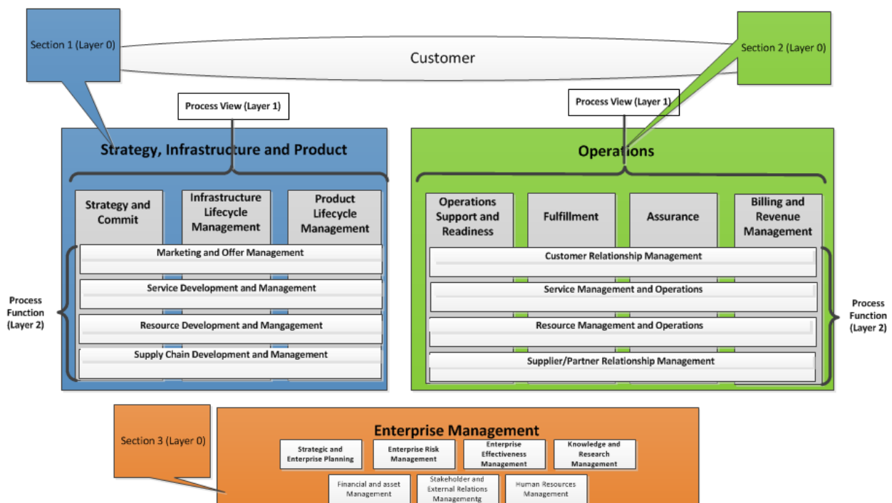
Figure 4-1: eTOM layout
