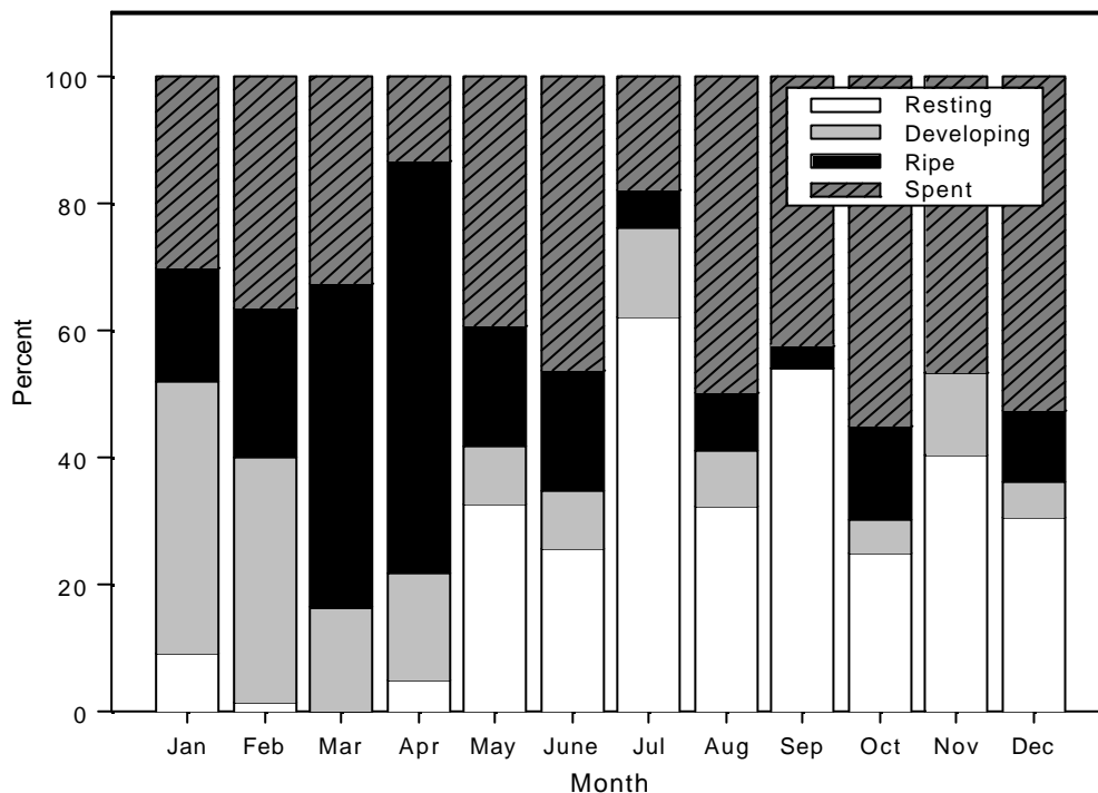
Figure 4.1: Female monthly maturity stages for Diplotaxodon limnothrissa sampled from the southeast arm of Lake Malawi (n = 604).
