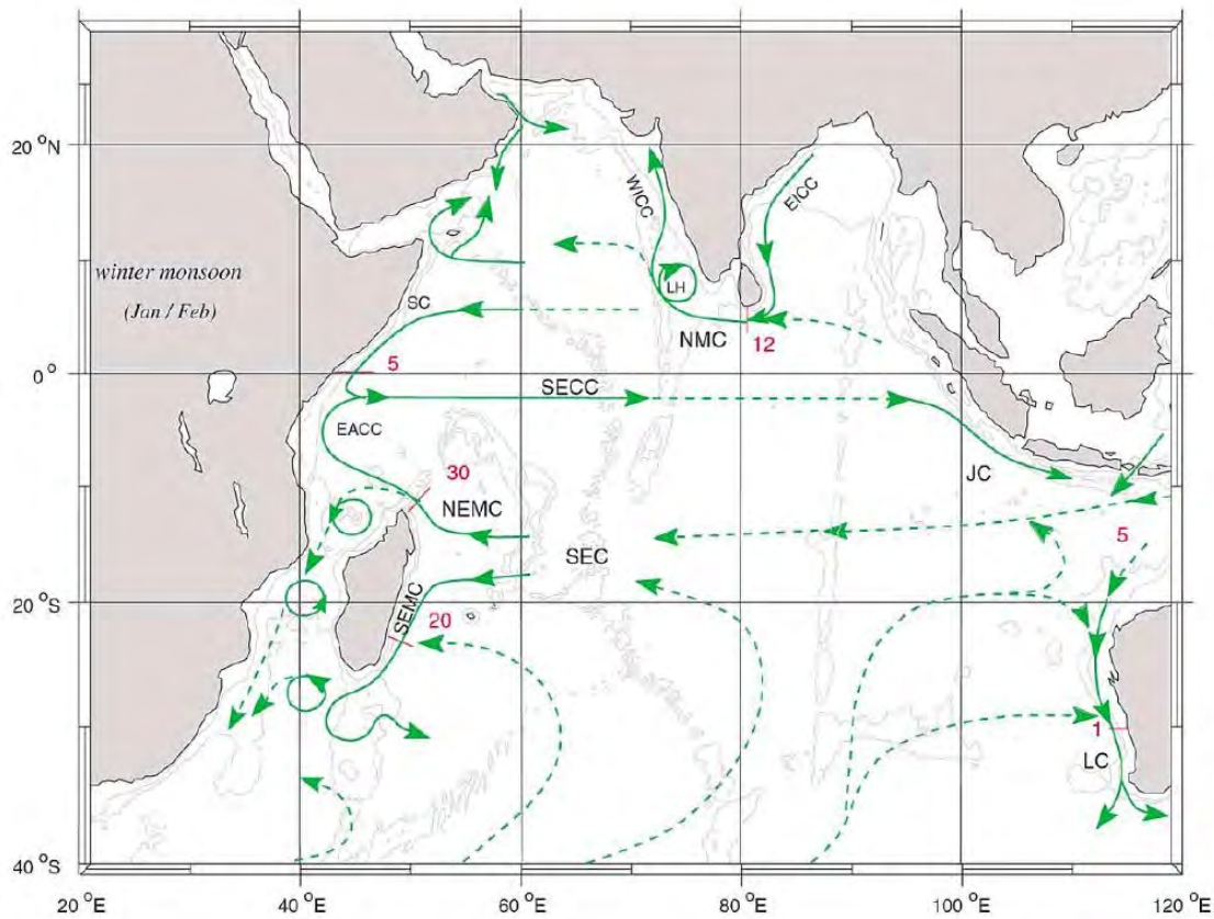
Figure 2.2. A schematic representation of ocean current branches during the Northeast Monsoon, including some choke point transport numbers (Schott and McCreary, 2001).
