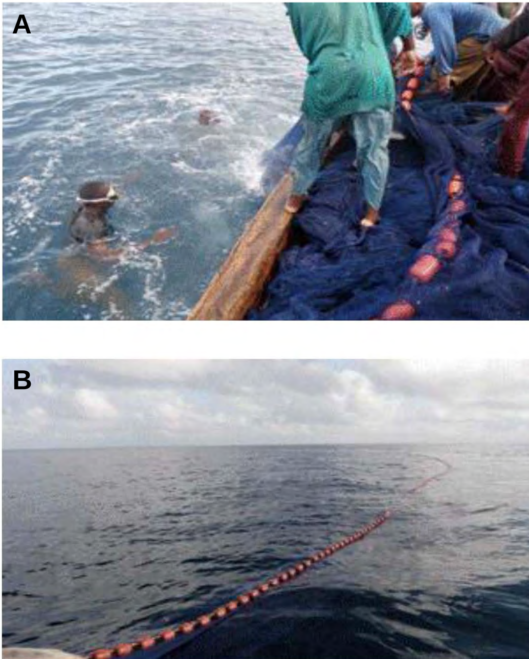
Figure 2.15. Ring net in use; a team of fishers deploying a ring net (A) and a ring net suspended by a string of light buoys (B).
