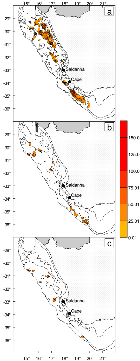
Fig. 5.7: Abundance (number caught per hour) of a) juvenile ( < L_{50} , 37 cm TL), b) sub-adult ( L_{50} - L_{100} , 37-47 cm TL) and c) adult ( > L_{100} , 47 cm TL) L. vomerinus in summer (Jan/ Feb) as estimated from data collected during research surveys ( n = 1112 ) on the west coast of South Africa between 1986 and 1997.
