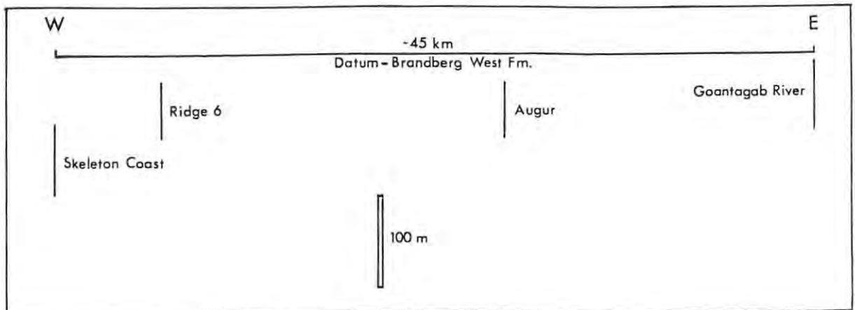
Fig. 3.23: Relative stratigraphic position of the sections measured in the Zebra River Formation with the base of the Brandberg West Formation as a datum.
