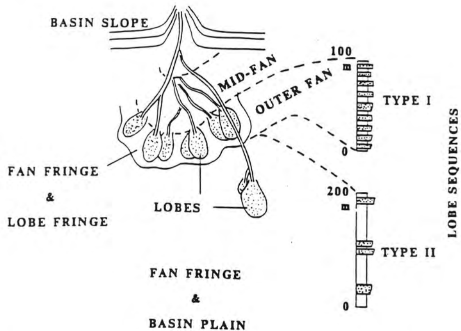
Fig. 3.18: Submarine fan model showing different types of lobe sequences as defined by Pickering (1981). Type I sequences develop by continual switching and stacking of lobes to produce sand dominated sequences, whereas intermittent, irregular progradation of lobes over the basin plain produces mud-rich sequences, or type II (from Pickering, 1981, his Fig. 9).
