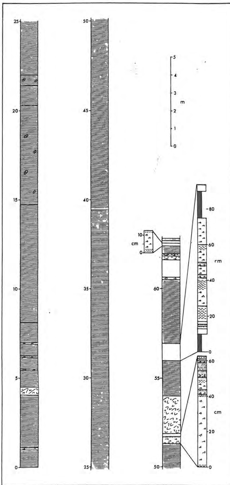
Fig. 3.19: Sedimentary log of the Goantagab River section of the Zebrapüts Formation (see back pocket).
