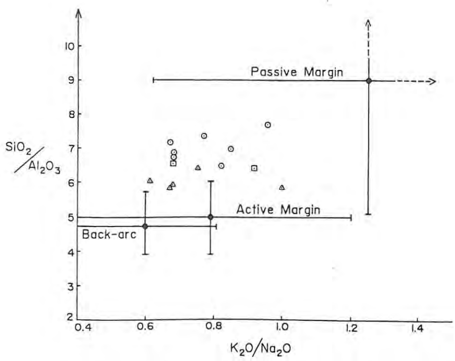
Fig. 4.7: Chemistry of modern deep-sea sands compared with that of the Zerrissene greywackes. Extensive overlap of modern sands from different tectonic settings occurs and it is therefore difficult to categorise the ancient greywackes. The error bars on the modern analyses are one standard deviation each side of the mean (from Maynard et al. , 1982). Symbols as for Fig. 4.4.
