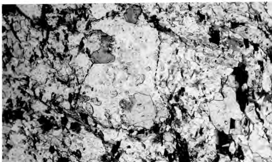
Fig. 4.3: Tourmaline is the most common detrital mineral, but is not useful for provenance studies as it is polycyclic. However rare inclusions of tourmaline grains in a granitic fragment (outlined) such as these shown here indicate that they were derived from a granitic source (sample UR 20/87).
