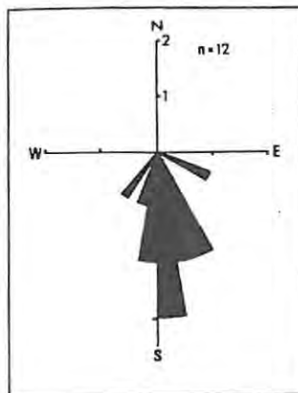
Fig. 4.13: Palaeocurrent rose diagram (in 10^0 sectors) for the Amis River Formation. The direction of sediment transport is dominantly from north to south.
