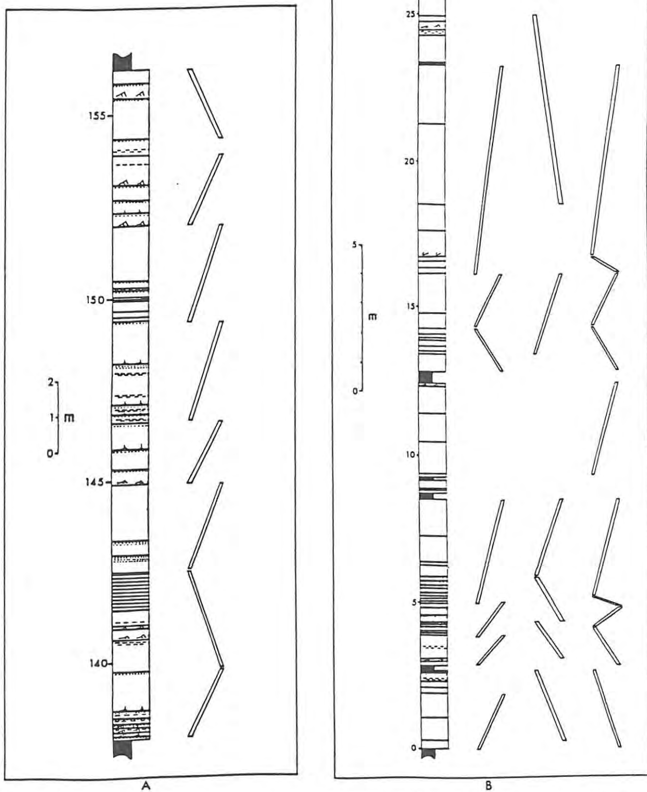
Fig. 3.41: A: Portion of Fig. 3.40 showing asymmetric cycles which comprise only a few beds. These are similar to the compensation cycles of Mutti and Sonnino (1981). B: Basal portion of the Jeppe east section showing different possible interpretations of cycles. Cycles shown as in Fig. 3.31.
