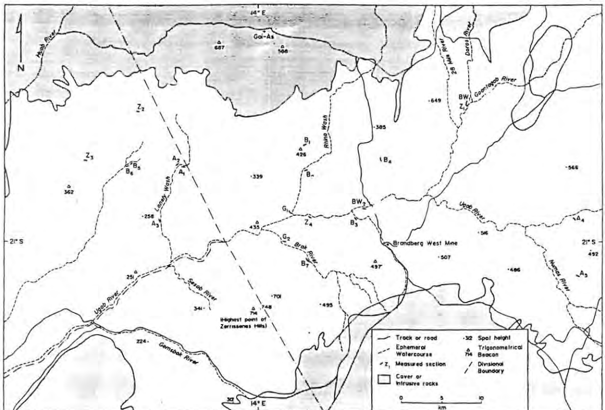
Fig. 1.4: Map of the lower Ugab River area showing major drainage lines, topographic features, routes and localities of measured sections. Section symbols are: Z1 - Goantagab River; Z2 - Ridge 6; Z3 - Skeleton Coast Park; Z4 - Augur; BW1 - Ulundi; BW2 - Ugab River; B1 - Shelter; B2 - Rhino Wash; B3 Zebra River; B4 - Gai-as South; B5 - Gemsbok Altar East; B6 - Gemsbok Altar West; B7 - Brak River; G1 - Lookout; G2 - Corner; A1 - Jeppe East; A2 - Jeppe West; A3 - Lonely River; A4 - Bee; A5 - Tributary.
