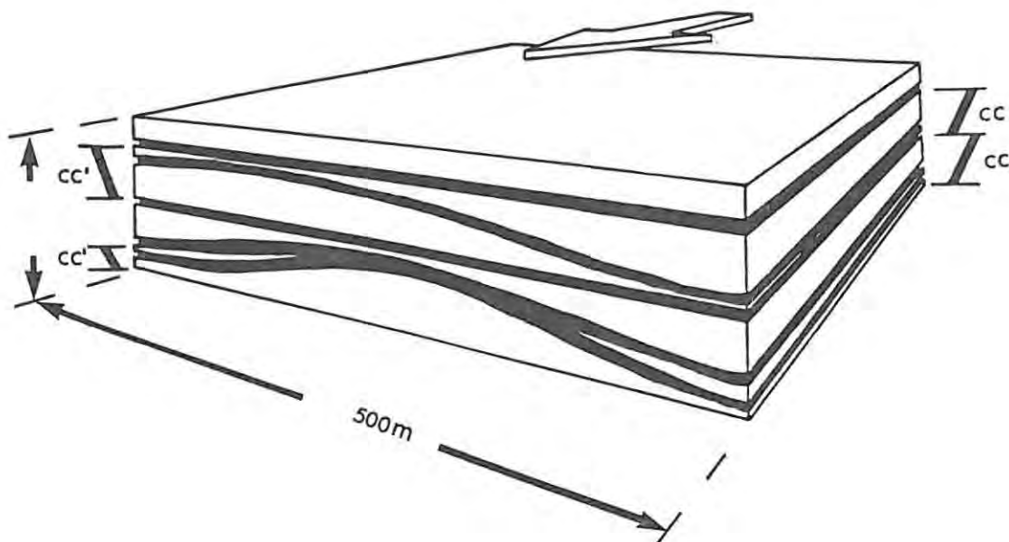
Fig. 3.33: A: Development of thickening-upward compensation cycles according to Mutti and Sonnino (1981), with modifications indicating how the same set of beds can develop thinning-upward cycles (cc').
