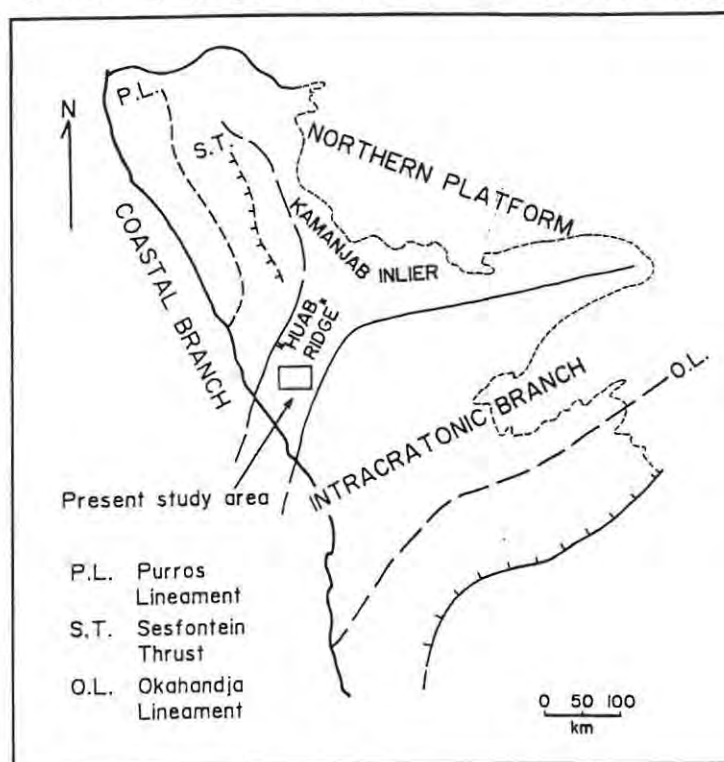
Fig. 1.10: Map showing position of assumed "Huab Ridge" of Porada (1983). This basement high is situated over the current study area.
