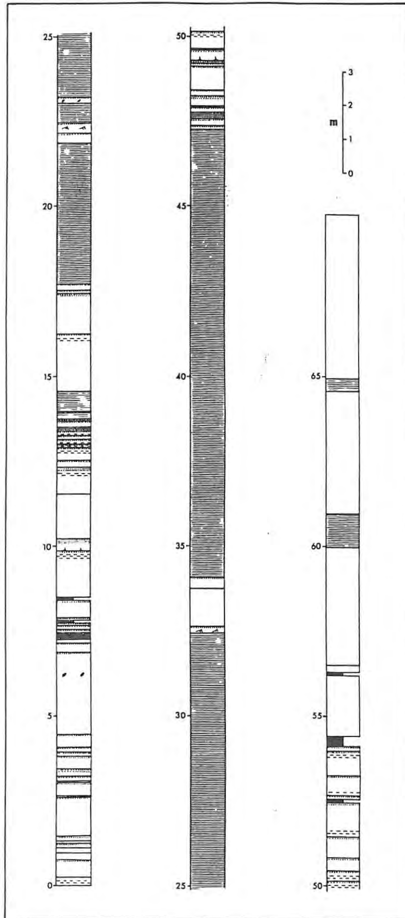
Fig. 3.21: Sedimentary log of the Augur section of the Zebrapüts Formation. See Fig. 3.22 for a photograph of this section.
