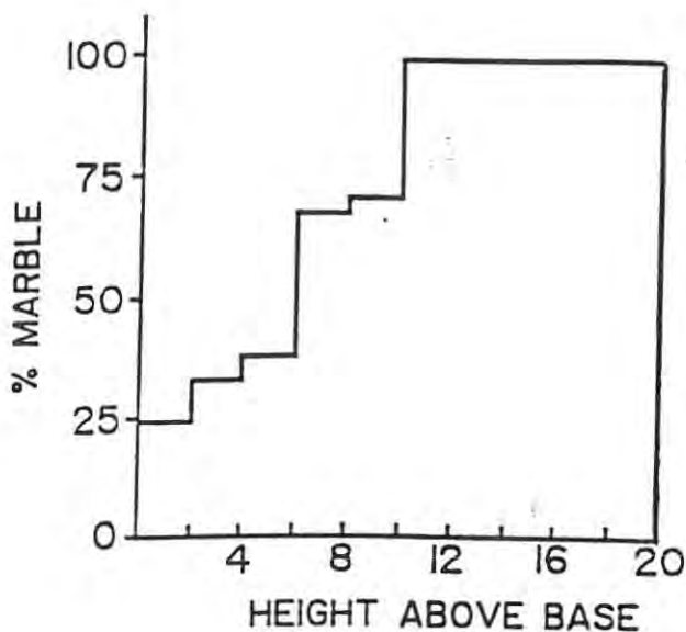
Fig. 2.13: Histogram showing the progressive increase in carbonate content with height in the section depicted in Fig. 2.10. Percentage carbonate determined from measured sections.
