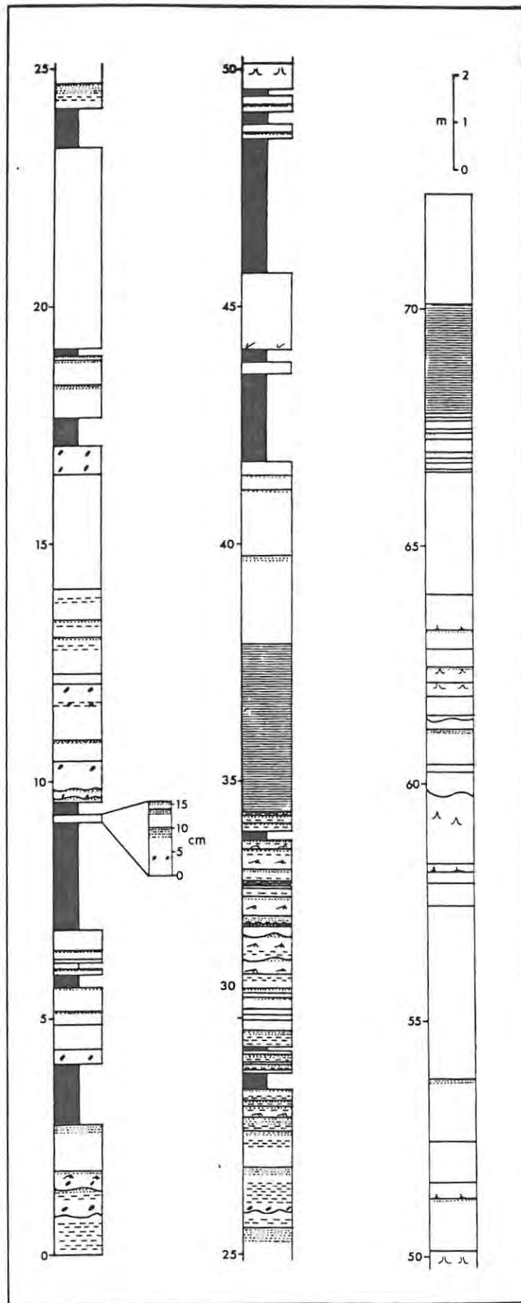
Fig. 3.44: Sedimentary log of the Jeppe west section. This section is dominated by facies D 1 and D 2 , with rare facies B 1 beds.
