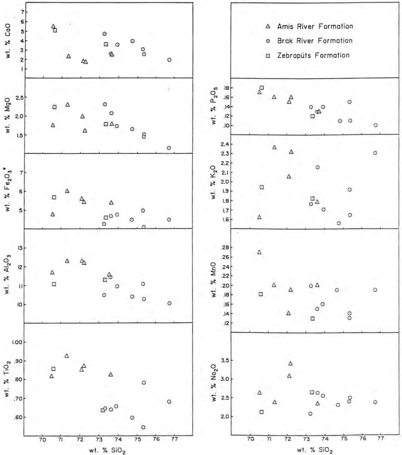
Fig. 4.4: Harker variation diagram for the analysed samples of Zerrissene greywackes.
