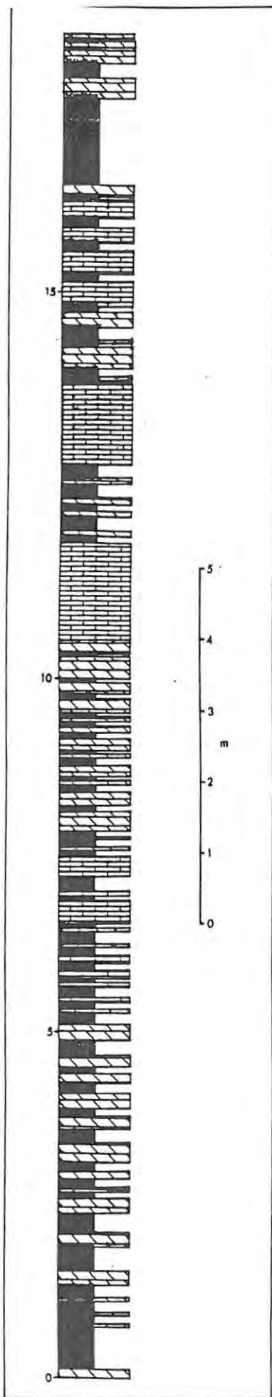
Fig. 2.10 (above): Sedimentary log of the Ugab section
