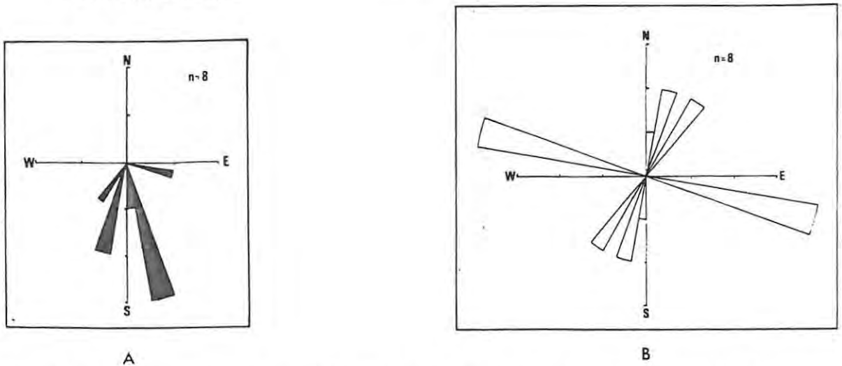
Fig. 4.12: Palaeocurrent rose diagrams (in 10^0 sectors) for the Brak River Formation. A: Directional structures; B: Trend only. A strong component of transport from the north and west is apparent.
