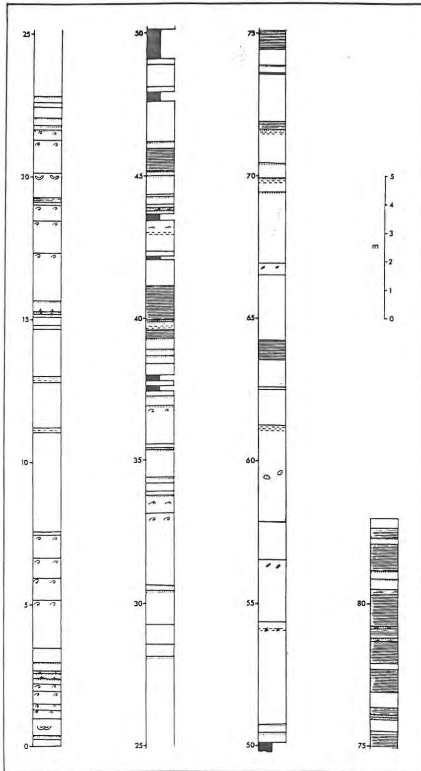
Fig. 3.34: Sedimentary log of the Gemsbok Altar west section of the Brak River Formation. The sequence here is characterised by a lack of pelitic material.
