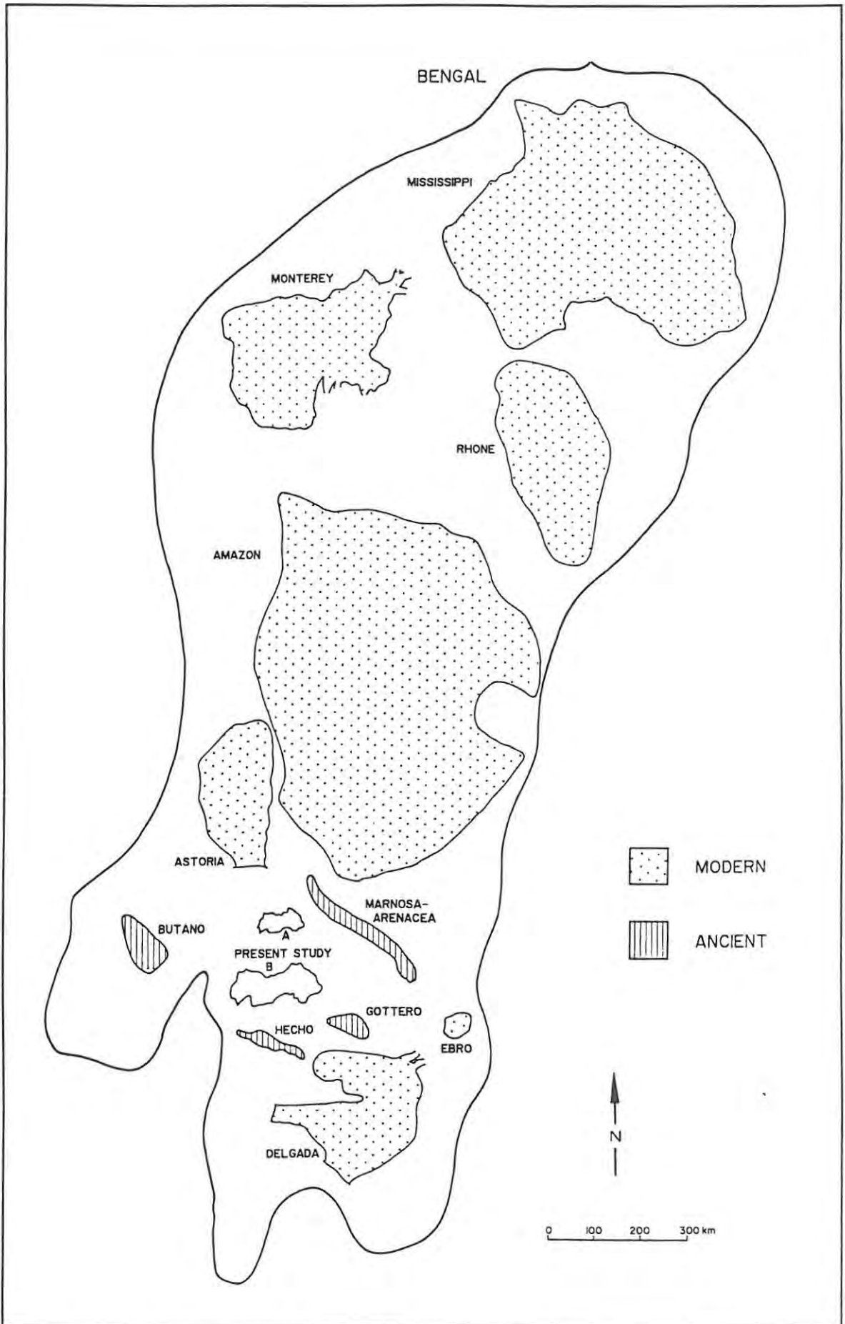
Fig. 1.8: Diagram comparing sizes of modern and ancient fans. The Zerrissene system is depicted showing the current outcrop area (A) and after unfolding assuming at least 50 per cent shortening (B).
