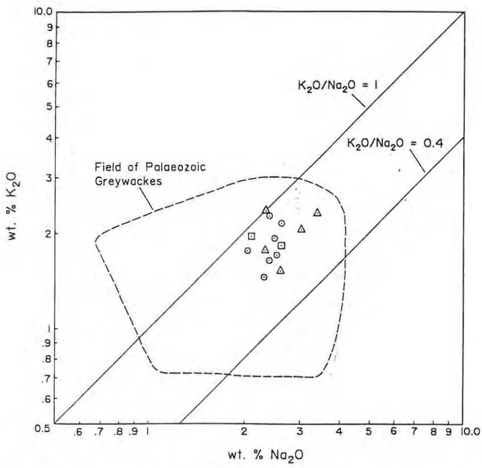
Fig. 4.6: The composition of the Zerrissene greywackes is typical for Palaeozoic greywackes (modified from Crook, 1974 and Floyd and Leveridge, 1987). Symbols as for Fig. 4.4
