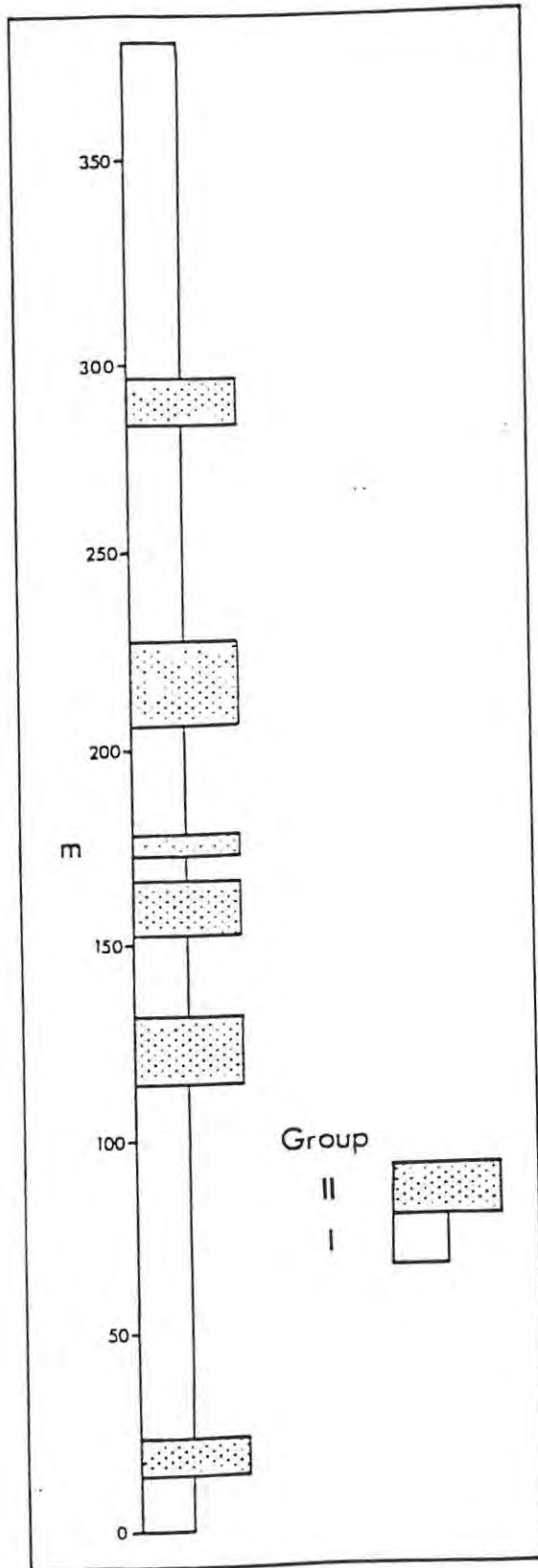
Fig. 3.42 (left): Two common facies associations are found in the Jeppe east section. Group I comprises largely facies D 1 , D 2 and G, while group II is made up of B 1 and D 1 . Fig. 3.43 (right): The group II association, a typical example of which is shown here, comprises largely beds of facies B 1 and D 1 .
