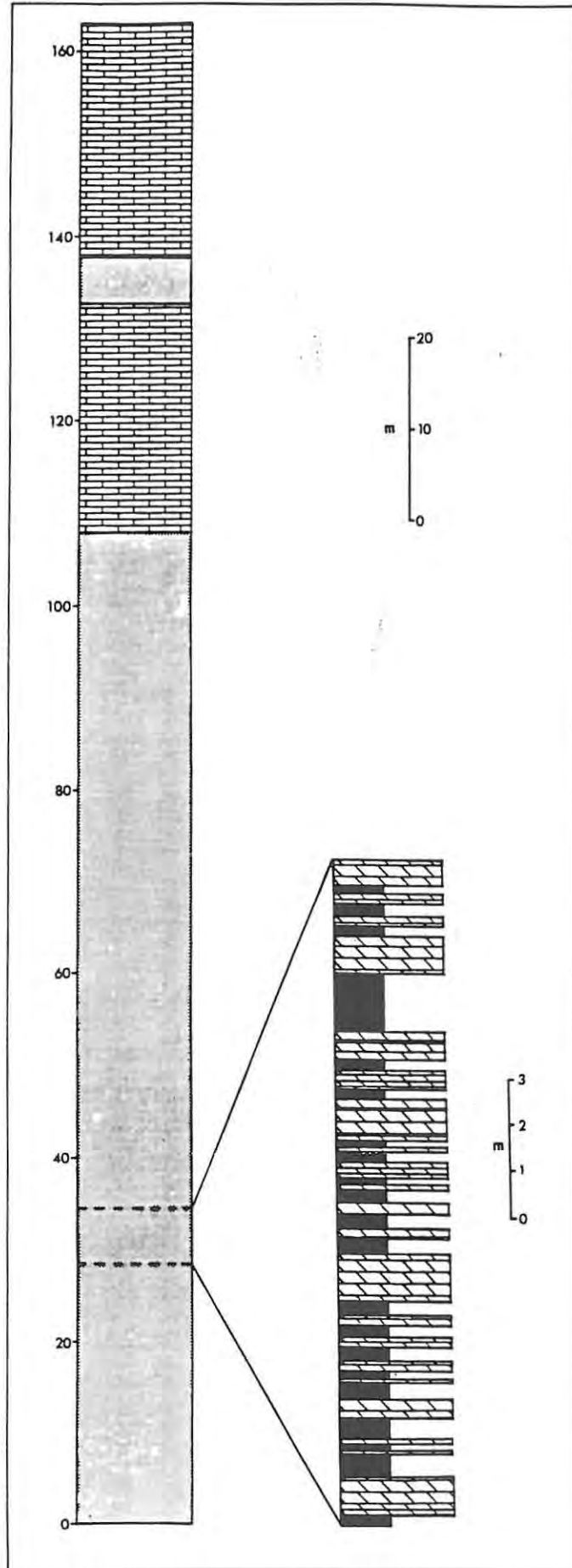
Fig. 2.14: Sedimentary log of the Lookout section through the Gemsbok River Formation (see Fig. 1.4 for locality). Fig. 2.8 is a photograph of the upper portion of this section.
