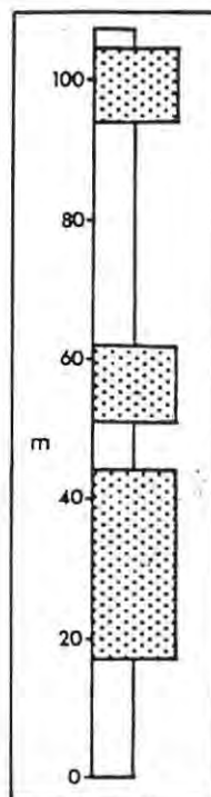
Fig. 3.46: The same facies groups found in the Jeppe east and west sections are found in the Lonely River section. These groupings are shown here. See Fig. 3.42 for key.
