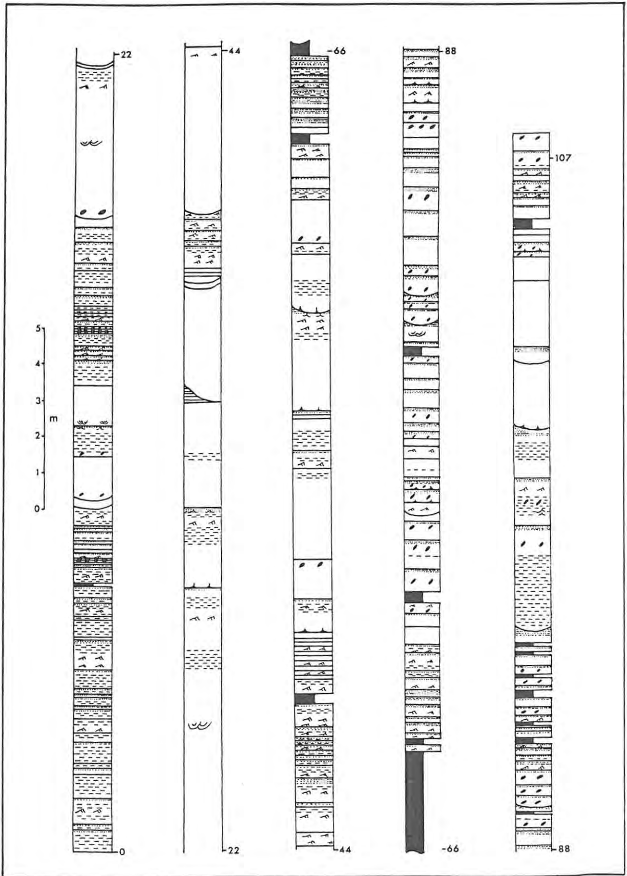
Fig. 3.45 A: The best exposures in the area are found in the Lonely River section, shown here. The section is dominated by facies D 1 beds with packages of facies B 1 . Facies D 2 , E and G are minor in the section. Fig. 3.46 shows the various facies groups.
