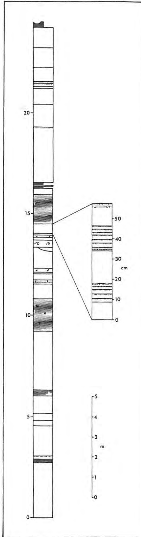
Fig. 3.29: Sedimentary log of the Shelter section of Brak River Formation.
