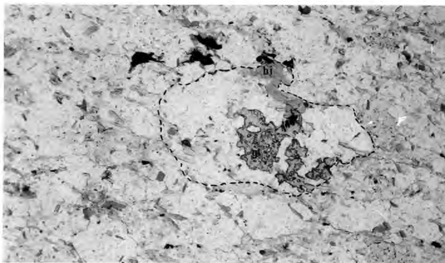
Fig. 4.2: Although no individual detrital garnet grains have been observed, a single clast of quartz-biotite-garnet schist (outlined) is present, and this combined with other metamorphic, igneous and sedimentary clasts indicates a basement - recycled orogen source terrane.
