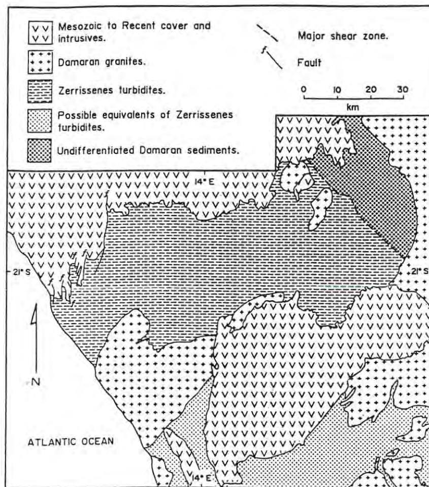
Fig. 1.9: Map showing locality of possible equivalents of the Amis River Formation south of the Mesozoic Karoo cover.
