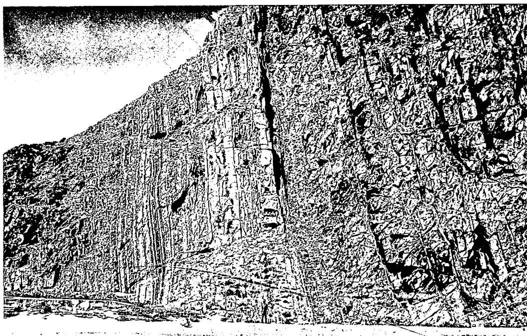
Fig. 2.9: Photograph of the Ugab River measured section
