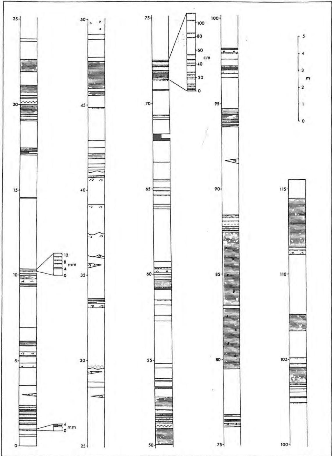
Fig. 3.27: Sedimentary log of the Rhino Wash section. Fig. 3.28 is a photograph of this section. Note the very thinly bedded facies D 1 units interbedded with facies B 1 (see back pocket).
