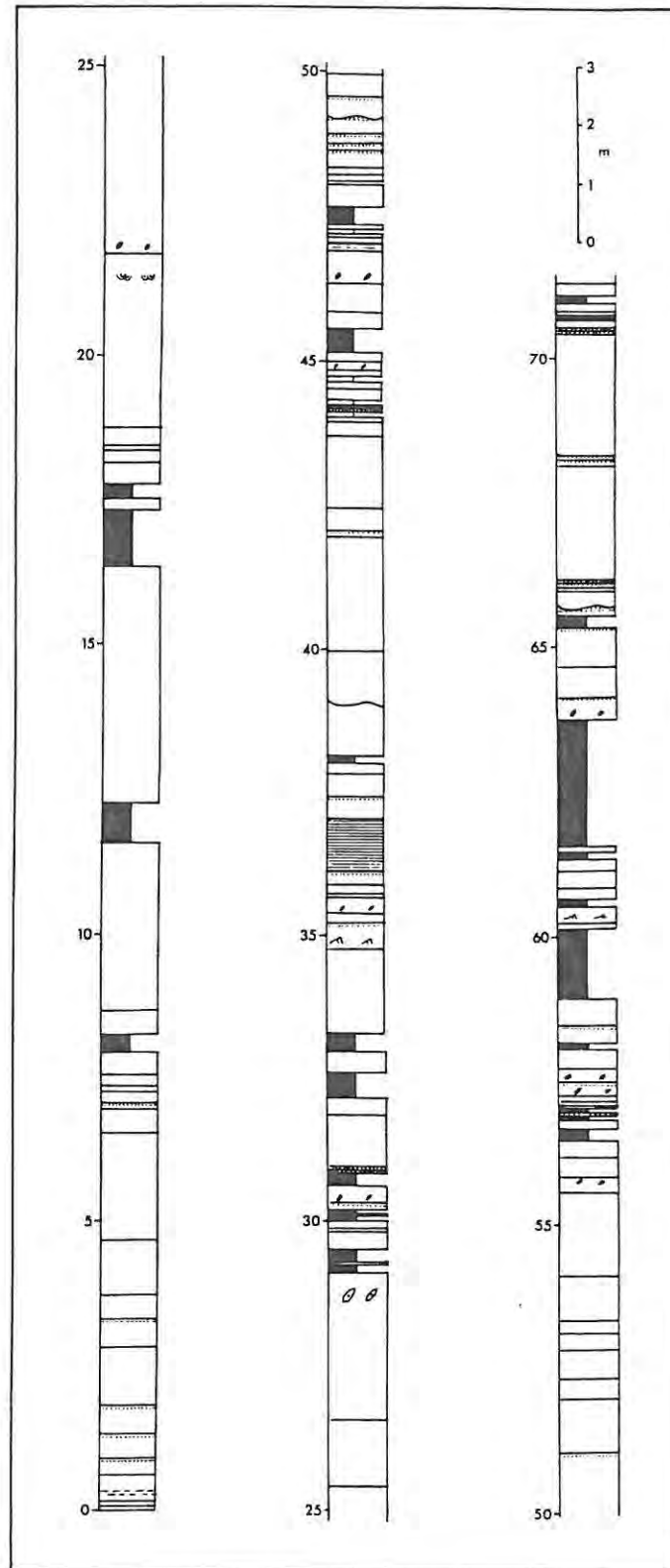
Fig. 3.20: Sedimentary log of the Skeleton Coast Park section of the Zebrapüts Formation, which is again dominated by a high sand:shale ratio.
