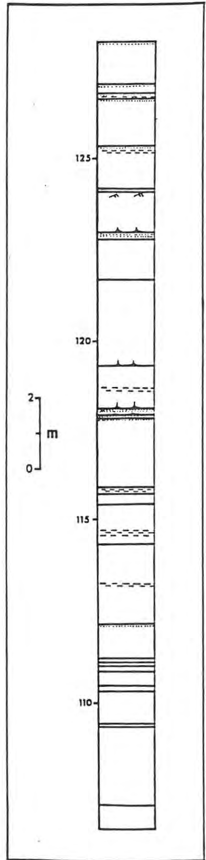
Fig. 3.42 (left): Two common facies associations are found in the Jeppe east section. Group I comprises largely facies D 1 , D 2 and G, while group II is made up of B 1 and D 1 . Fig. 3.43 (right): The group II association, a typical example of which is shown here, comprises largely beds of facies B 1 and D 1 .
