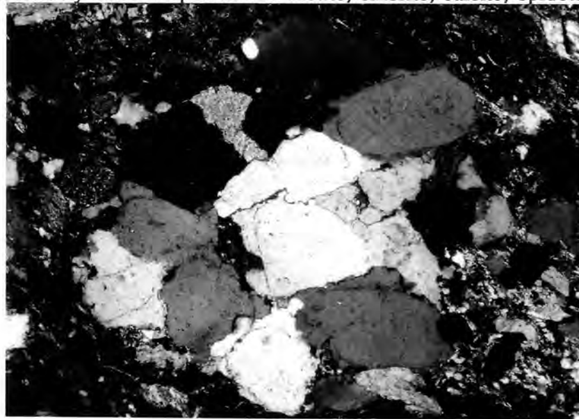
Fig. 4.1: Photomicrograph of a quartz-arenite clast which shows well developed, optically continuous, overgrowths on individual quartz grains (sample UR 6/87).
