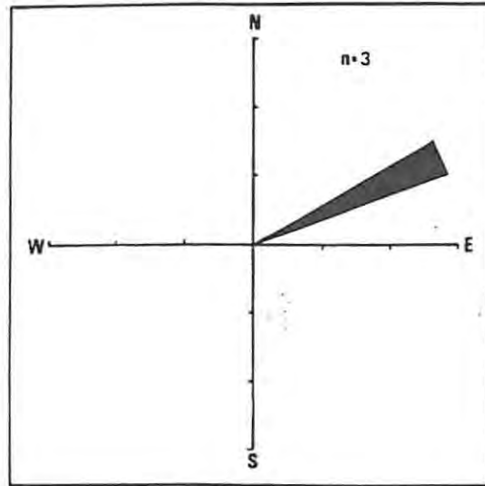
Fig. 4.11: Palaeocurrent rose diagram (in 10^0 sectors) for the Zebra pits turbidites. This formation has few directional structures.
