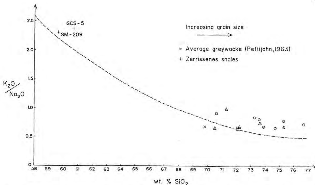
Fig. 4.5: Grain size variations strongly affect the geochemical composition of sediments, with decreasing grain size corresponding to a decrease in SiO 2 , and an increase in the K 2 O/Na 2 O ratio (adapted from Roser and Korsch, 1986). Symbols as for Fig. 4.4.
