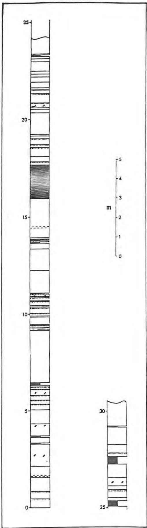
Fig. 3.36: Sedimentary log of the Gai-as south section of the Brak River Formation.
