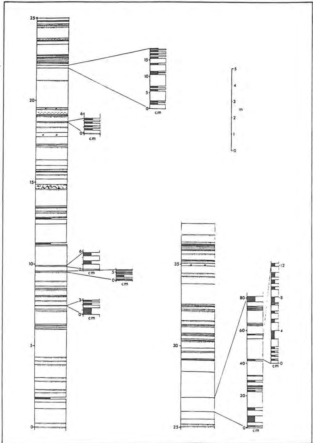
Fig. 3.15: Graphic log of the Ridge 6 section through the Zebrapüts Formation. The section is dominated by facies D 1 with a high sand:shale ratio. Most beds are capped by a very thin pelitic top. For enlarged version of this diagram and the key to all sections of the siliciclastics see Figs. 3.15 and 3.16 in back pocket.
