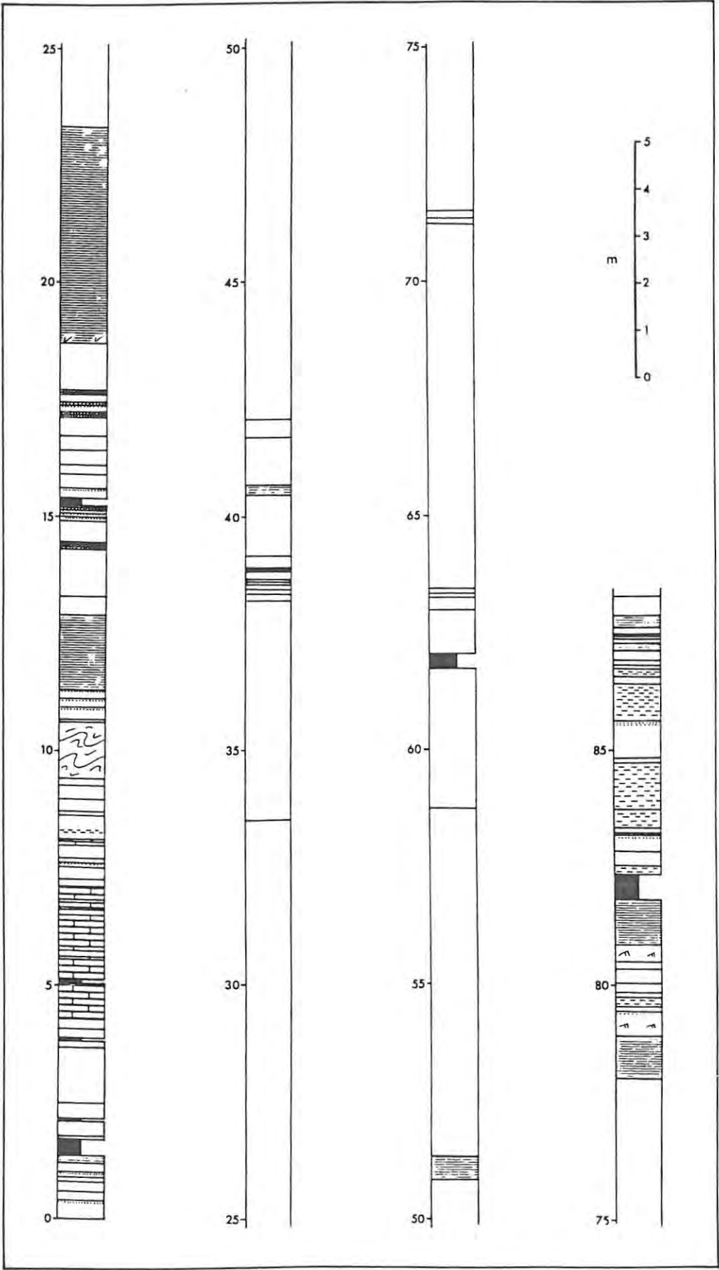
Fig. 3.24: Sedimentary log of the Zebra River section of the Brak River Formation.
