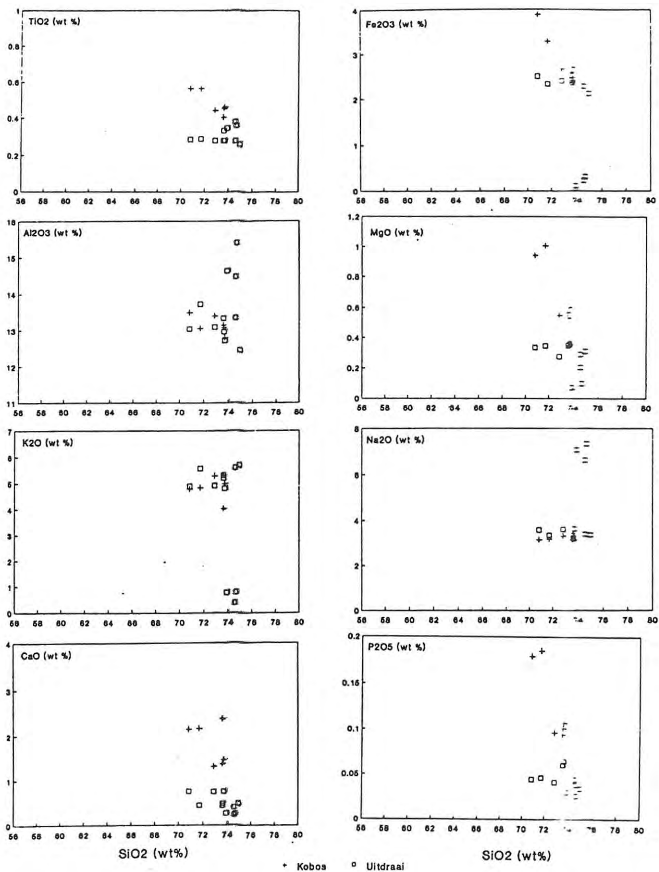
Figure 1.10.3(b) Harker variation diagrams of the Gamsberg Granites
