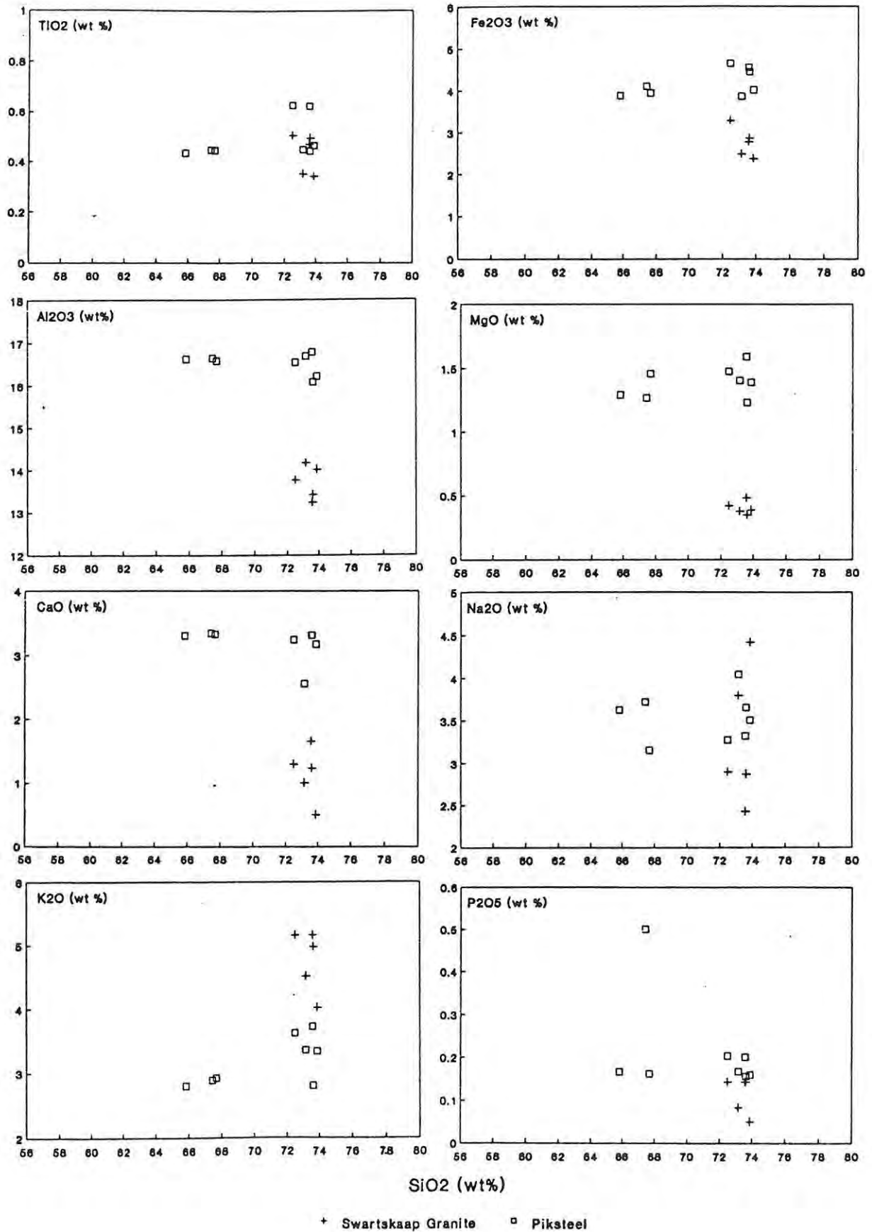
Figure 1.4(b): Harker variation diagrams for the Piksteel Granodiorite and Swartskaap Granite.
