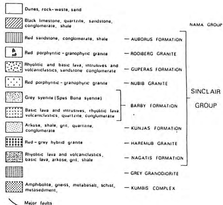
FIGURE 1: GEOLOGICAL MAP OF THE SINCLAIR - HELMERINGHAUSEN AREA*
