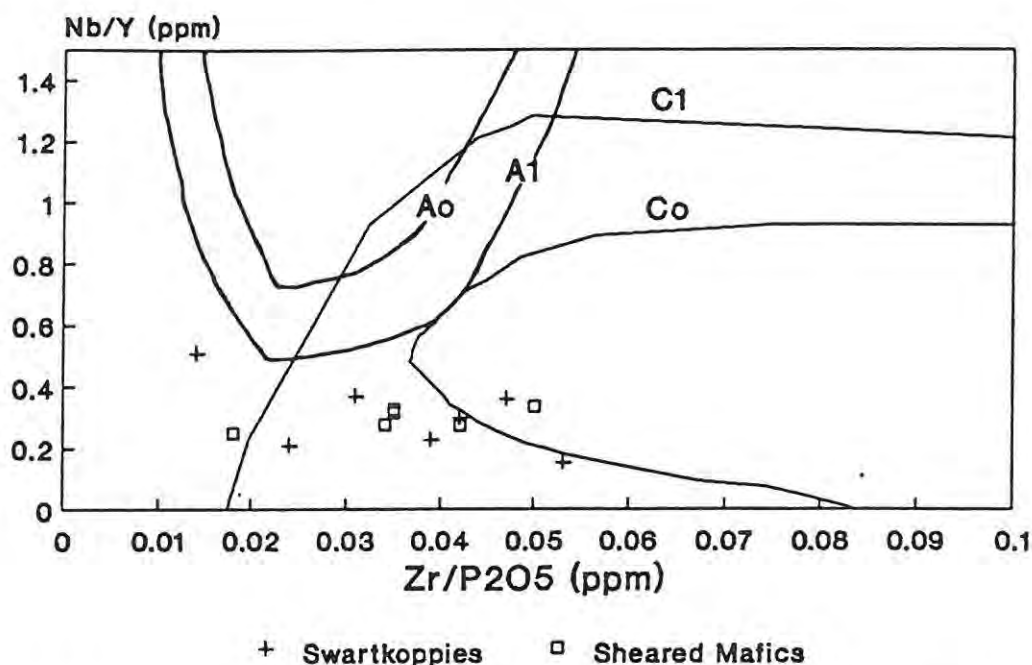
Figure 1.9.3(e): Nb/Y versus Zr/P_2O_5 discrimination diagram where oceanic alkali basalts are represented by fields enclosed by line A_0 , continental alkali basalts by A_1 , oceanic tholeiitic basalts by C_0 and continental tholeiitic basalts by C_1 (after Floyd and Winchester, 1975).
