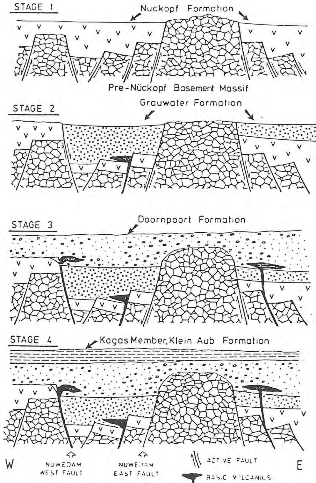
Figure 2.4(b): The tectonic, volcanic and sedimentological development of the Klein Aub basin from Nüekopf to Klein Aub times (after Borg & Maiden, 1986).
