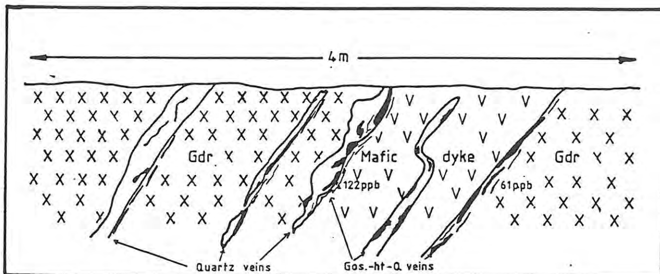
Figure 4.5.8.3: Field sketch of mineralization adjacent to a mafic dyke - Area 3.
