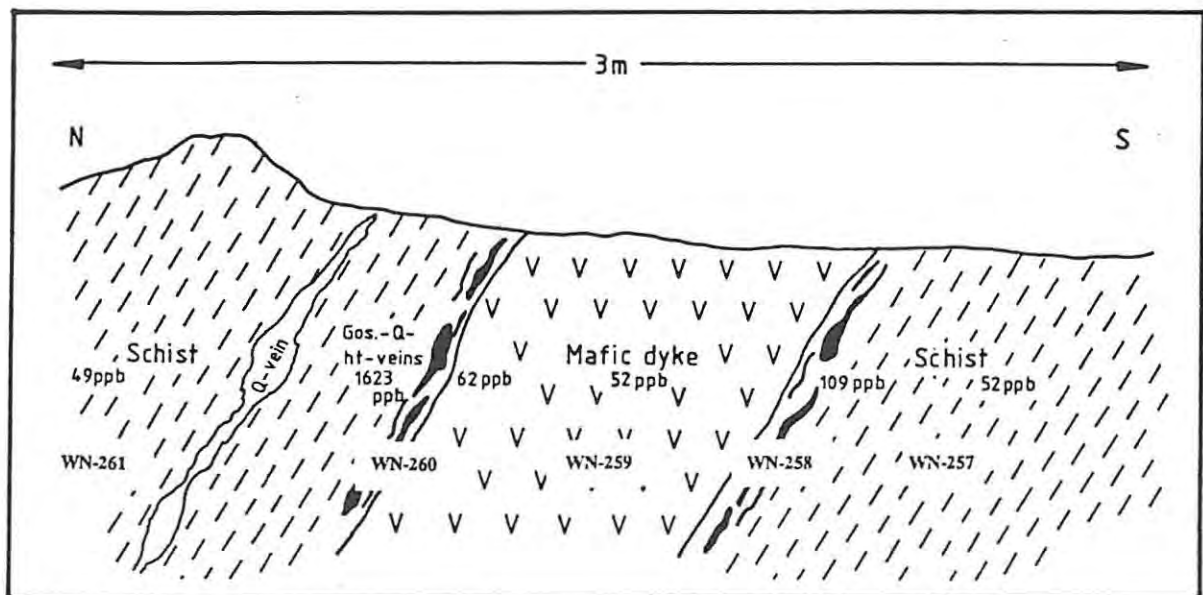
Figure 4.5.8.9(a): Field sketch and associated gold values.
