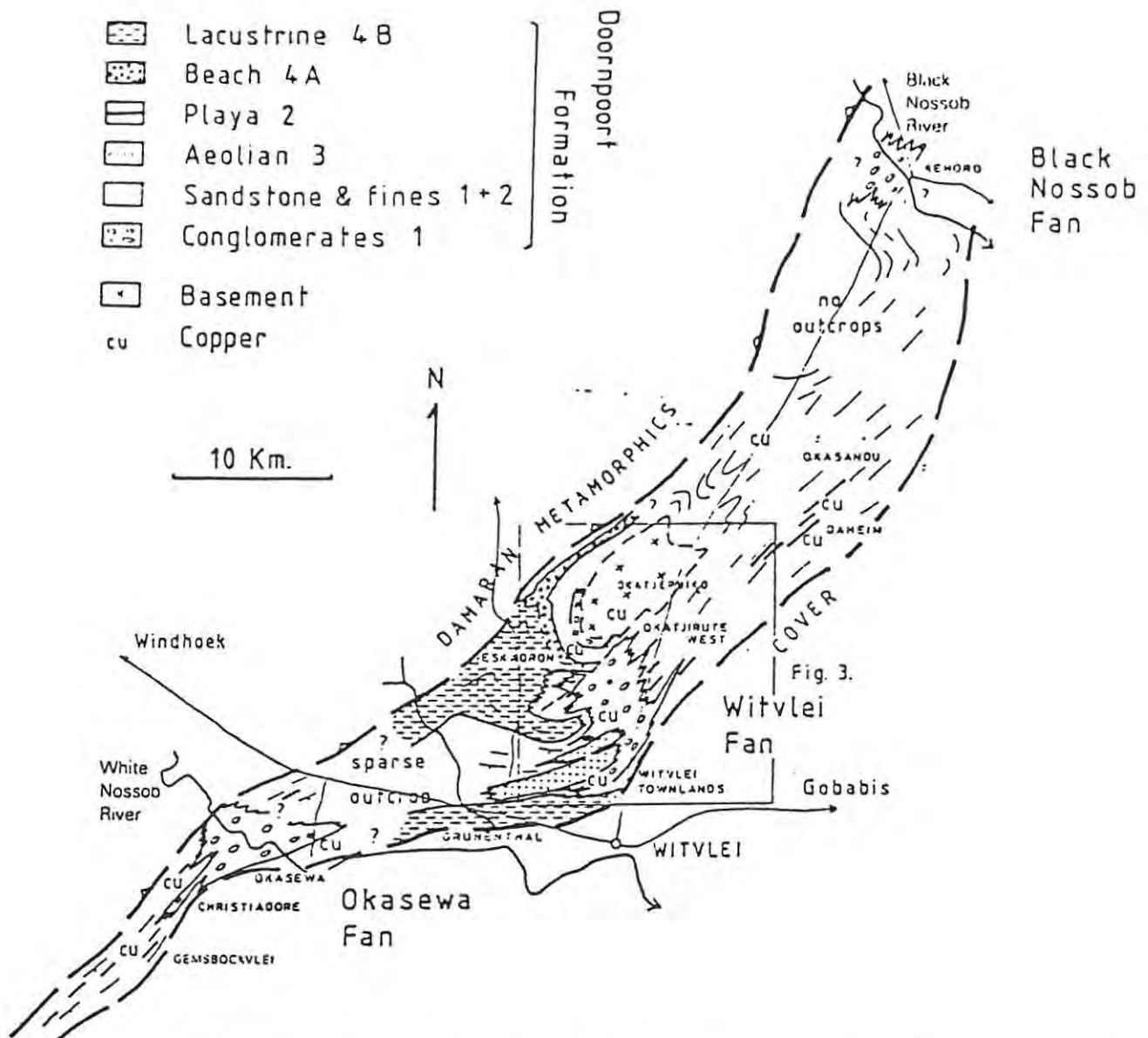
Figure 2.5(a): Sedimentary facies relations and copper distribution in the Doornpoort Formation of the Witvlei area (after Ruxton & Clemmey, 1986).
