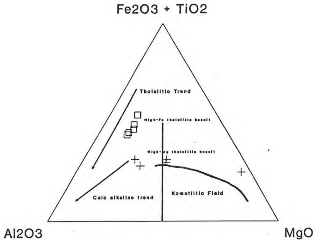
Figure 1.9.3(d): Jensen Cation Plot illustrating the tholeiitic trend in the Dordabis metabasalts (after Jensen 1976).
