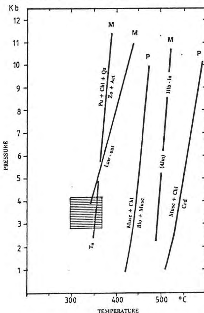
Figure 4.3.5(a): Pressure / Temperature estimates of the Neuras Grant.
