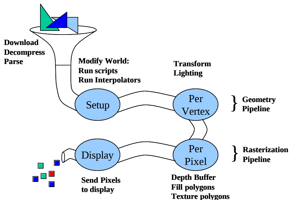
Figure B.1. VRML Rendering Pipeline [Silicon Graphics 1998]
