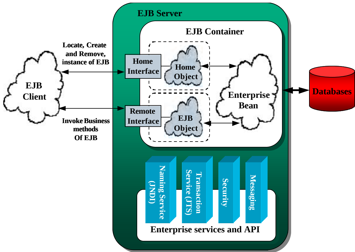
Figure 2.4. The basic EJB Model [Raj 1998]
