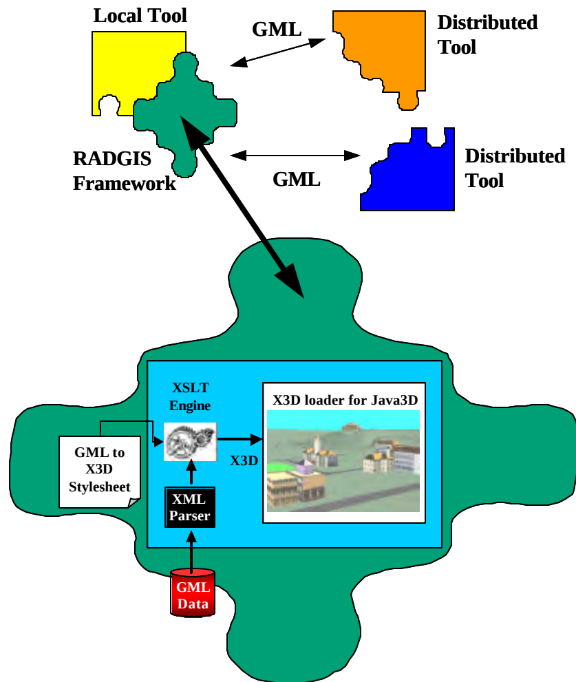
Figure 4.4. The intended use of GML in the RADGIS architecture
