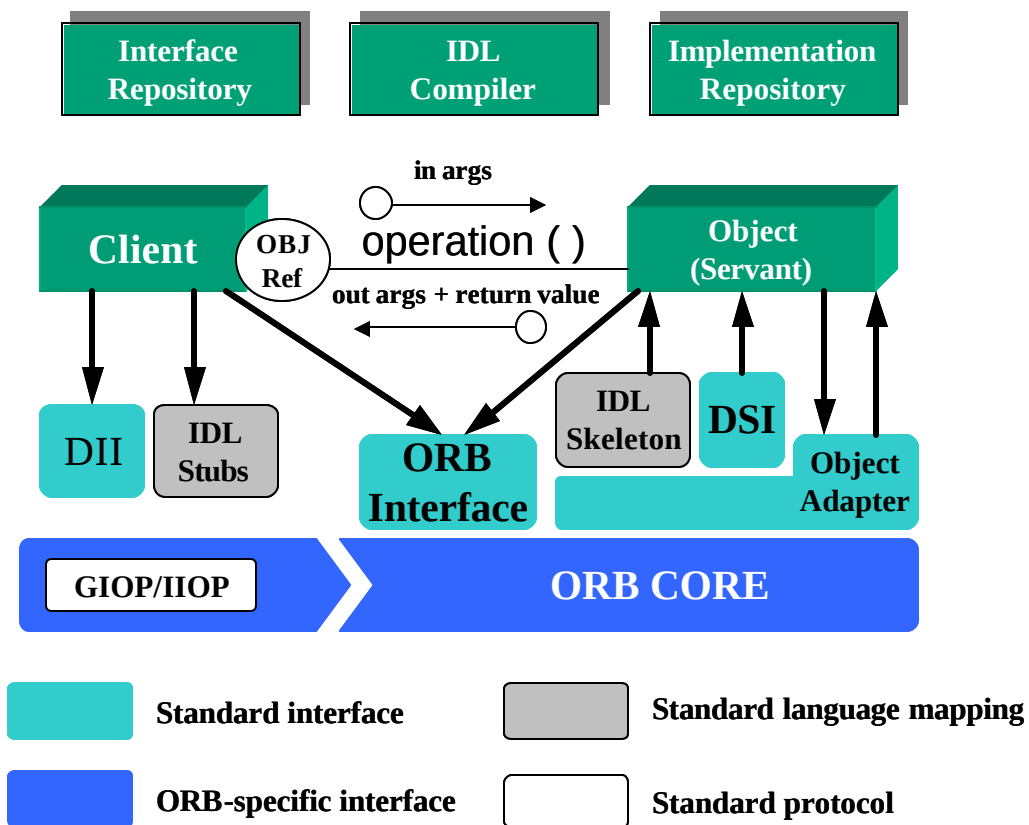
Figure 2.2. CORBA ORB Architecture [Schmidt 2001]
