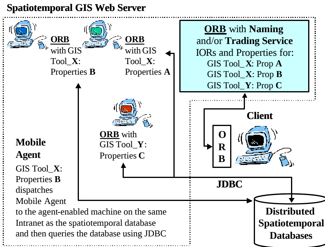
Figure A.1. Example of component interaction using a Mobile Agent
