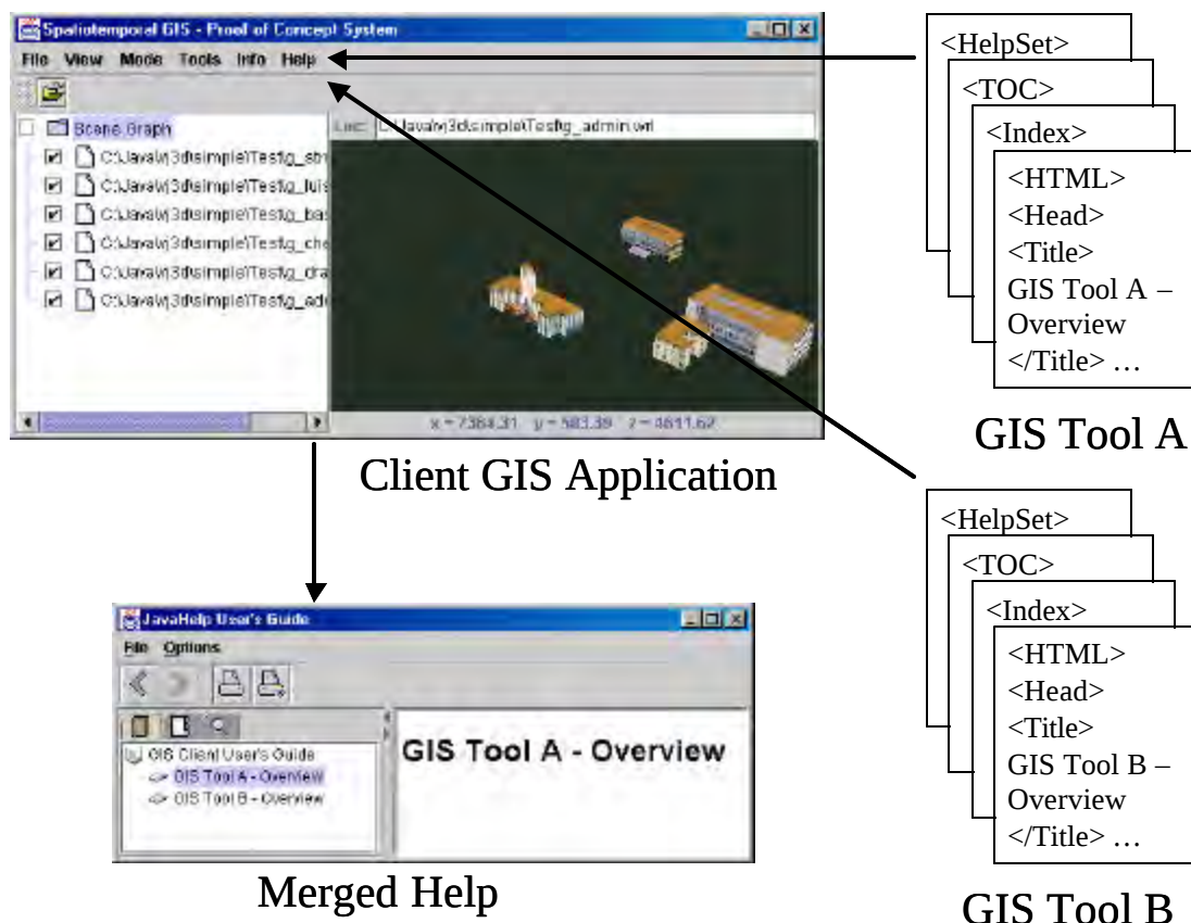
Figure 5.6. Use of JavaHelp to display help data from different GIS Services
