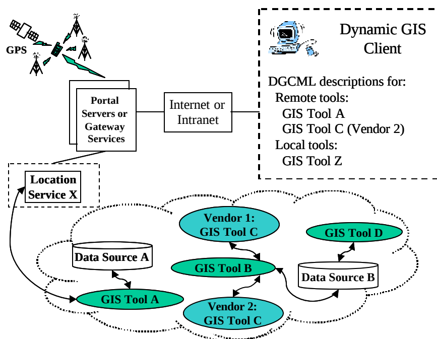
Figure 4.7. RADGIS: A highly distributed component-based GIS
