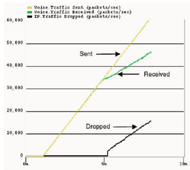
Figure 3.5: Total packets per second from simulation [64]
