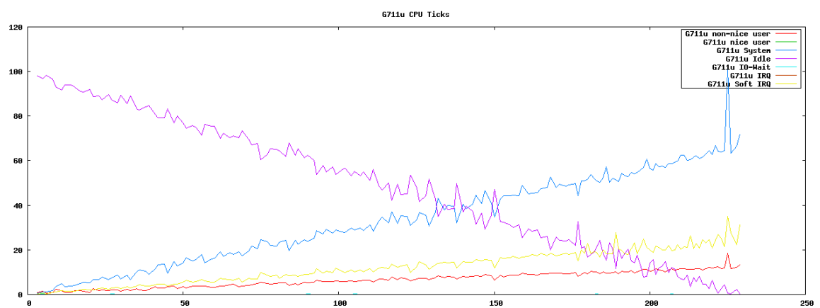
Figure 3.9: CPU usage for the DRAPA VoIP server
