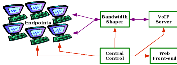
Figure 4.2: Physical layout of the DRAPA testbed.
