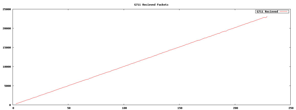
Figure 3.6: Total packets per second from DRAPA
