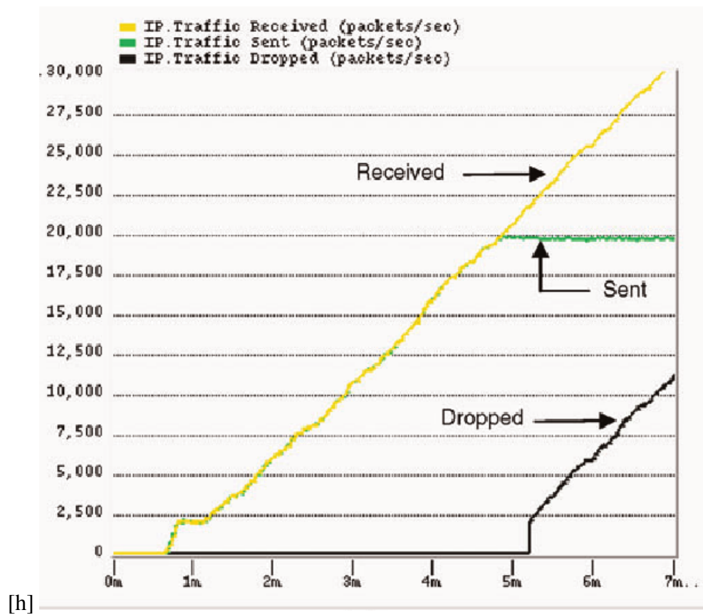
Figure 3.8: Packets per second received and sent by the router [64]
