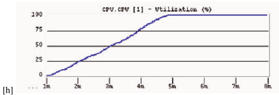
Figure 3.7: Simulation of CPU utilisation of router [64]
