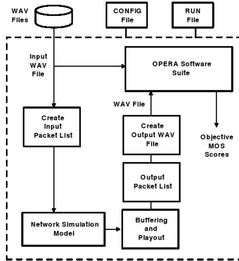
Figure 2.8: Software architecture of VoIP analysis tool by Conway & Zhu [22]
