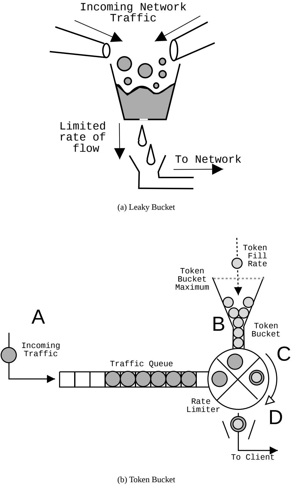
Figure 4.7: Leaky and Token bucket principals
