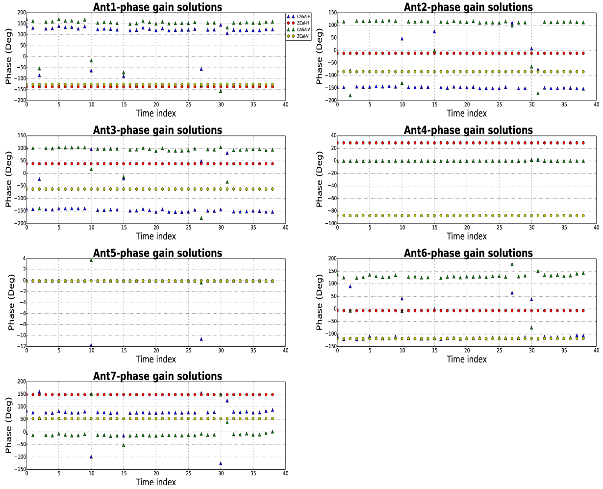
Figure 3.31: This figure shows the response of the decision tree learning algorithm in predicting the H & V phase gain solutions for the calibrator PKS1613-586 from the validation dataset-2. In each subplot we compare the predicted phase gain solutions (where H polarization is represented by red and V-polarization is represented by yellow) with the CASA generated phase gain solutions (where H polarization is represented by blue and V-polarization is represented by green). The decision tree algorithm is failing to predict the gain phase solutions for some antennas and performing well in others as seen for example in antenna 1 where CASA estimated solutions at 150^\circ and the decision tree at -150^\circ with no outliers. We also observe that it has simply learned that the reference antenna is flat.
