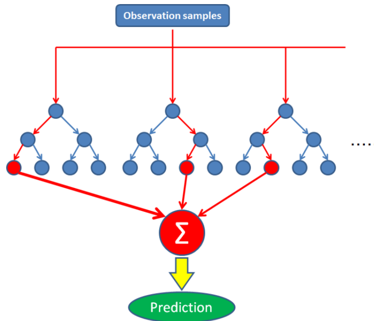
Figure 2.8: Random forest regression. [image by Data scientist TJO in Tokyo]
