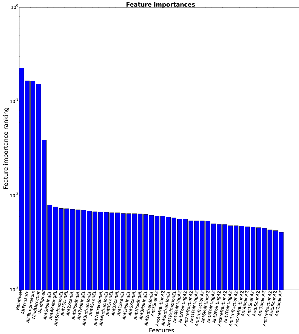
Figure 3.14: Feature importance
