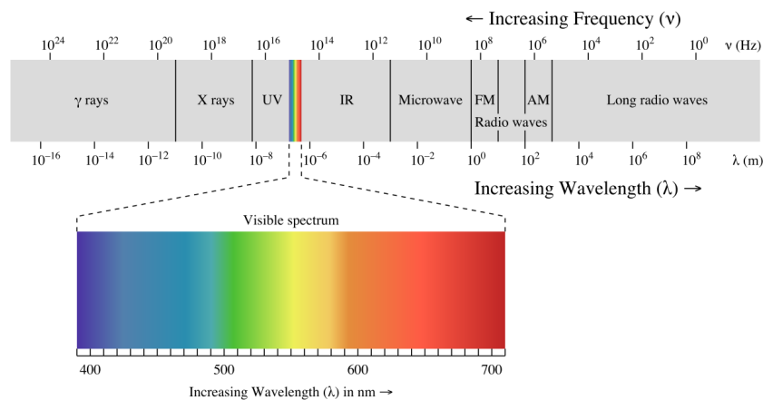
Figure 1.1: The electromagnetic spectrum (The Electromagnetic Spectrum)
