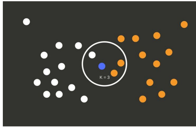
Figure 2.9: Example of K-nearest neighbor. The figure shows two different target classes orange and white circles, and one blue data point which has an unknown class. From the data points presented, we observe that the total number of the training samples with known classes is 26. To predict the unknown target class for the blue circle, one considers the K value as 3, and calculates the similarity distance using similarity measures such as Euclidean distance to find its nearest neighbours, and then computes the average value of the 3 nearest neighbors to find the unknown target's prediction (K-nearest neighbor algorithm).
