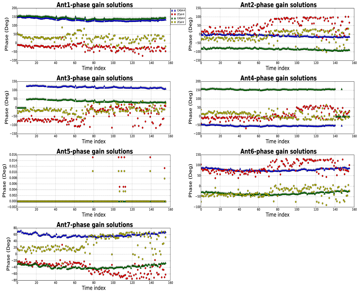
Figure 3.29: This figure shows the response of the extremely randomized tree learning algorithm in predicting the phase gain solutions for the calibrator PKS1613-586 from the validation dataset-1. In each subplot we compare the predicted phase gain solutions (where H polarization is represented by red and V-polarization is represented by yellow) with the CASA generated phase gain solutions (where H polarization is represented by blue and V-polarization is represented by green). The extremely randomized tree algorithm is failing to predict the gain phase solutions for some antennas and performing well in others with few outliers.
