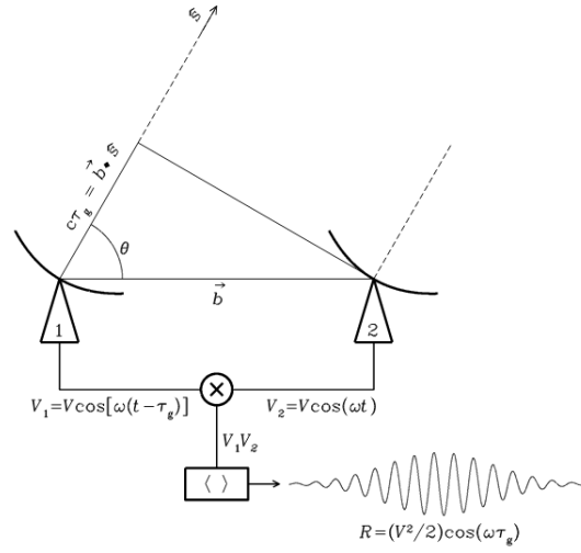
Figure 1.2: Two-antenna interferometer diagram [National Radio Astronomy Observatory]
