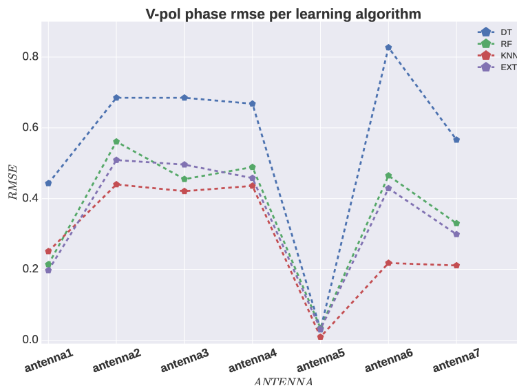
Figure 4.4: Root mean square error for each learning algorithm in predicting the V polarization phase gain solutions for each antenna. The blue, green, red and purple lines represent the different learning algorithms used in the experiment.
