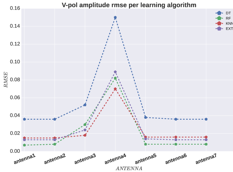
Figure 4.5: Root mean square error for each learning algorithm in predicting the V polarization amplitude gain solutions for each antenna with different colours representing different learning algorithms used in the experiment.
