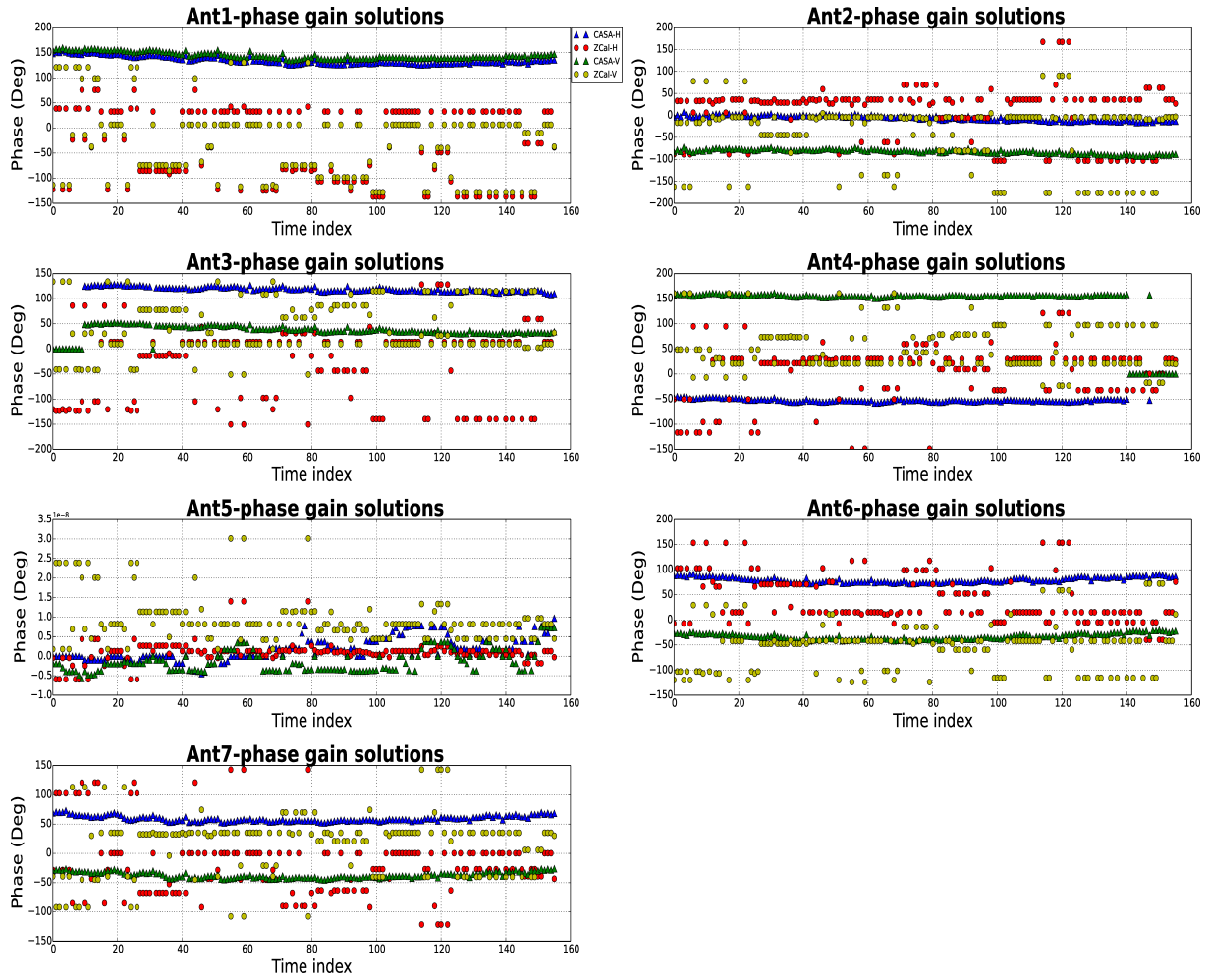
Figure 3.23: This figure shows the response of the decision tree learning algorithm in predicting the H & V phase gain solutions for the calibrator PKS1613-586 from the validation dataset-1. In each subplot we compare the predicted phase gain solutions (where H polarization is represented by red and V-polarization is represented by yellow) with the CASA generated phase gain solutions (where H polarization is represented by blue and V-polarization is represented by green). The decision tree algorithm is failing to predict the gain phase solutions on the new observation dataset-1.
