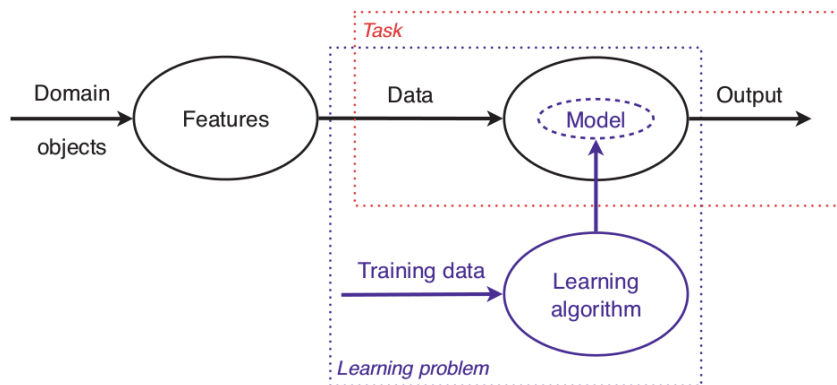
Figure 3.5: An overview of machine learning model training (Flach, 2012).
