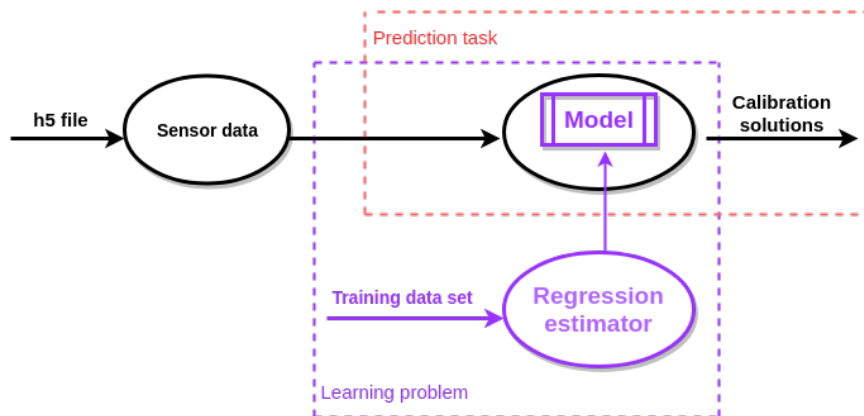
Figure 3.9: Regression learning diagram showing how we built a regression model estimator by taking in an observation file as input and extracting the sensor data per calibrator scan to obtain an accurate model that predict calibration solutions.
