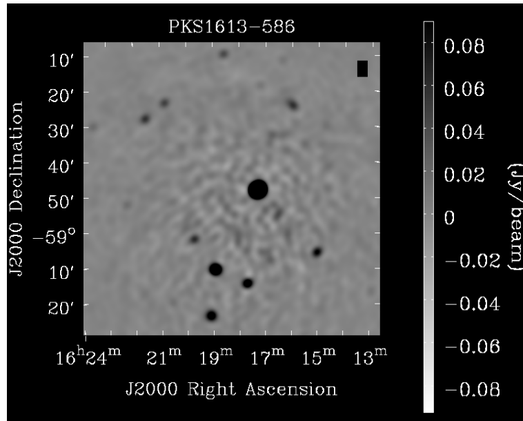
Figure 3.4: An image of the phase calibrator PKS1613-586 located at RA, Dec (J2000): 16:17:17, -58:48:07. Its flux density in Jy at frequency = 1.83GHz is 4.6 \pm 0.015 . This flux scaling was carried out in CASA using a strong flux calibrator. The expected rms noise of this image was calculated to be 0.08Jy using CLEAN task in CASA.
