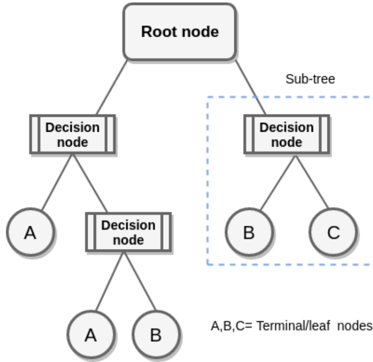
Figure 2.7: An illustration of a decision tree where a recursive partition is shown from the root node where there is an entire data sample to the internal nodes (decision nodes) where splitting occurs to form child nodes, which are either decision nodes or terminal nodes. A terminal node implies that after this split, further splitting of the samples does not provide relevant information in predicting the response variable (Moisen, 2008).
