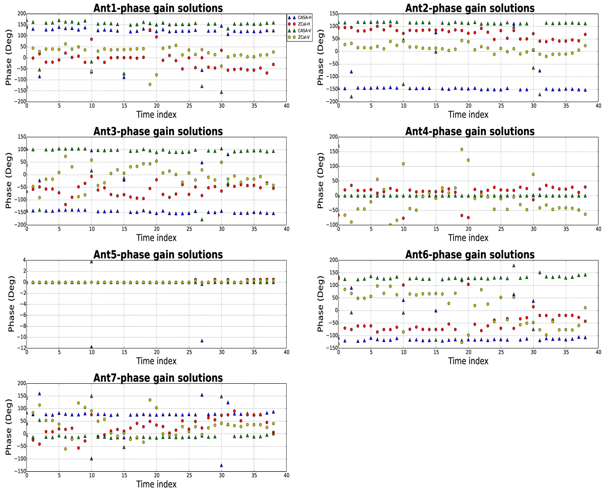
Figure 3.35: This figure shows the response of the K-nearest neighbor learning algorithm in predicting the H & V phase gain solutions for the calibrator PKS1613-586 from the validation dataset-2. In each subplot we compare the predicted phase gain solutions (where H polarization is represented by red and V-polarization is represented by yellow) with the CASA generated phase gain solutions (where H polarization is represented by blue and V-polarization is represented by green). The K-nearest neighbor algorithm is failing to predict the gain phase solutions, except for the reference antenna 5, where it learned that it is flat.
