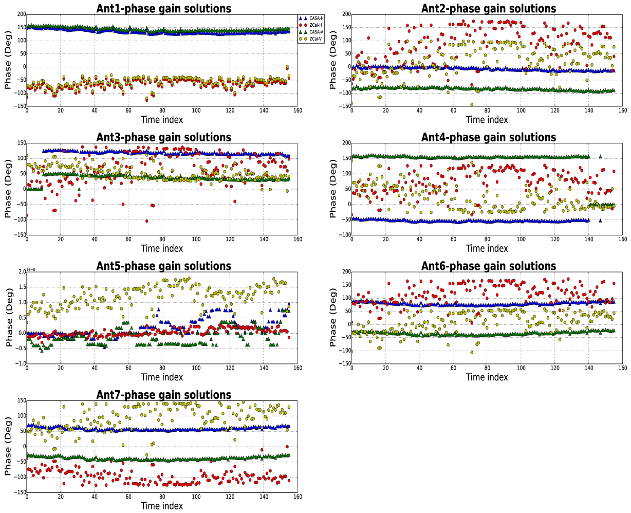
Figure 3.27: This figure shows the response of the K-nearest neighbor learning algorithm in predicting the phase gain solutions for the calibrator PKS1613-586 from the validation dataset-1. In each subplot we compare the predicted phase gain solutions (where H polarization is represented by red and V-polarization is represented by yellow) with the CASA generated phase gain solutions (where H polarization is represented by blue and V-polarization is represented by green). The K-nearest neighbor algorithm is failing to predict the gain phase solutions on the new observation dataset-1.
