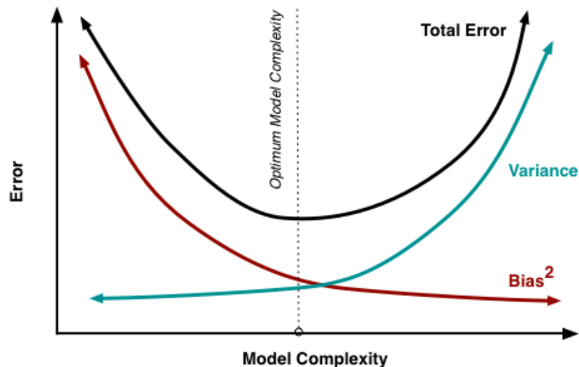
Figure 2.6: The figure is showing the bias and variance contribution to total error. Dealing with bias and variance is about dealing with overfitting and underfitting of the model. The bias is reduced and the variance is increased in relation to the model complexity. As the parameter space of the model increase, the more one experience complexity whereby the variance increases and becomes the primary concern while bias steadily decreases ( Fortmann-Roe, 2012 ).
