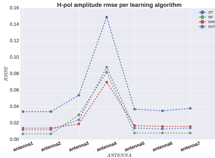
Figure 4.3: Root mean square error for each learning algorithm in predicting the H polarization amplitude gain solutions for each antenna. The blue, green, red and purple lines represent the different learning algorithms used in the experiment.
