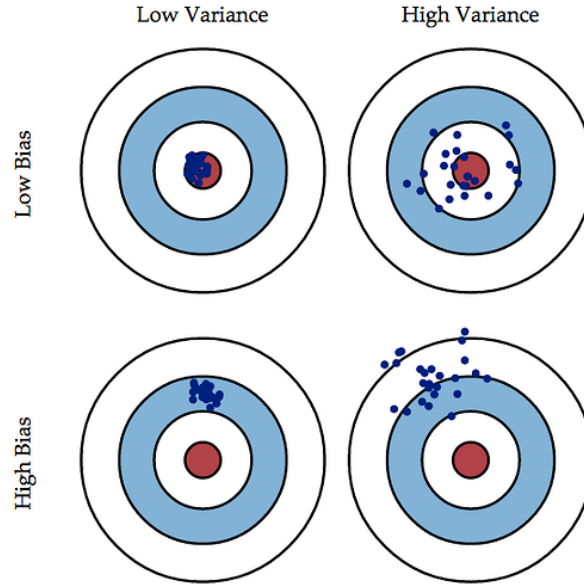
Figure 2.5: Graphical illustration of bias and variance. The center of each target represents a model that perfectly predicts the true value and as one moves away from the centre, the model gets worse at predicting the true value. Variability in the training dataset due to outliers or non-standard values will also result in poor prediction (Fortmann-Roe, 2012).
