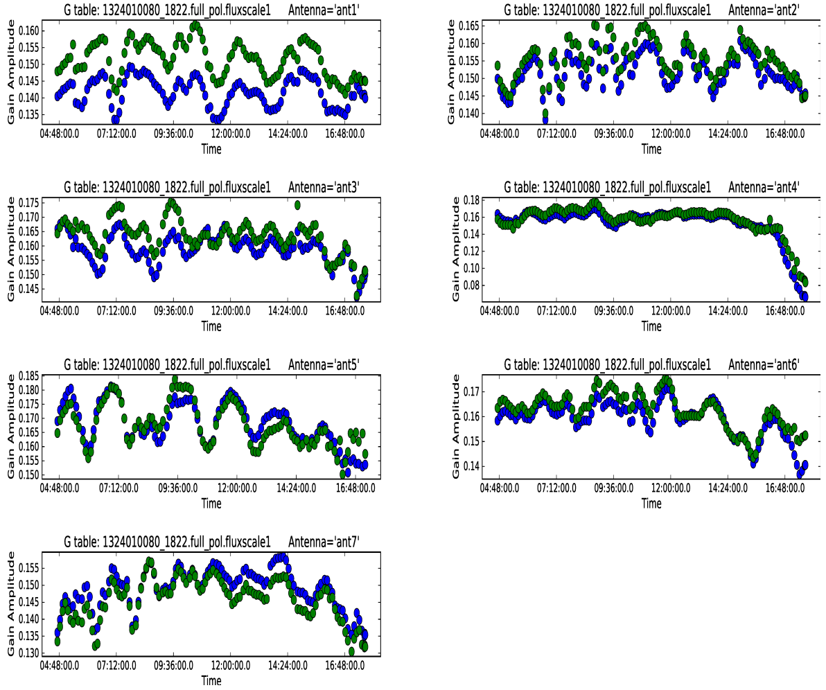
Figure 3.3: Complex gain amplitude solutions for phase calibrator PKS1613-586 obtained from CASA per antenna i . Blue is H-polarization and green is V-polarization.
