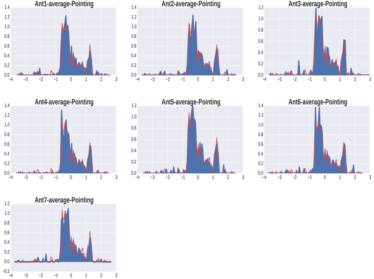
Figure 4.1: This figure shows the distribution of the averaged pointing data per antenna during the tracking of the calibrator source PKS1613-586. The blue plot represents the average of all the pointing sensors per antenna, and the red line is the reference probability distribution for all KAT-7 antennas.
