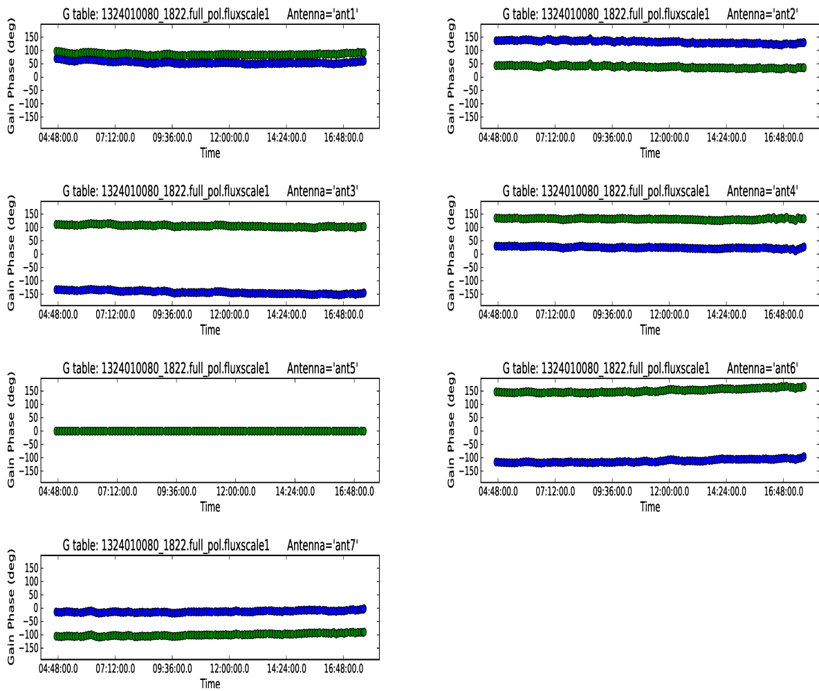
Figure 3.2: Complex gain phase solutions for phase calibrator PKS1613-586 obtained from CASA per antenna i . Blue is H-polarization and green is V-polarization. Antenna 5 shows zero phase since it is used as a reference antenna.
