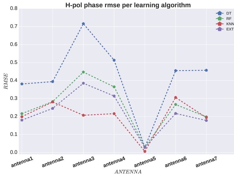
Figure 4.2: Root mean square error for each learning algorithm in predicting the h polarization phase gain solutions for each antenna. The blue, green, red and purple lines represent the different learning algorithms used in the experiment.
