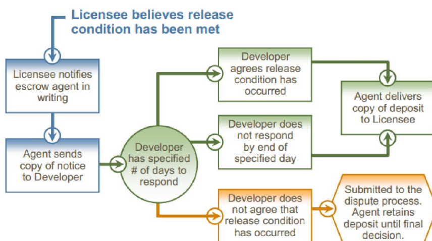
Figure 4 - Release Process Workflow (Covello & Boruvka, 2010)
