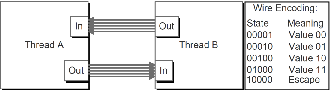
Figure 2.5: XMOS Fast Link Communication (May, 2009)
