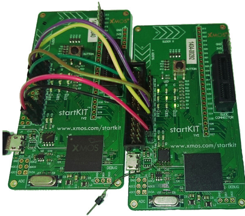
Figure 4.1: Implemented Platform for Testing XMOS Serial Link
