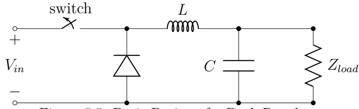
Figure 5.5: Basic Design of a Buck Regulator
