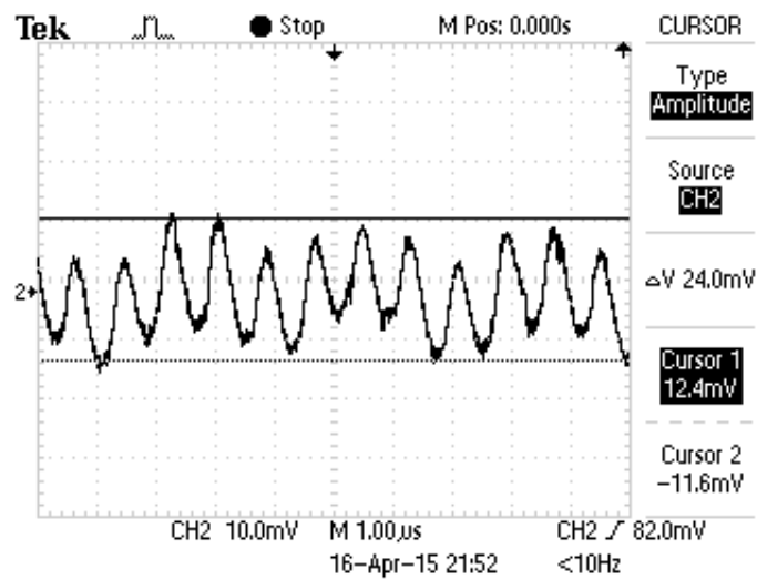
(c) Recorded V_{ripple} after low pass filter (approximately 2.4% of DC voltage)
