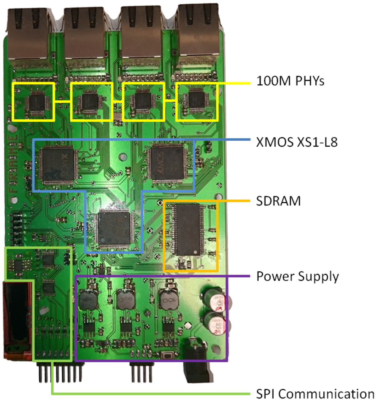
Figure 5.18: Annotated Image of the Fabricated FRAME Board
