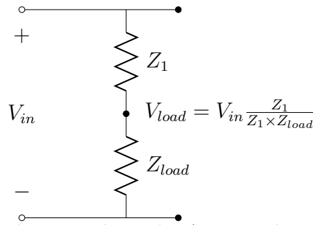
Figure 5.1: Theoretical Potential Divider Associated With a Linear Regulator
