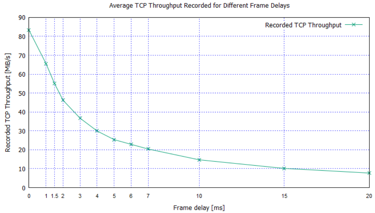
Figure 4.11: Frame Throughput For Varying Latencies
