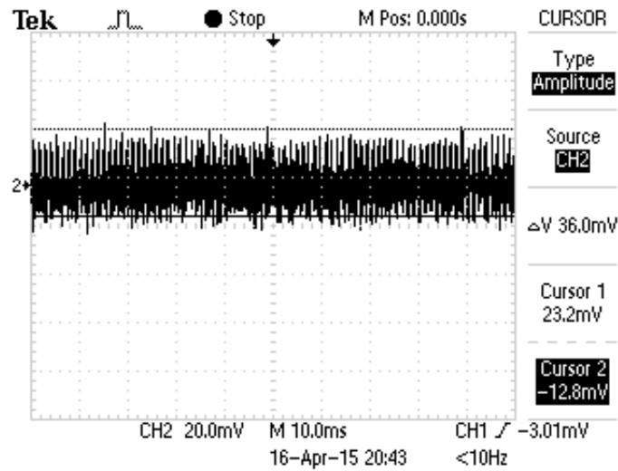
Figure 5.14: Recorded Voltage Ripple at Test Point A After Adding an Additional Capacitor
