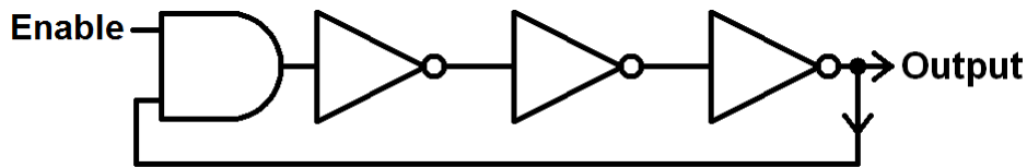
Figure 4.12: Logical Representation of a Ring Oscillator
