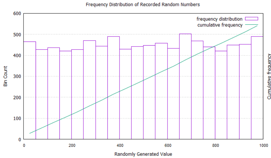
Figure 4.14: Frequency Distribution of Generated Numbers
