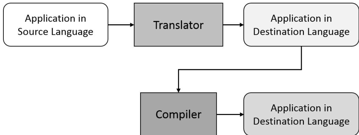
Figure 2.8: Two-Stage Compilation
