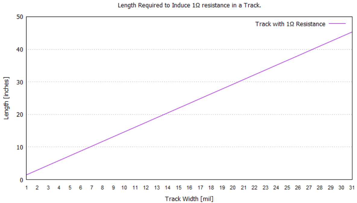
Figure 5.10: Trace Dimensions Contributing a Net Resistance of 1 Ohm
