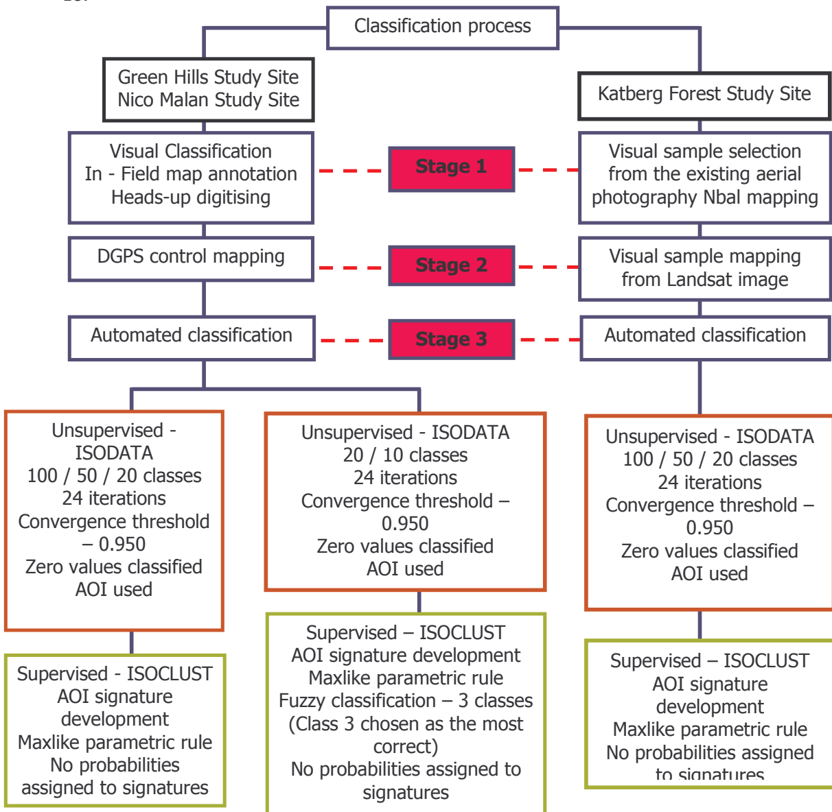
Figure 18. Classification routine summary
