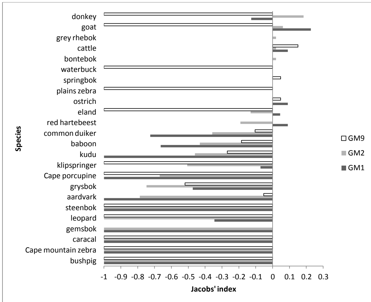
Figure 5-10. Comparison of Jacobs' index values for prey species based on kills made by each of the three collared male leopards and the relative abundance of prey within a 95% kernel home range of each leopard. The absence of a bar for a species indicates that it was not recorded within the home range of that leopard.
