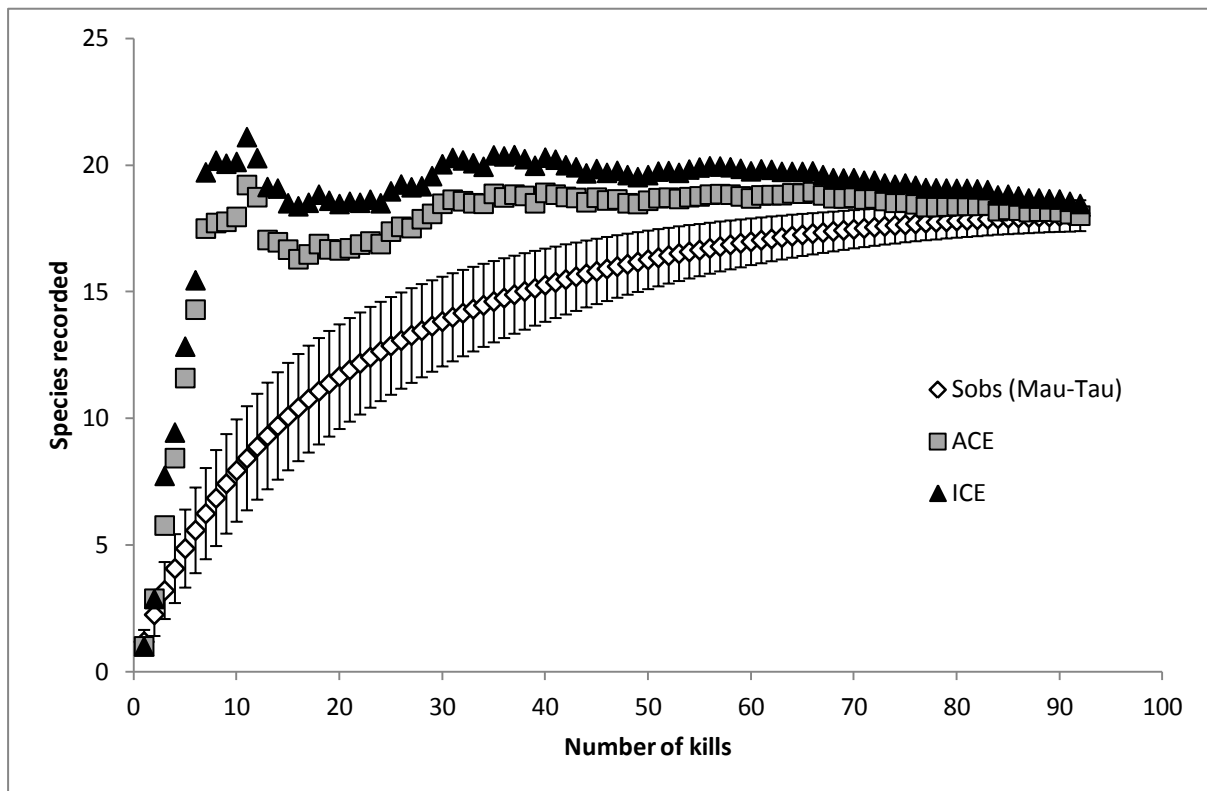
Figure 5-6. Mau-Tau species accumulation curve with 95% confidence intervals (50 randomised iterations, ACE = 18.00, ICE=18.46) for species found at leopard kill sites (n=93). ACE and ICE provide estimates of the number of species at which the curve is likely to reach an asymptote, and thus represent an estimate of the total number of species likely to be present at leopard kill sites in the area.
