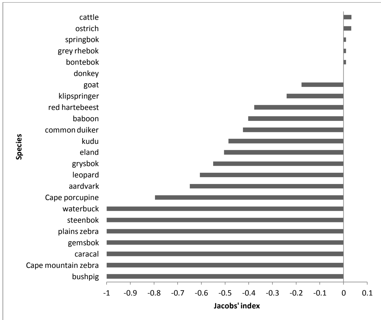
Figure 5-9. Jacobs' index scores for leopard prey based on remains found at kills made by three male leopards. Relative abundances were calculated using camera traps set within the territories of the three male leopards. Species weighing less than 9 kg were excluded from this analysis due to the difficulties of locating kills of relatively small prey species.
