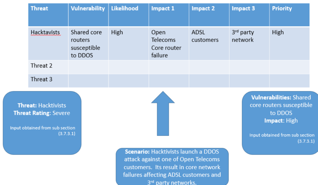
Figure 28 - Application of ENISA Risk Assessment
