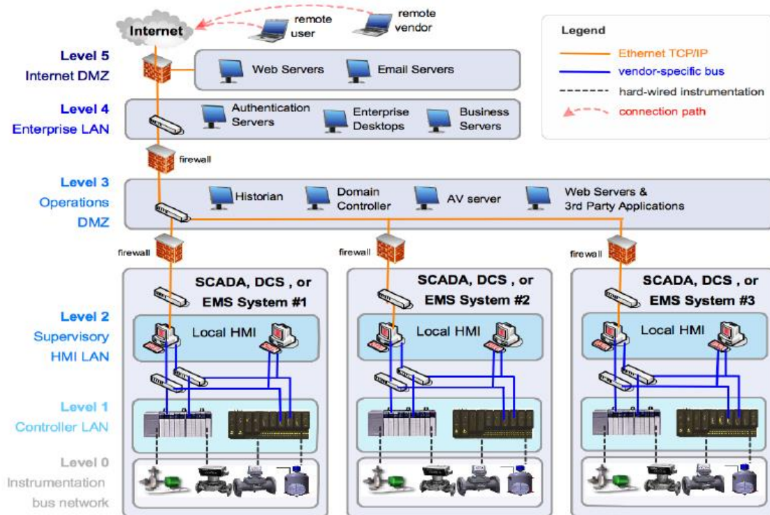
Figure 9 - ISA 99 Stacked Level Approach (Pollet, 2011)
