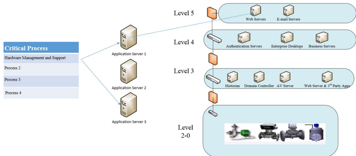
Figure 11 - Example of Process to Infrastructure Mapping
