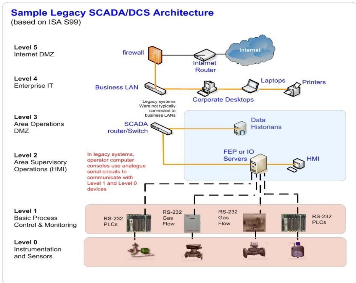
Figure 1 – Sample Legacy SCADA/DCS example (Pollet, 2011)
