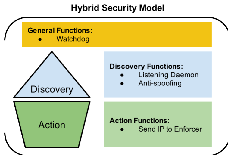
Figure 3.4: Hybrid security model components
