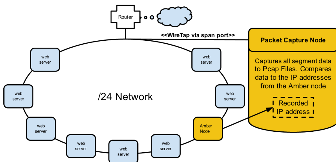
Figure 3.5: Malicious activity verified via wiretap
