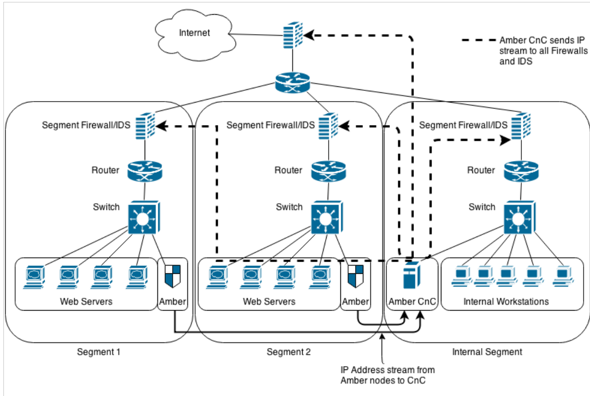
Figure 4.15: Amber architecture for a complex network with CnC server
