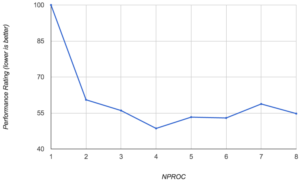
Figure 3.10: Identifying optimum NPROC setting
