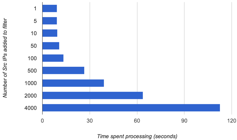
Figure 3.8: Processing time per IP (500mb pcap file)
