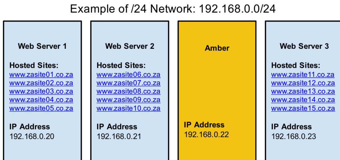
Figure 3.3: Typical Amber deployment
