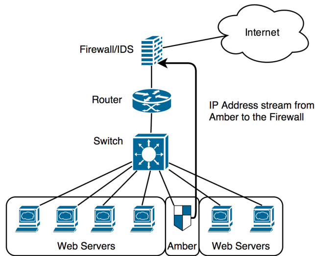
Figure 4.14: Amber architecture for a small network
