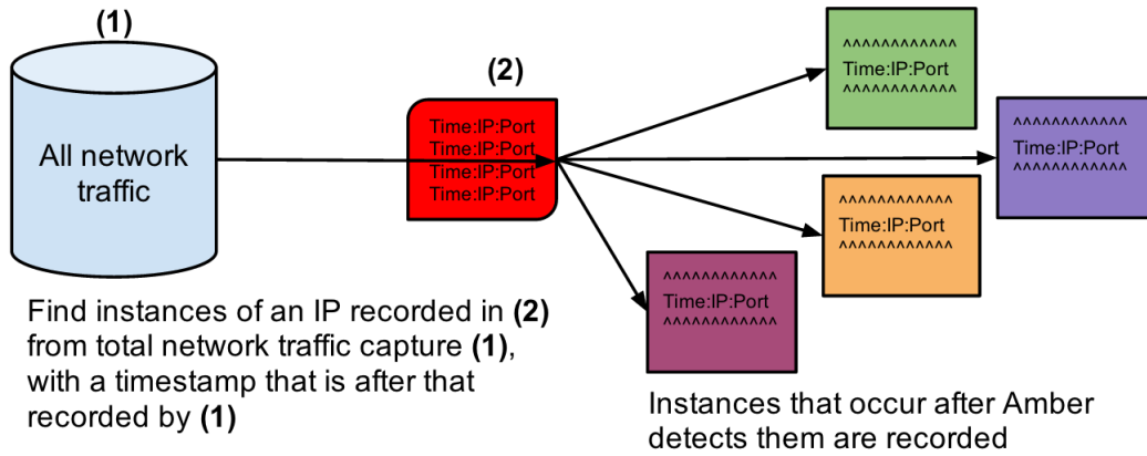
Figure 4.3: Network IP filtering according to Amber
