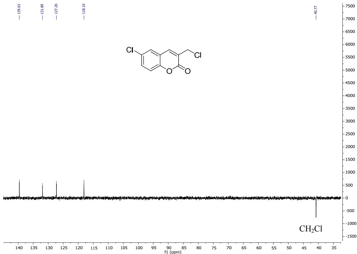
Figure 43. DEPT 135 NMR spectrum of compound 121 in CDCl 3 .
