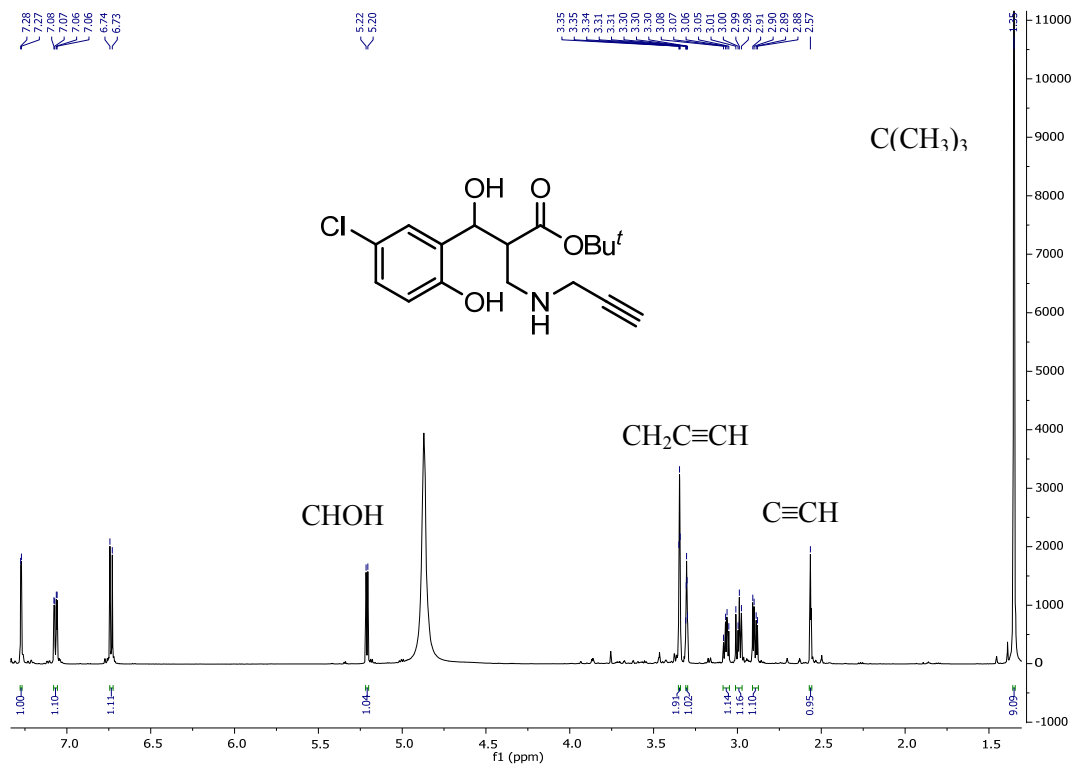
Figure 33. 600 MHz ^1\text{H} NMR spectrum of compound 114b in \text{CD}_3\text{OD} .
