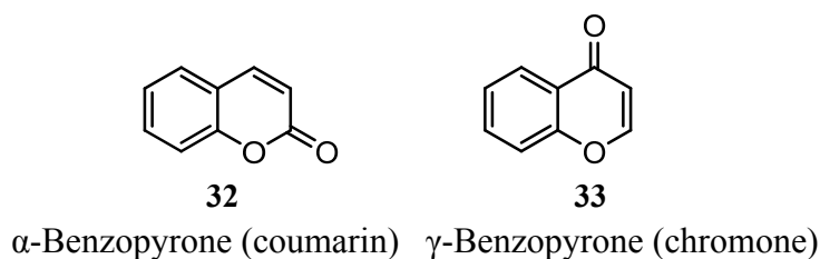
Figure 5. Chemical structures of benzopyrone subgroups. 36
