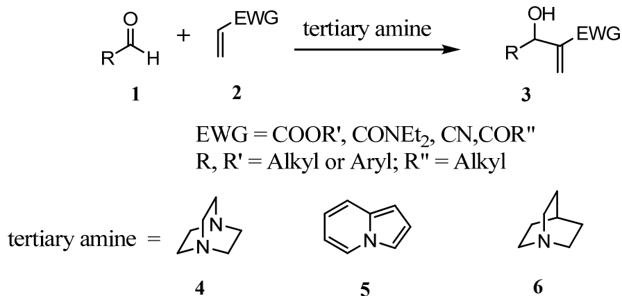
Figure 1. The Baylis-Hillman reaction, as identified in the original patent information. 5
