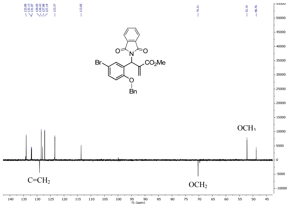
Figure 40. DEPT 135 NMR spectrum of compound 117a in \text{CDCl}_3 .
