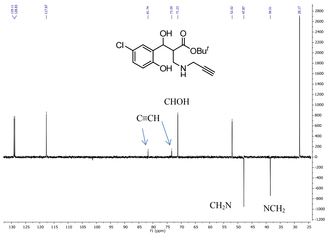
Figure 34. DEPT 135 NMR spectrum of compound 114b \text{CD}_3\text{OD} .
