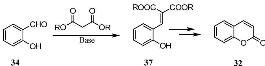
Scheme 5. The Knoevenagel reaction. 35
