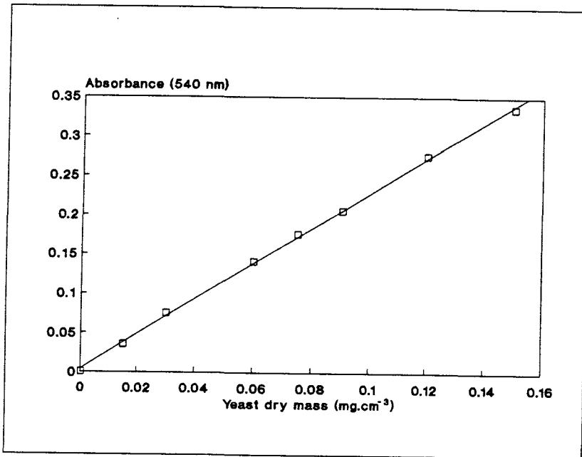
Figure 14.1: Cell concentration standard curve.
