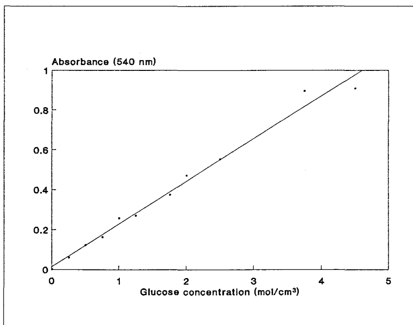
Figure 14.4: Glucose standard curve.
