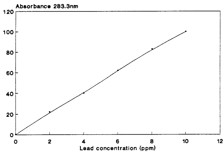
Figure 14.6: Atomic absorption standard curves for metals.
