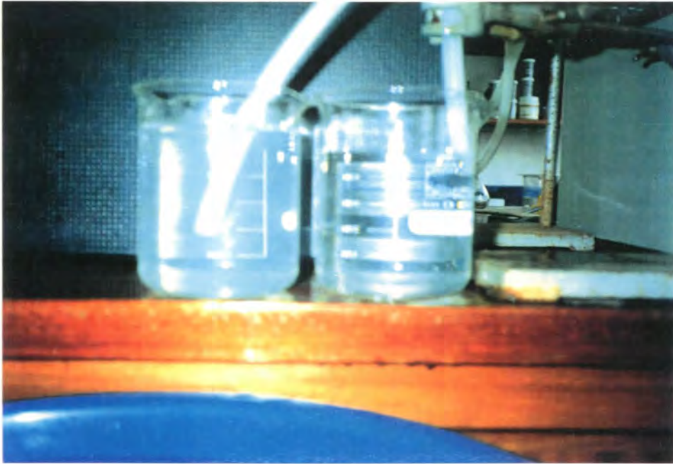
Figure 3.13: Haze removal by the yeast cell coated cross-flow microfiltration unit. The haze observed in the influent solution (left) is removed by the CFMF based bioaccumulation system to yield a clear effluent solution (right).
