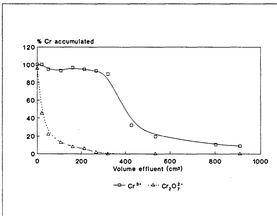
Figure 9.11: Comparison of Cr (III) (100 ppm as \text{Cr}_2(\text{SO}_4)_3 ) and dichromate (VI) (100 ppm as \text{K}_2\text{Cr}_2\text{O}_7 ) biosorption by granular biosorbent. Influent pHs were 2.6 and 4.2 respectively.
