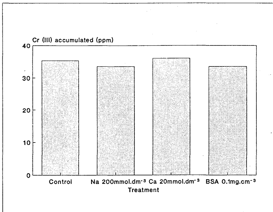
Figure 10.7: Interference of chromium biosorption by granular biosorbent by certain organic and inorganic compounds. The control was biosorption of Cr 3+ from an aqueous CrCl 3 solution.
