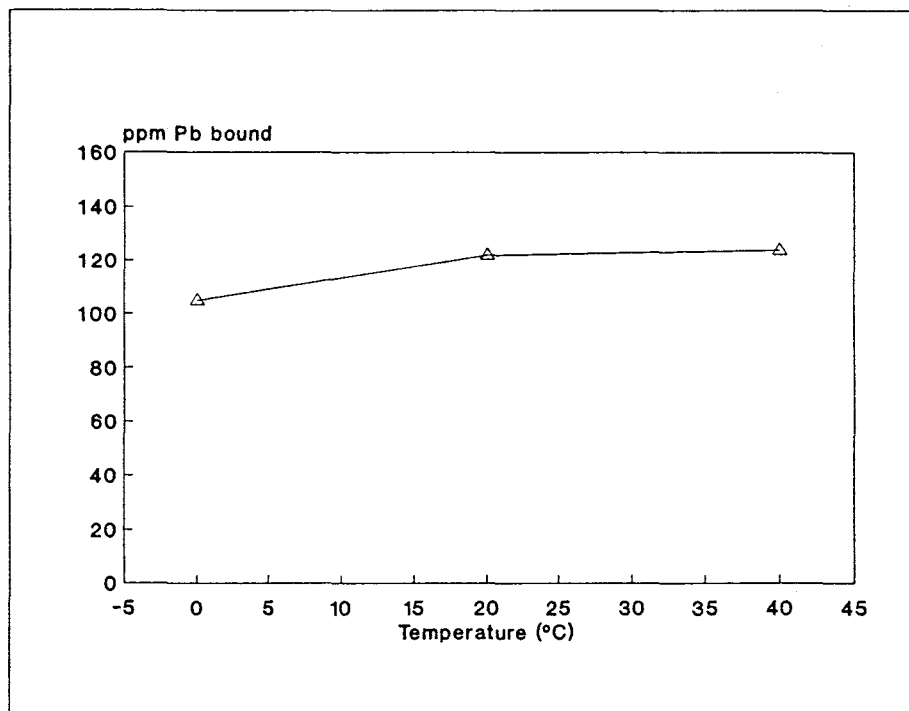
Figure 10.5: Variation of lead accumulation by granular biosorbent with temperature. Initial Pb(NO_3)_2 concentration was 200 ppm.
