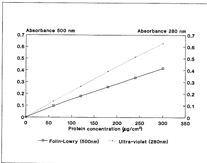
Figure 14.3: Protein standards curve, using the absorbance of aromatic amino acids at 280 nm and the Folin-Lowry method (Lowry et al, 1951).
