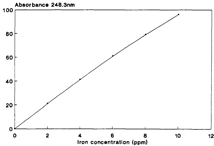
Figure 14.5: Atomic absorption standard curves for metals.
