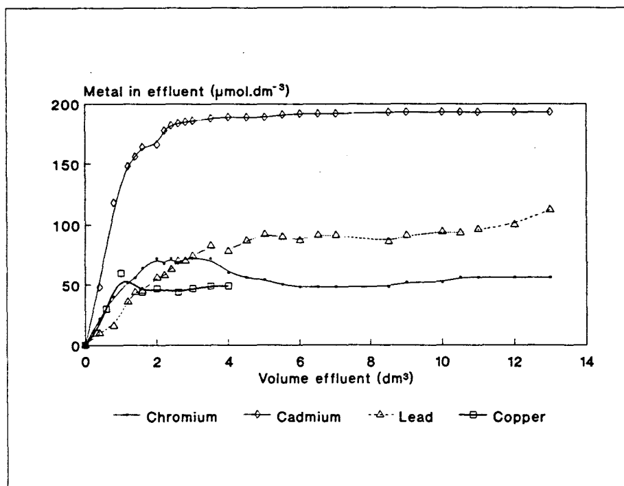
Figure 3.12: Bioaccumulation of metal cations from domestic tapwater artificially contaminated by metal chloride salts. \text{Cu}^{2+} accumulation was only monitored for the first 4 \text{ dm}^3 .
