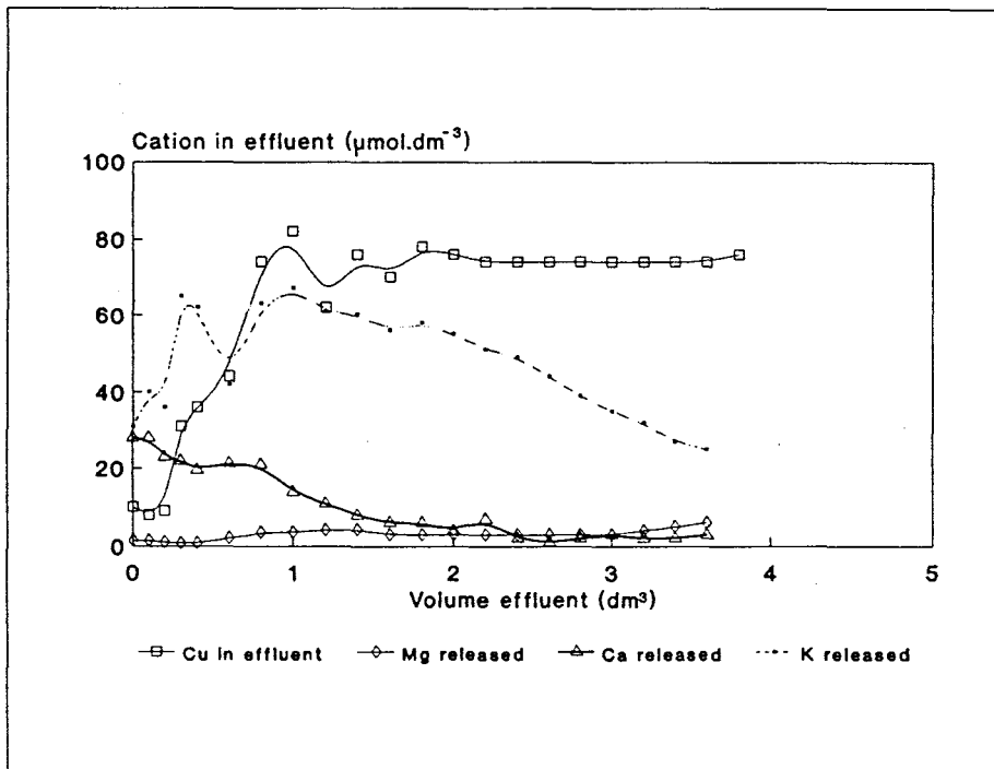
Figure 3.10: Sequential packing of the hollow fibre cartridge with yeast, followed by bioaccumulation. Temperature: 30^\circ\text{C} , flux rate: 12.5 \times 10^2 \text{ dm}^3\cdot\text{m}^2\cdot\text{hr}^{-1} .
