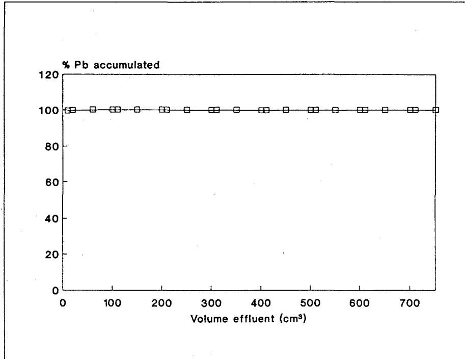
Figure 10.4: Lead accumulation from tapwater artificially contaminated by Pb(NO_3)_2 (100 ppm) by a column of granular biosorbent.
