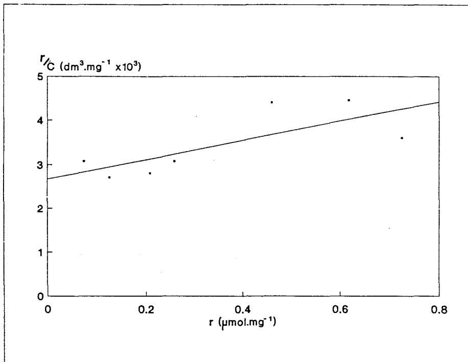
Figure 2.7: Scatchard plot of the bioaccumulation of copper by yeast cell suspensions. This figure was derived from the results presented in table 2.1 and figure 2.6.
