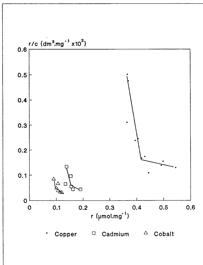
Figure 6.8: Scatchard plot of metal cation binding by the cell wall of S. cerevisiae . ( r ) is \mu moles of metal bound per mg cell wall, ( c ) is the concentration of unbound metal.
