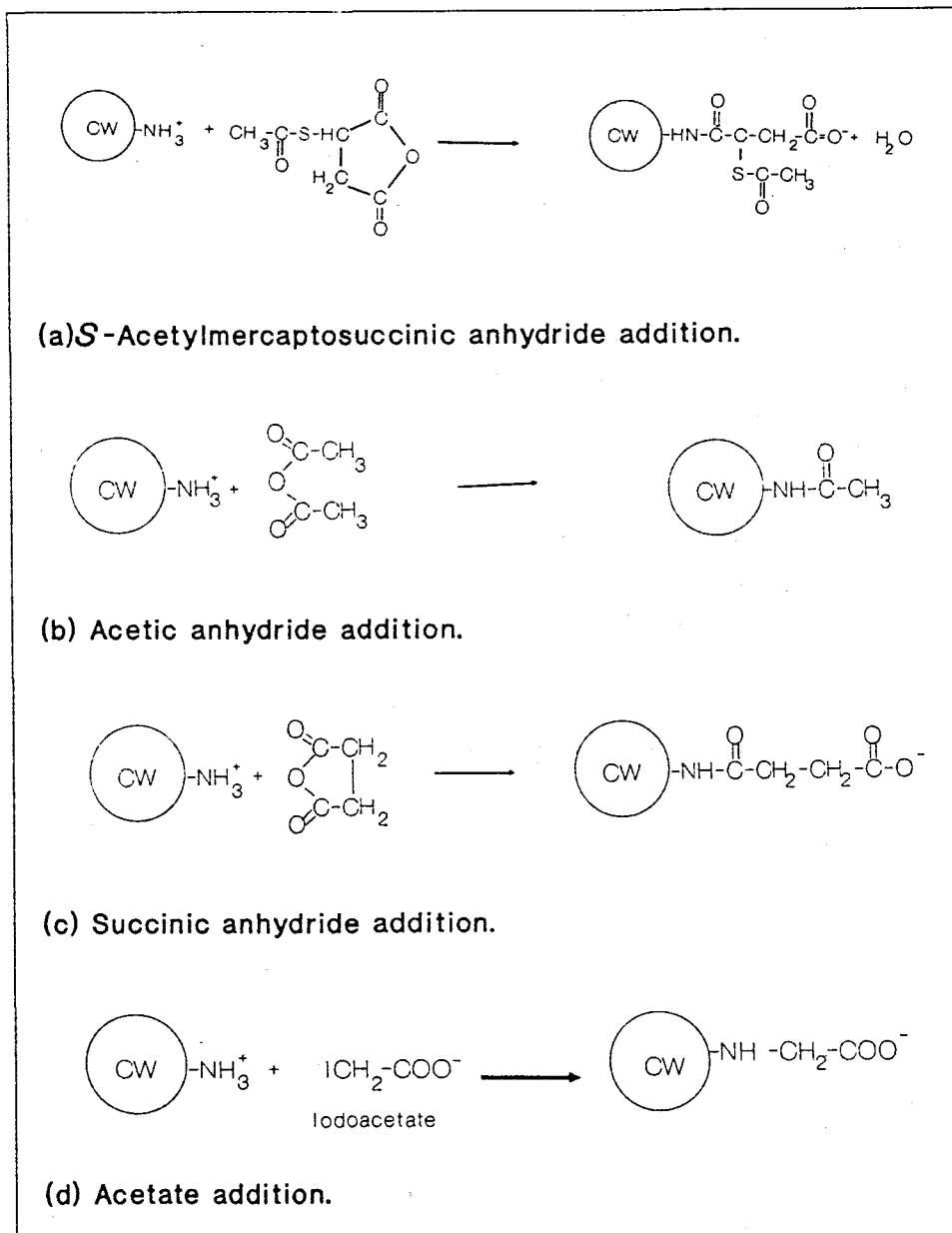
Figure 6.9: Chemical modifications of amino groups.
