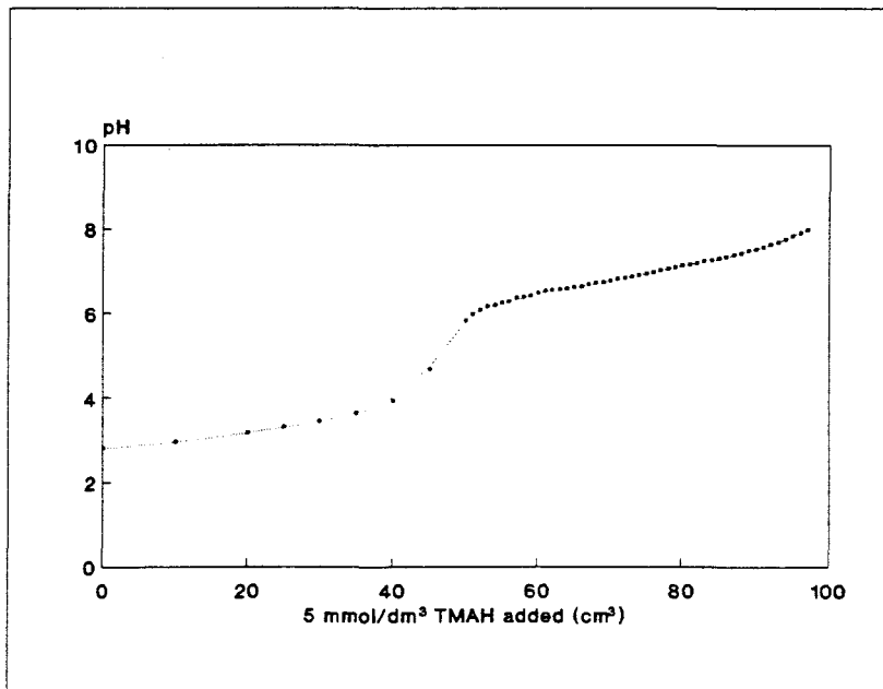
Figure 14.2: Titration curve of 5 mmol.dm -3 tetramethylammonium hydroxide against 50 cm 3 of 5 mmol.dm -3 PIPES buffer.
