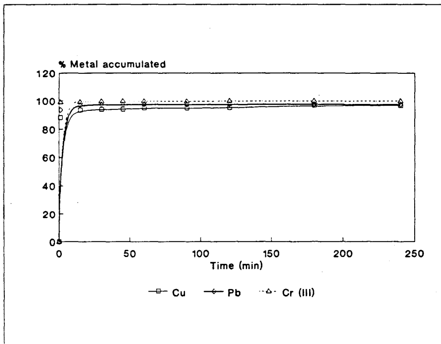
Figure 12.1: Rate of metal accumulation by Scenedesmus .
