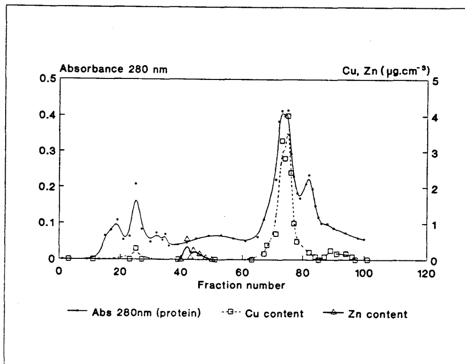
Figure 8.2: Sephadex G-75 chromatography profile of intracellular copper chelating molecules extracted from copper tolerant yeast cells. Buffer: 20 \text{ mmol}\cdot\text{dm}^{-3} Tris/ 5 \text{ mmol}\cdot\text{dm}^{-3} 2-mercaptoethanol. Column height: 75 cm, volume: 340 \text{ cm}^3 . Temperature: 20^\circ\text{C} . Flow rate: 0.4 \text{ cm}^3\cdot\text{min}^{-1} . Fraction volume: 4 \text{ cm}^3 .
