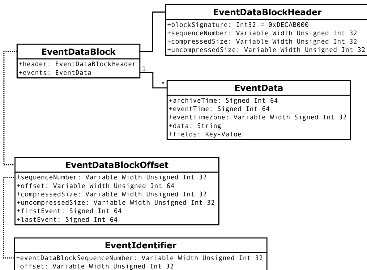
Figure 3.5: Event data block structure
