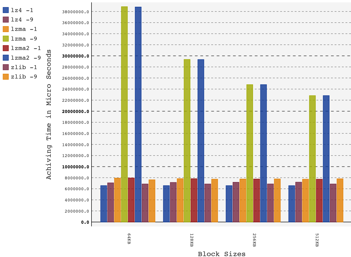
Figure 5.6: Average times for archiving sample logs
