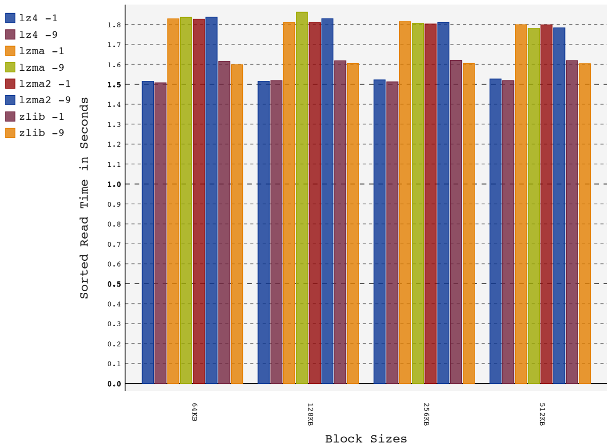
Figure 5.9: Average retrieval time based on sorted entry identifiers
