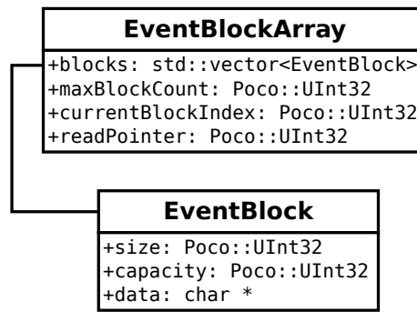
Figure 5.1: Event block array structures
