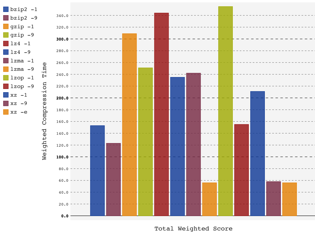
Figure 4.2: Total weighted compression times
