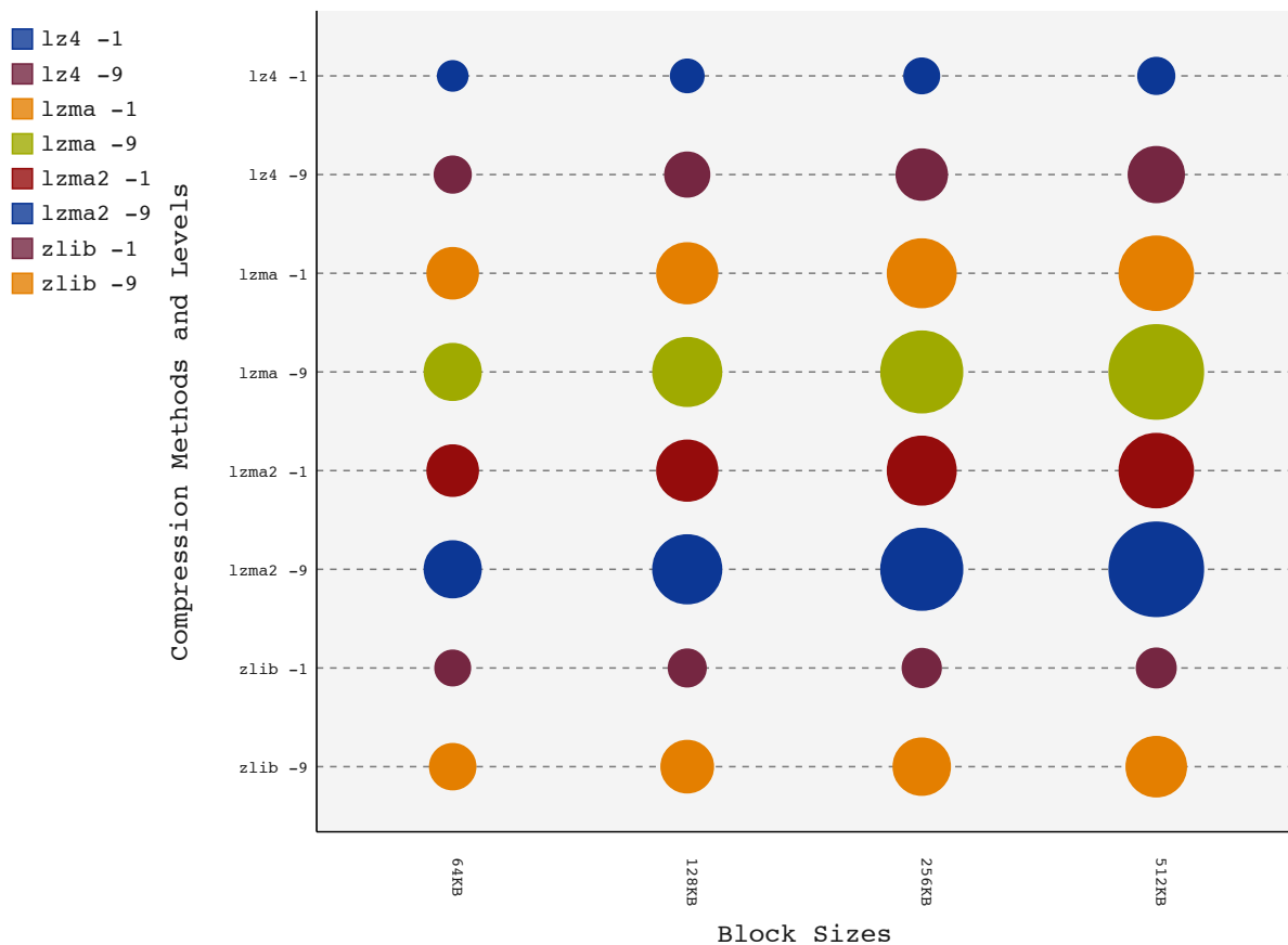
Figure 5.4: Average compression ratios in archive
