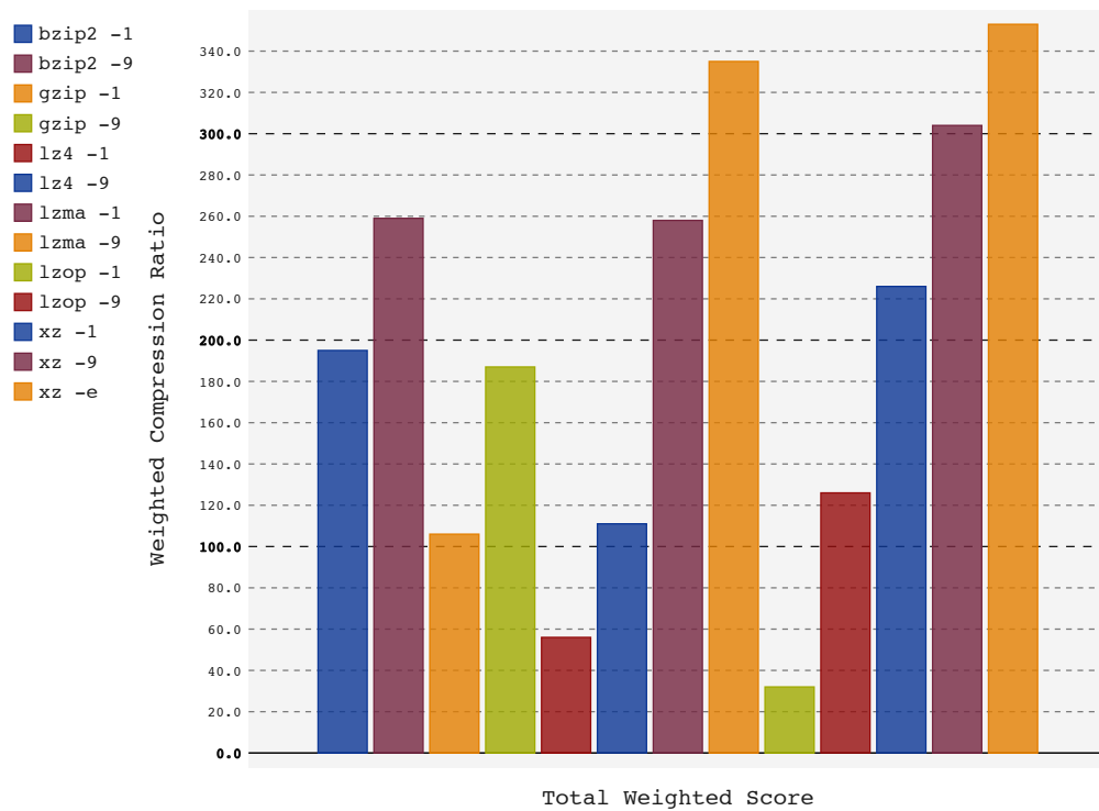
Figure 4.1: Total weighted compression ratios
