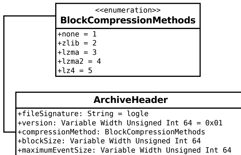
Figure 3.4: Archive header fields
