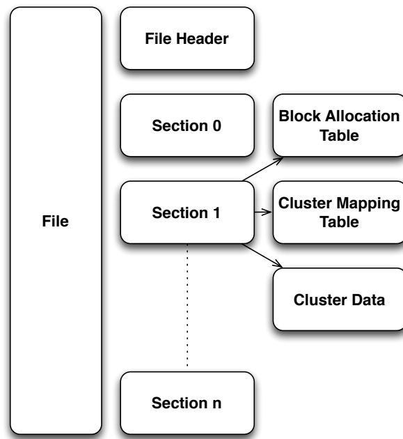
Figure 2.1: File structure of York's compressed random access file.
