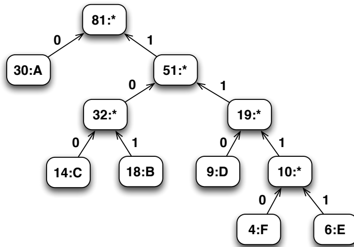
Figure 2.2: Example Huffman binary tree
