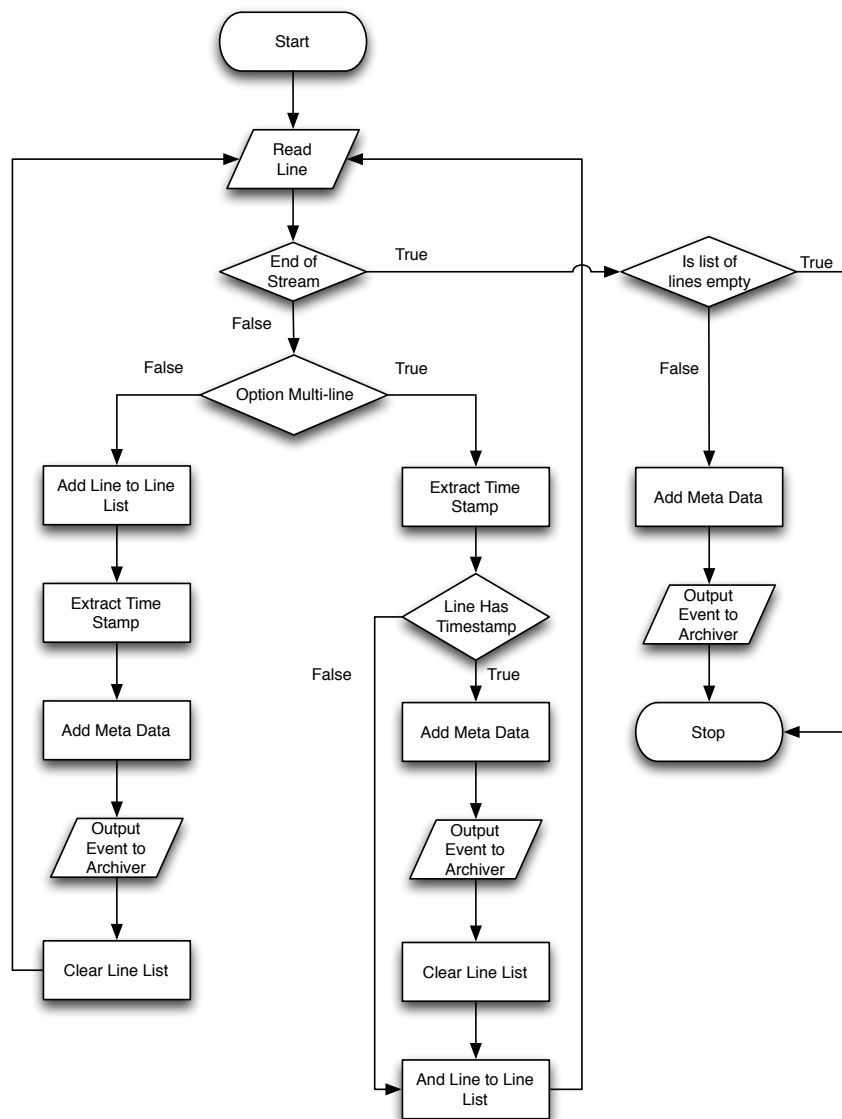
Figure 3.2: Event breaking process flow
