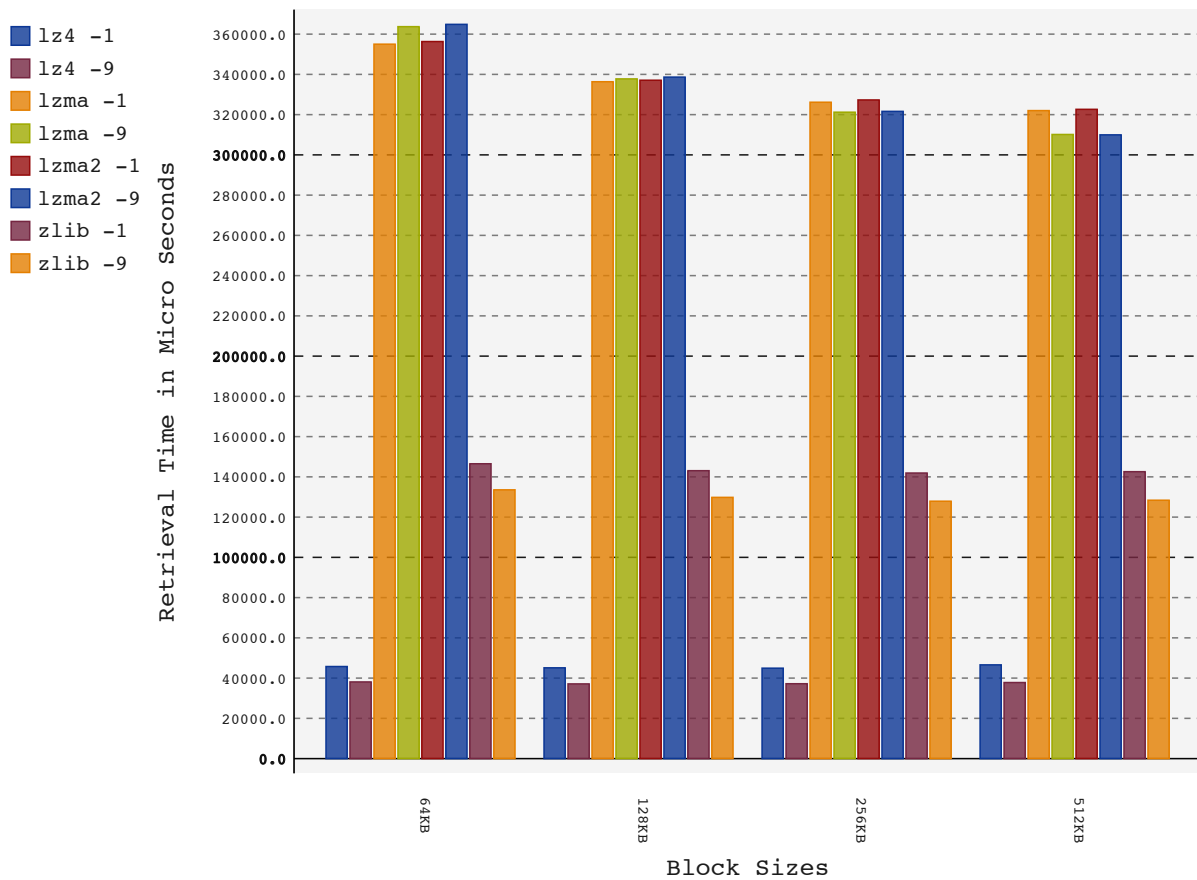
Figure 5.8: Average block retrieval times
