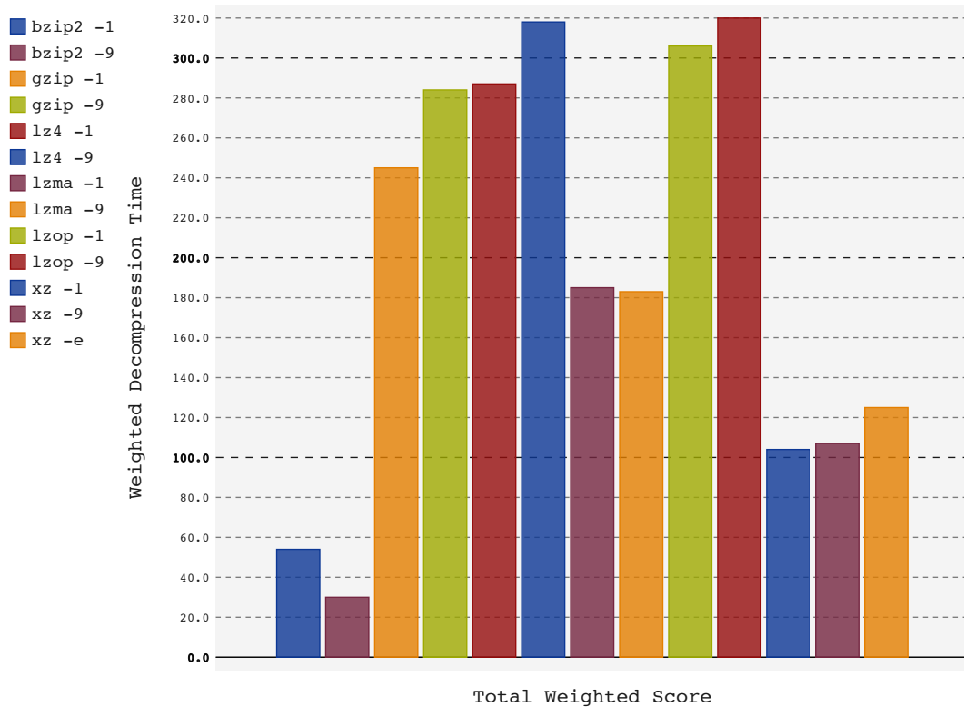
Figure 4.3: Total weighted decompression times
