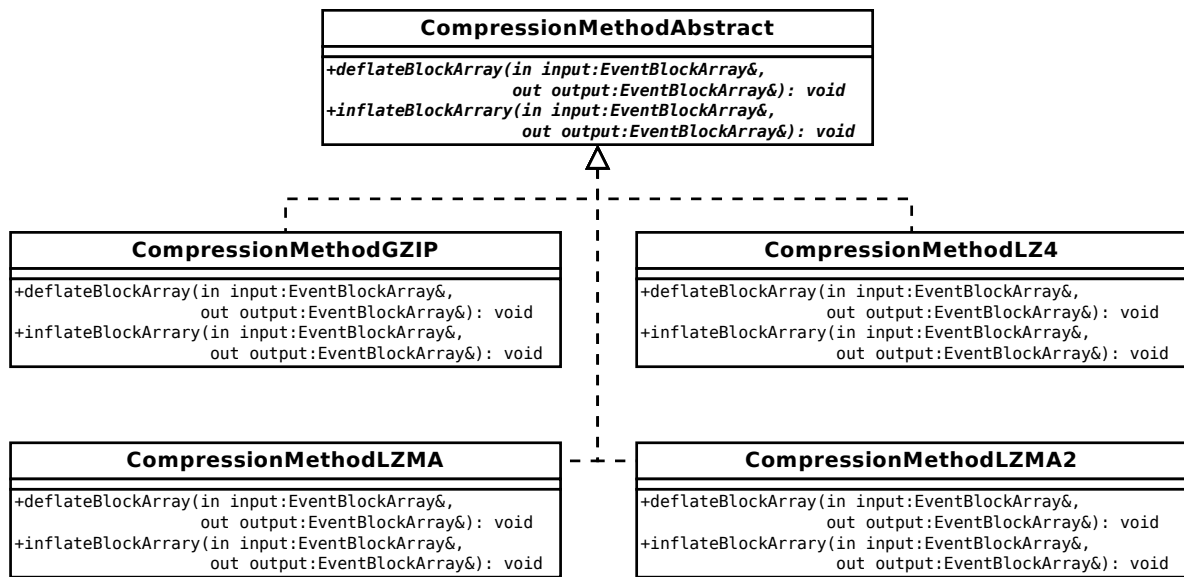
Figure 5.2: Abstract compression method design
