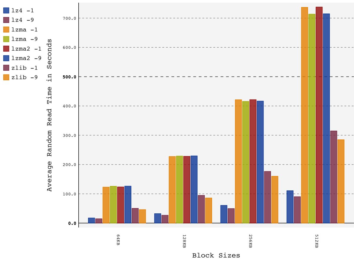
Figure 5.10: Average retrieval time based on randomly ordered entry identifiers
