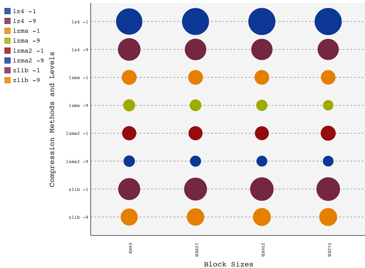
Figure 5.5: Weighted times for archiving sample logs
