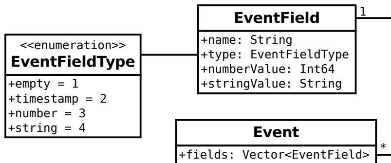
Figure 3.1: Structure of an event
