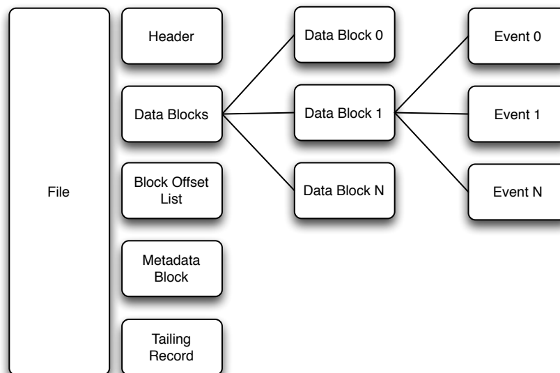
Figure 3.3: Pseudo-random access compressed file format
