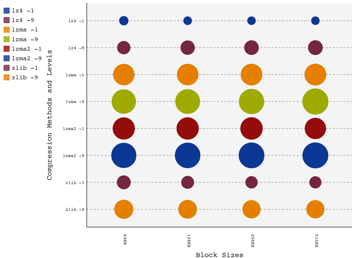
Figure 5.3: Weighted compression ratio in archive
