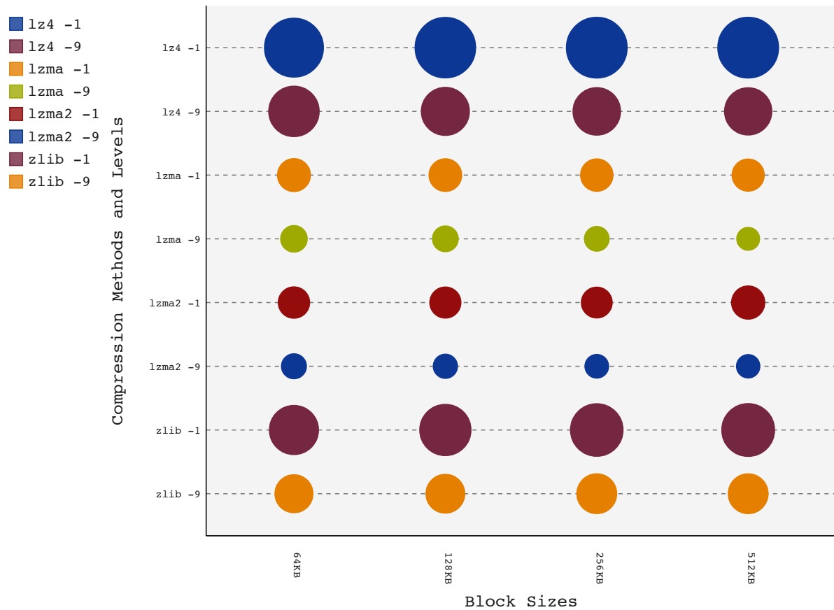
Figure 5.7: Weighted times for reading blocks from archives
