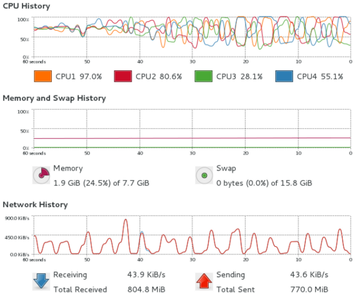
Figure 4.3: System Monitor at Simulation Runtime using Round Robin Scheduler
