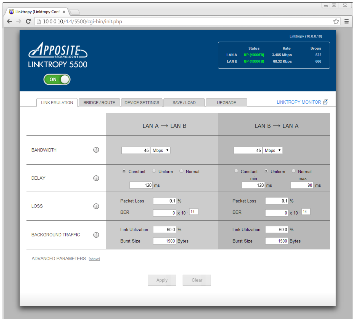
Figure 2.6: Linktropy 5500 by Apposite Technologies Web Based GUI 13
