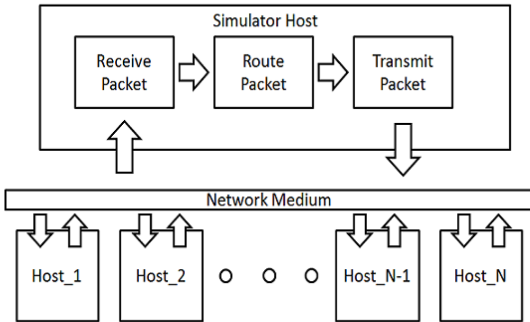
Figure 3.5: Overview of Packet Handling
