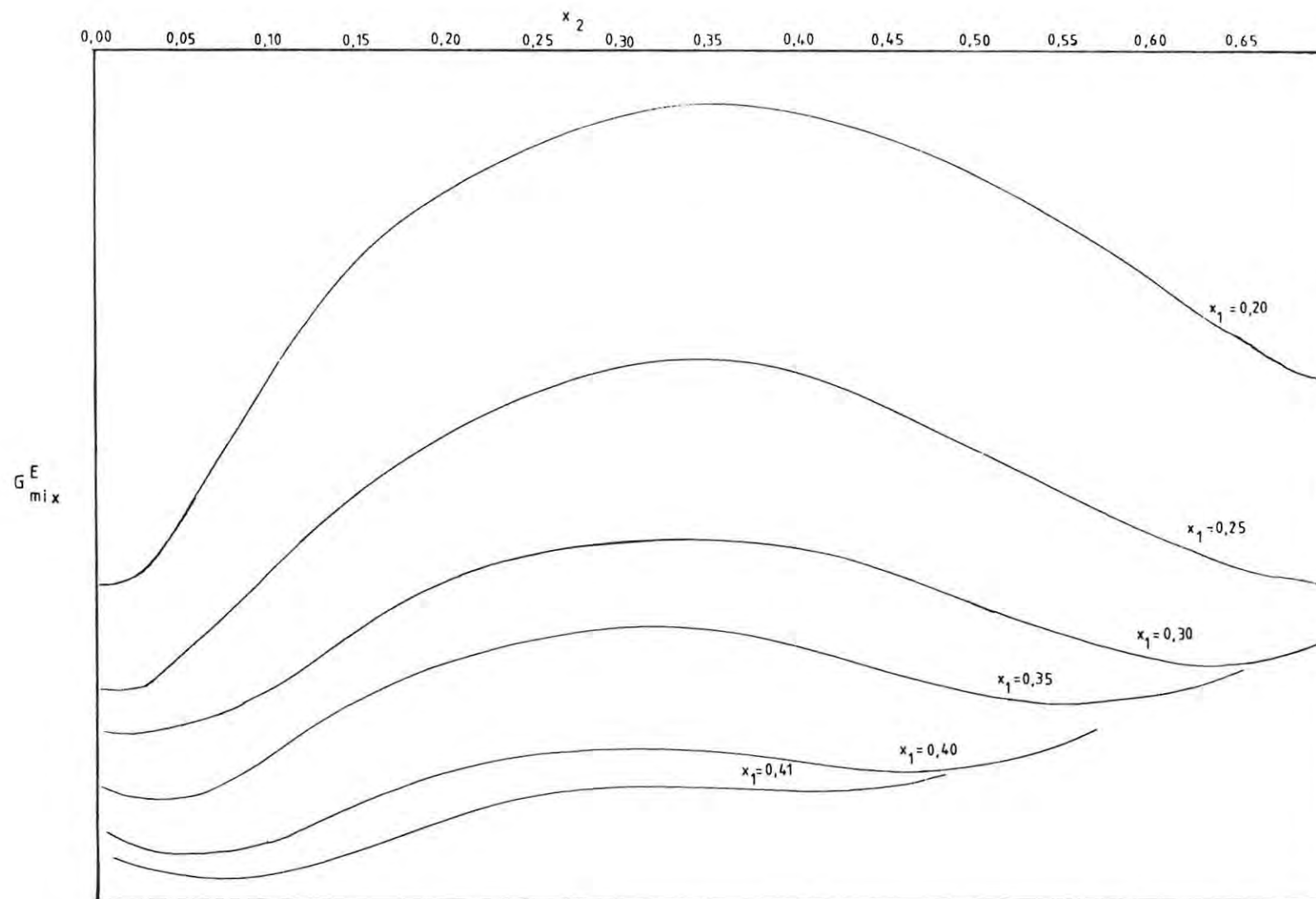
FIGURE 2.8 RESULTS OF G^E_{\text{MIX}} COMPUTATION FOR THE BENZENE-ETHANOL-WATER SYSTEM
