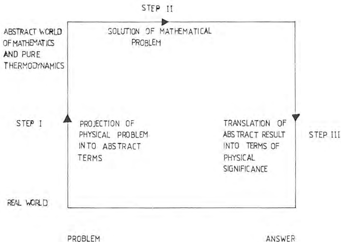
FIGURE 2.2 THREE-STEP APPLICATION OF THERMODYNAMICS TO PHASE-EQUILIBRIA PROBLEMS
