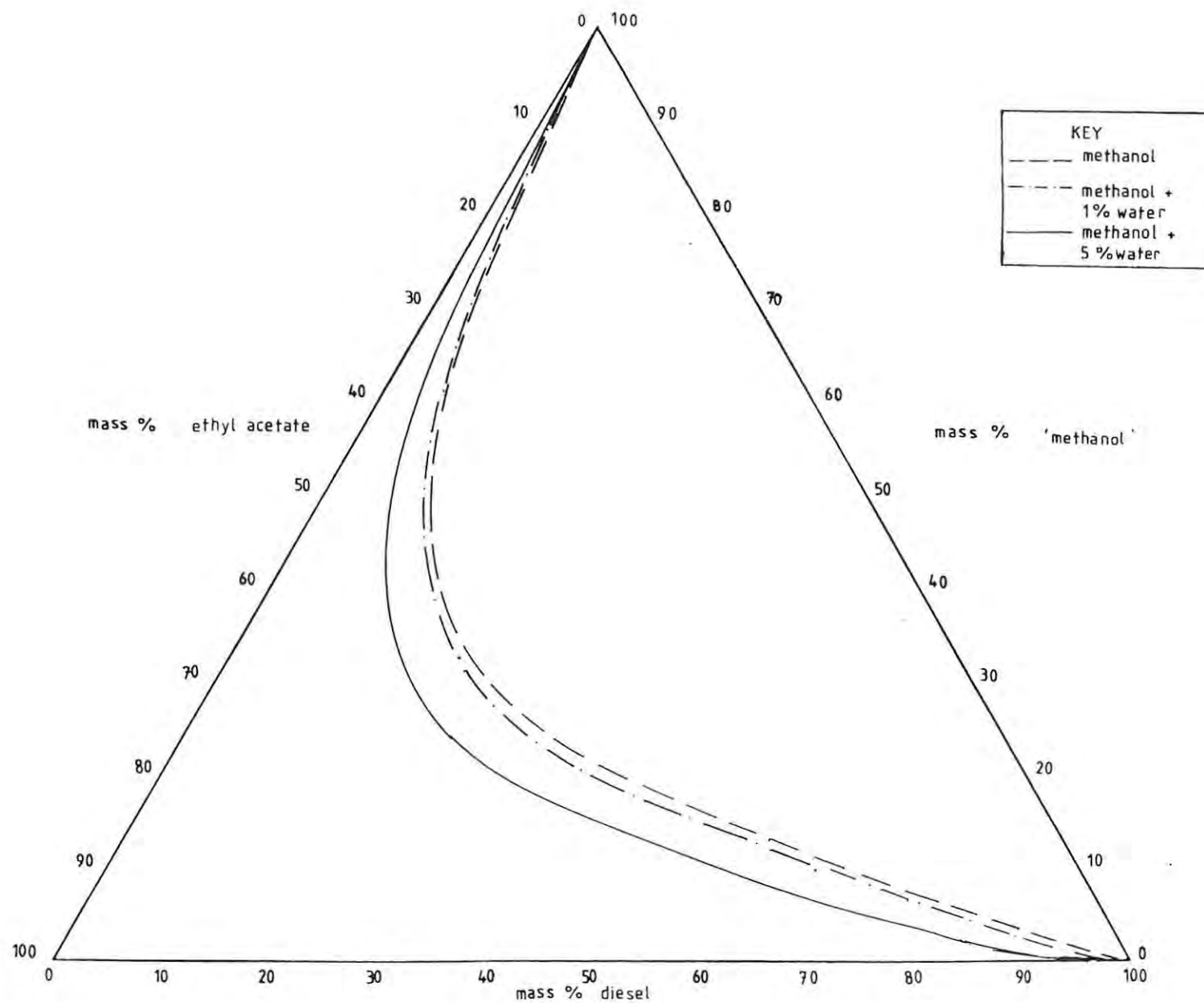
FIGURE 5.1 BINODAL CURVES FOR DIESEL-METHANOL-ETHYL ACETATE SYSTEMS
