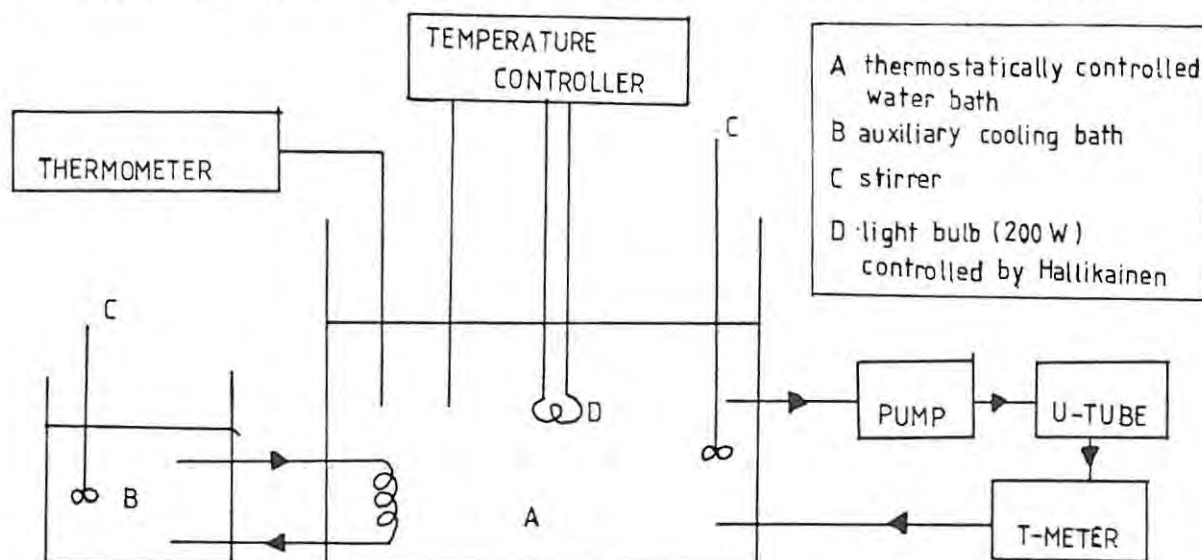
FIGURE 3.7 LABORATORY ARRANGEMENT FOR THE MEASURING OF V_M^E VALUES
