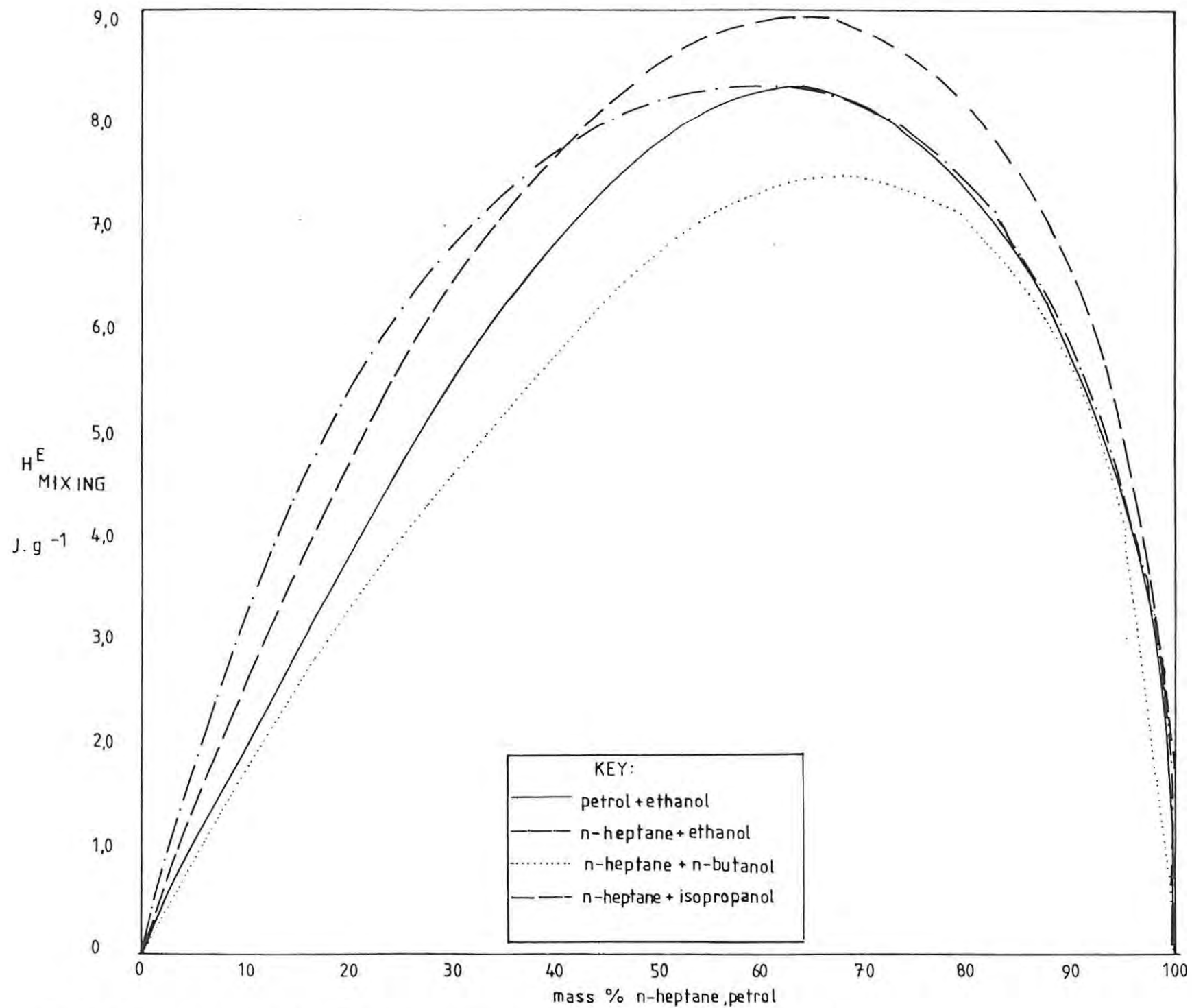
FIGURE 3.6 EXPERIMENTAL H_M^E RESULTS FOR N-HEPTANE + ALCOHOLS AT 298,15 K
