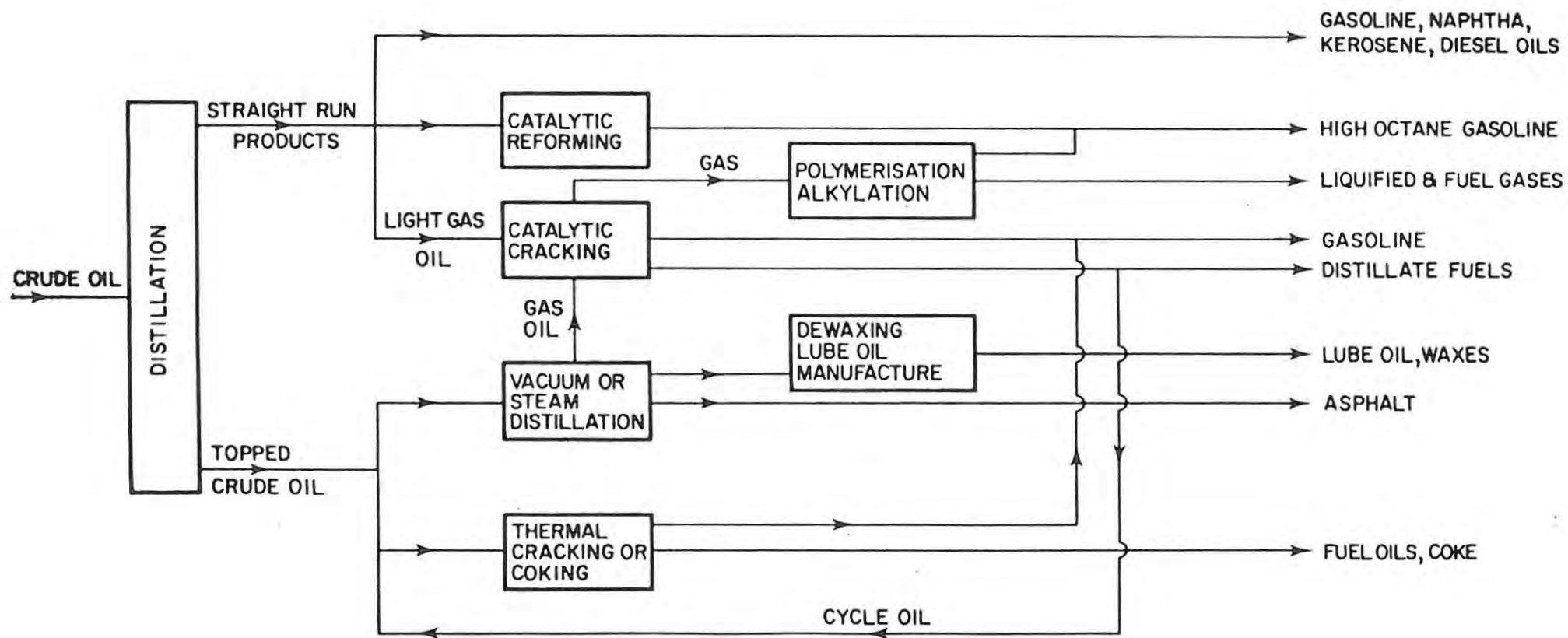
FIGURE 1.A.1 - BASIC REFINING OPERATIONS
