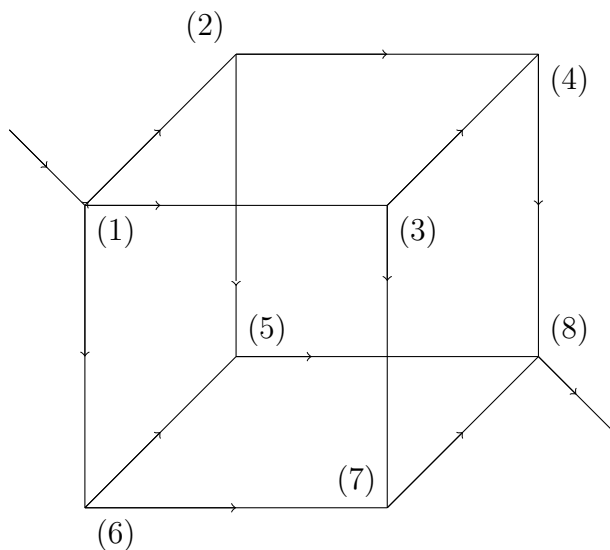
FIGURE 3. Electric circuit
