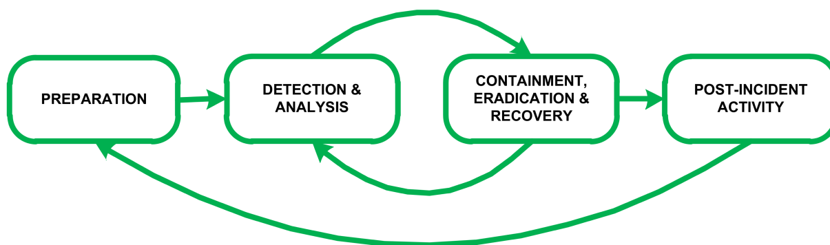
Figure 2.2: Security incident response life cycle (adapted from NIST [63])
