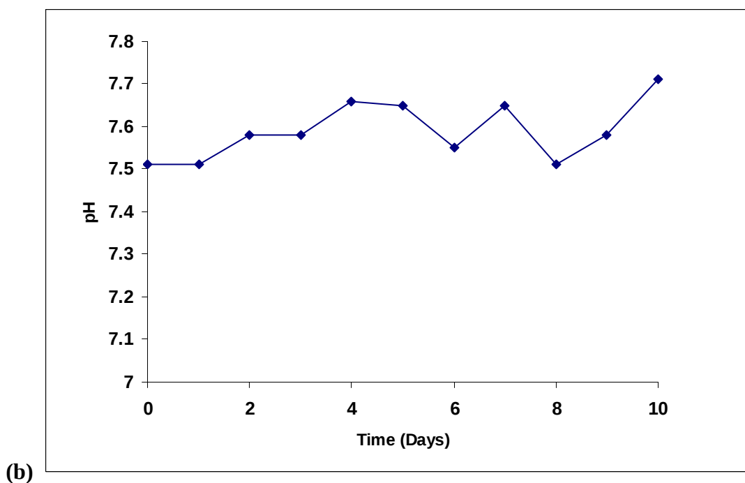
Figure 2.3: Batch bioreactor results of SRB metabolic activity during SRB growth at 30 °C. (a) Time course of sulphate reduction and concurrent sulphide production by SRB. The points are the means of the three triplicate and the error bars are \pm standard deviation of the triplicate values measured. Where error bars cannot be seen is because they are very small. (b) Corresponding pH profile during the time course.
