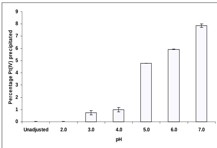
Figure 2.2: Effect of pH adjustment on initial platinum (IV) concentration of 16 mg.l -1 in the absence of SRB biomass. The points are the means \pm the standard deviation of triplicate values measured. The experiment was conducted at room temperature and initial platinum (IV) concentration was 16 mg.l -1 and incubation time was 1h.
