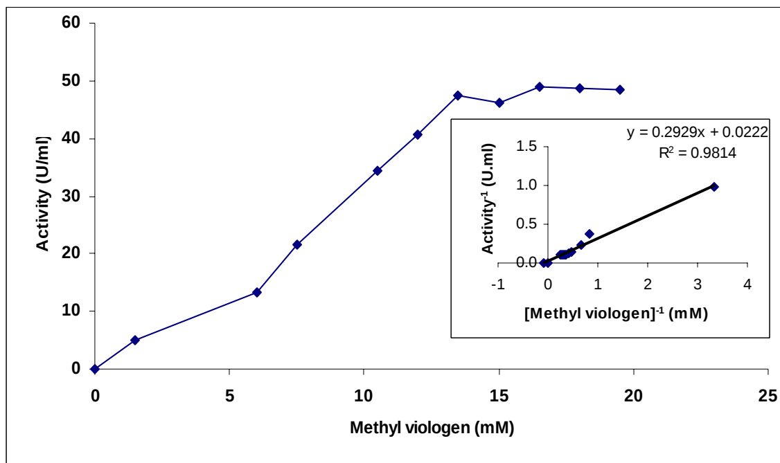
Figure 5.10: Dependence of the \text{H}_2 uptake by hydrogenase on the concentration of methyl viologen. (A) Michaelis-Menten plot of the reaction initial velocity ( V_o ) as a function of electron acceptor concentration (methyl viologen), and (B) Double-reciprocal (Lineweaver-Burk) plot of 1/V_o as a function of 1/[\text{methyl viologen}] .
