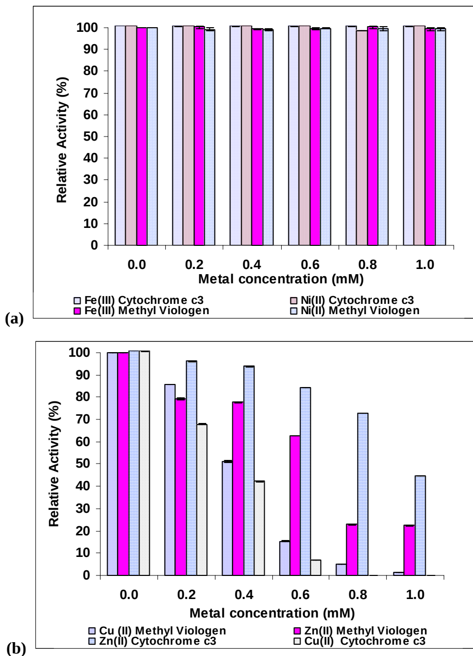
Figure 5.8: Effect of heavy metal ions on hydrogenase activity (a) Fe (III) and Ni (II), and (b) Cu (II) and Zn (II). Net enzymatic activity was obtained by subtracting non-enzymatic activity measured in presence of N 2 (control) instead of hydrogen.
