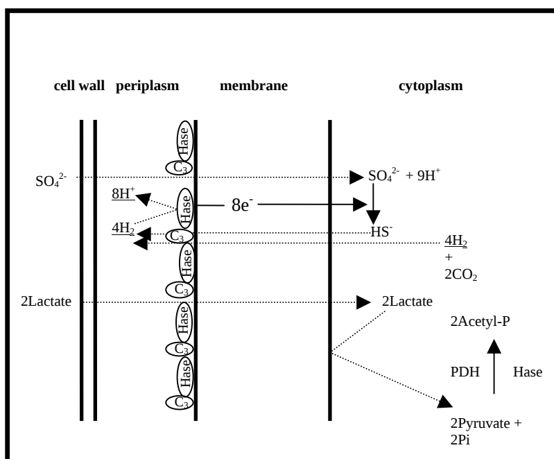
Figure 1.4: Hydrogen cycling in Desilfovibrio vulgaris [ \text{C}_3 =Cytochrome \text{C}_3 ; \text{Hase} =Hydrogenase; \text{PDH} = pyruvate dehydrogenase] (Odom and Peck, 1984).
