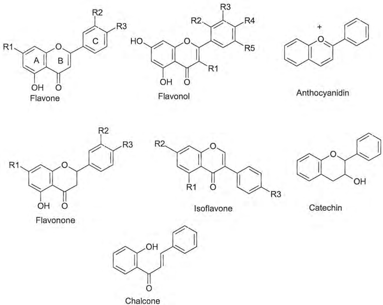
Fig. 4.2. Structures of the main flavonoid subclasses (Adapted from de Rijke et al. , 2006).
