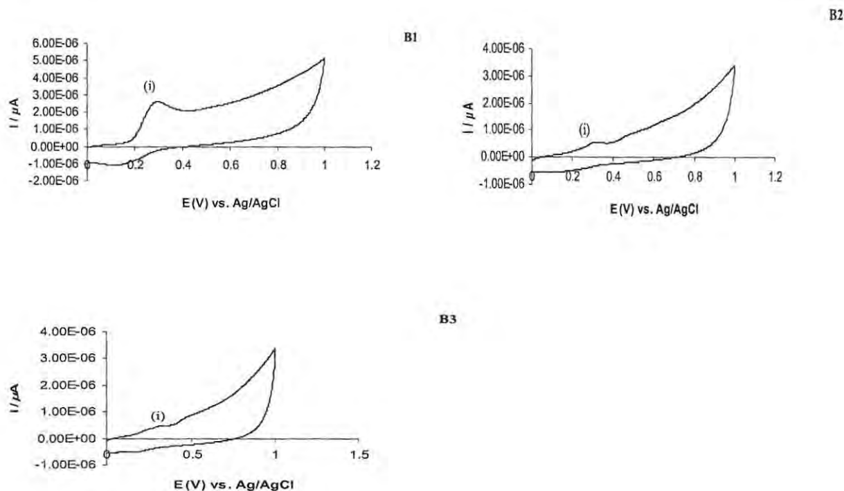
Fig. 4.7. Cyclic voltammograms of B. elliptica solvent extracts (107.4 \mu\text{g/ml} ) in 0.2 M Tris-HCl buffer (pH 7). Scan rate at 100 mV/sec. B1 (methanol extract), B2 (ethyl acetate extract) and B3 (chloroform extract).
