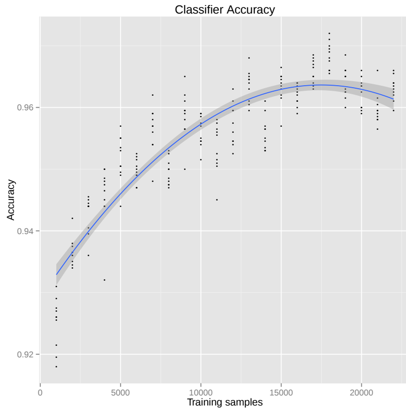
(a) Accuracy. Peaking at dataset #18.
