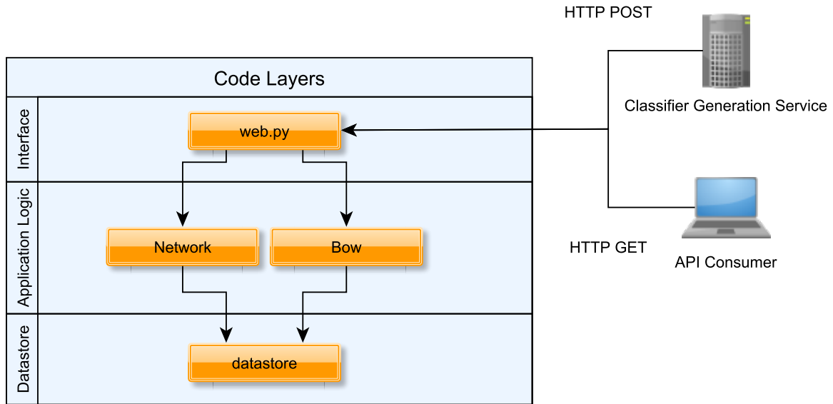
Figure 4.8: Layout of code structure within the Classifier Distribution Service (CDS).
