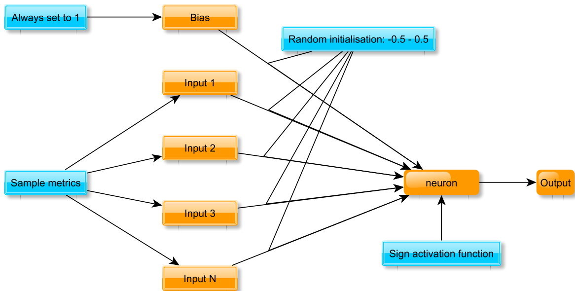
Figure 3.1: Structure and initialisation of the classifier.
