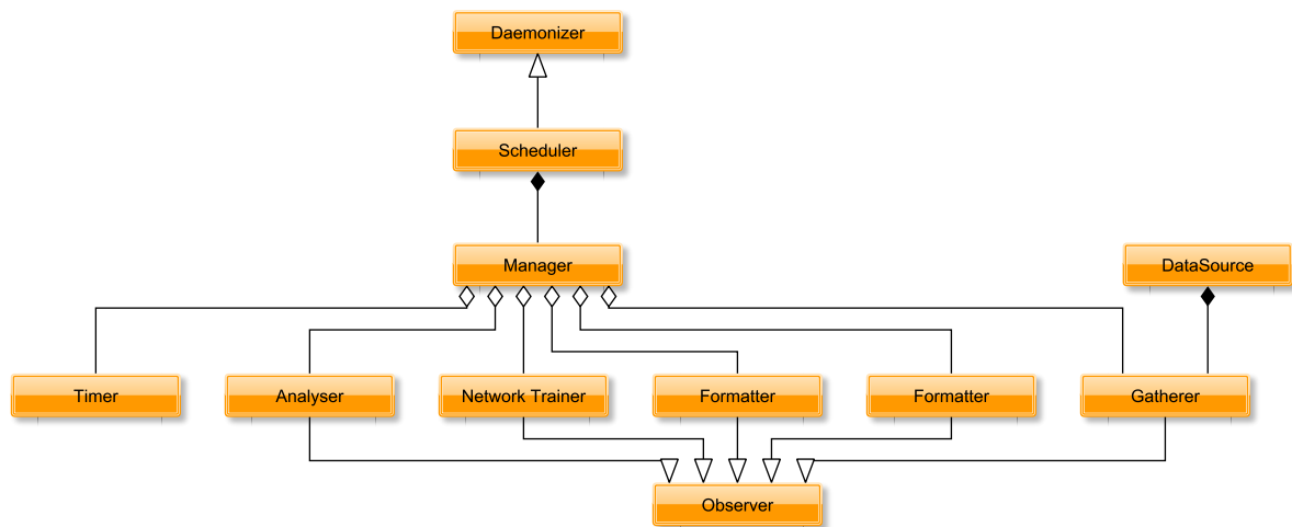
Figure 4.3: Overview of Python framework implementation.
