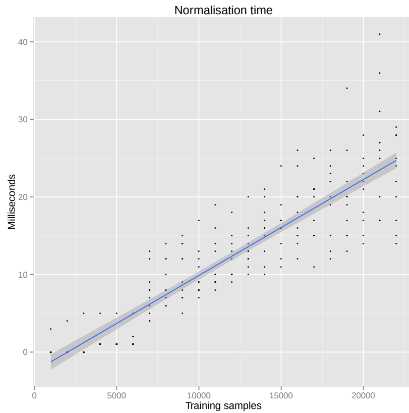
(b) Normalisation time.
