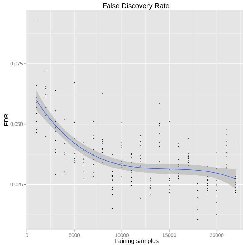
(c) False Discovery Rate (FDR).
