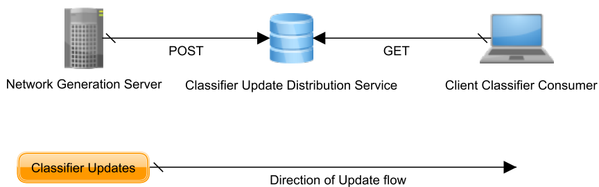
Figure 4.6: Flow of updates via Classifier Distribution Service (CDS).
