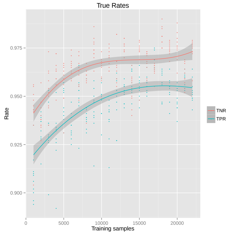
(a) True Positive Rate (TPR) and True Negative Rate (TNR).
