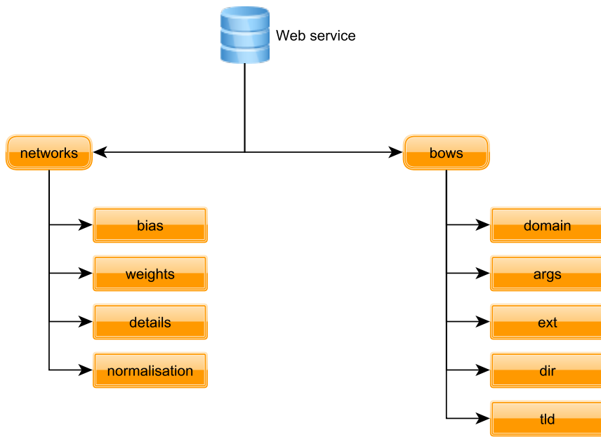
Figure 4.7: Logical resources available in Classifier Distribution Service (CDS).
