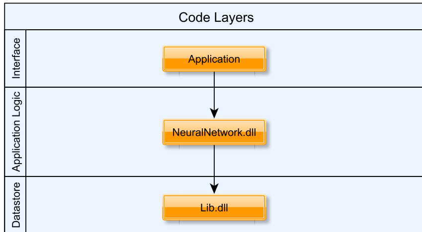
Figure 4.5: Layout of code structure withing the Classifier Generation Service (CGS).
