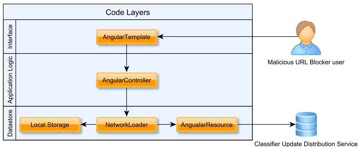
Figure 4.10: Layout of code structure within Net Defence.
