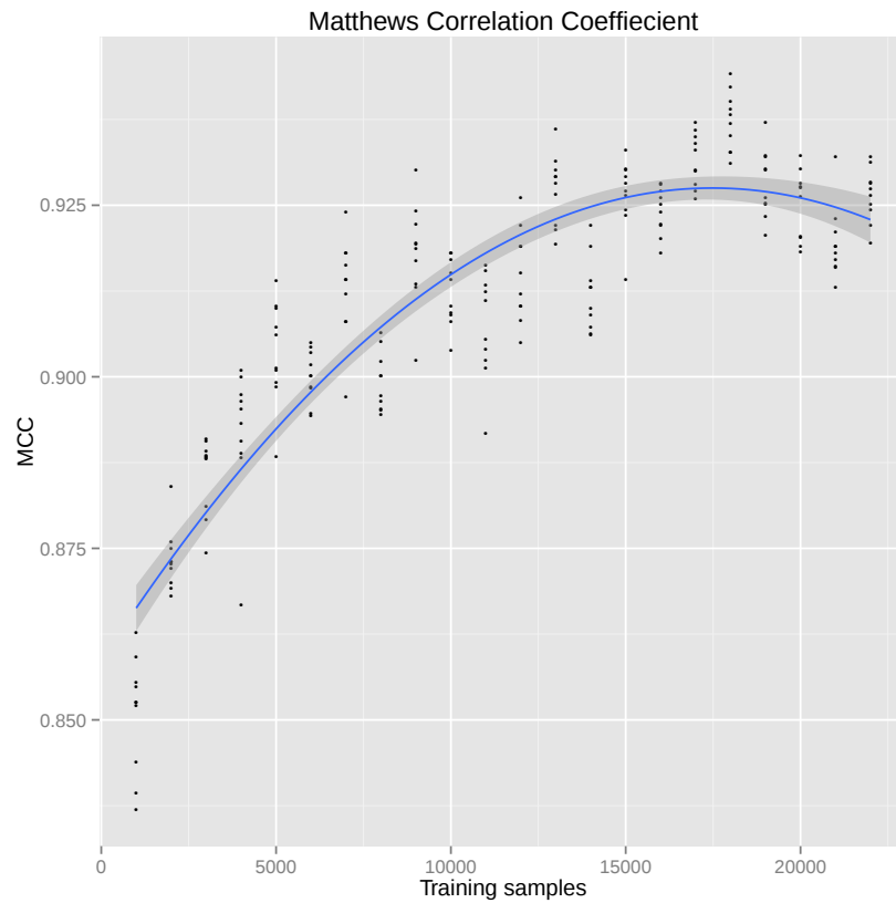
(c) Matthews Correlation Coefficient (MCC). Peaking at dataset #18.
