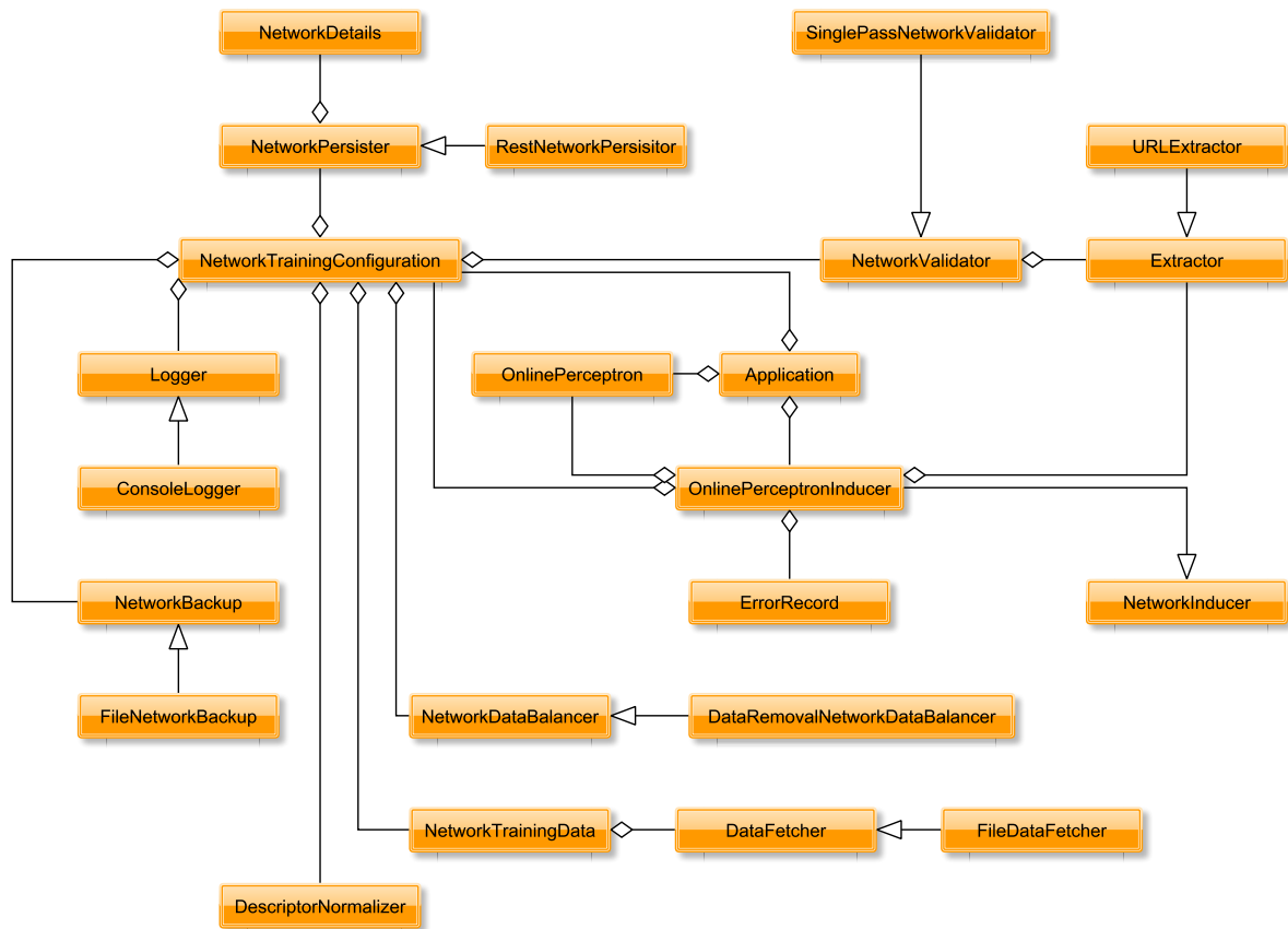
Figure 4.4: Overview of the Classifier Generation Service (CGS).
