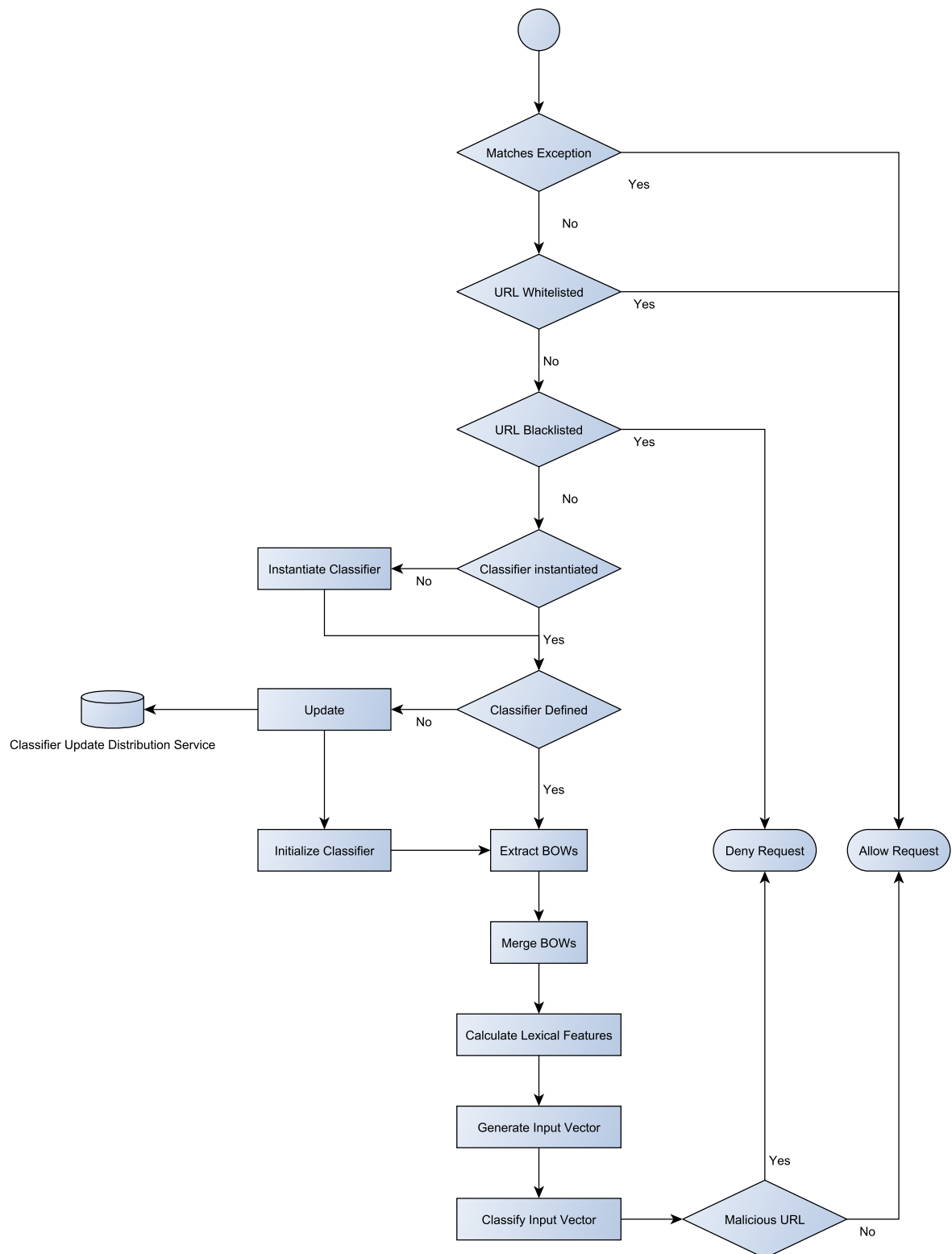
Figure 4.11: Flow diagram of the Net Defence classification algorithm.
