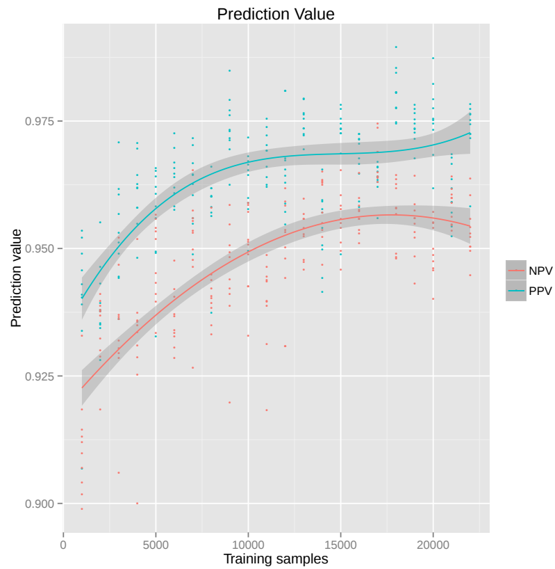
(b) Positive Prediction Value (PPV) and Negative Prediction Value (NPV).
