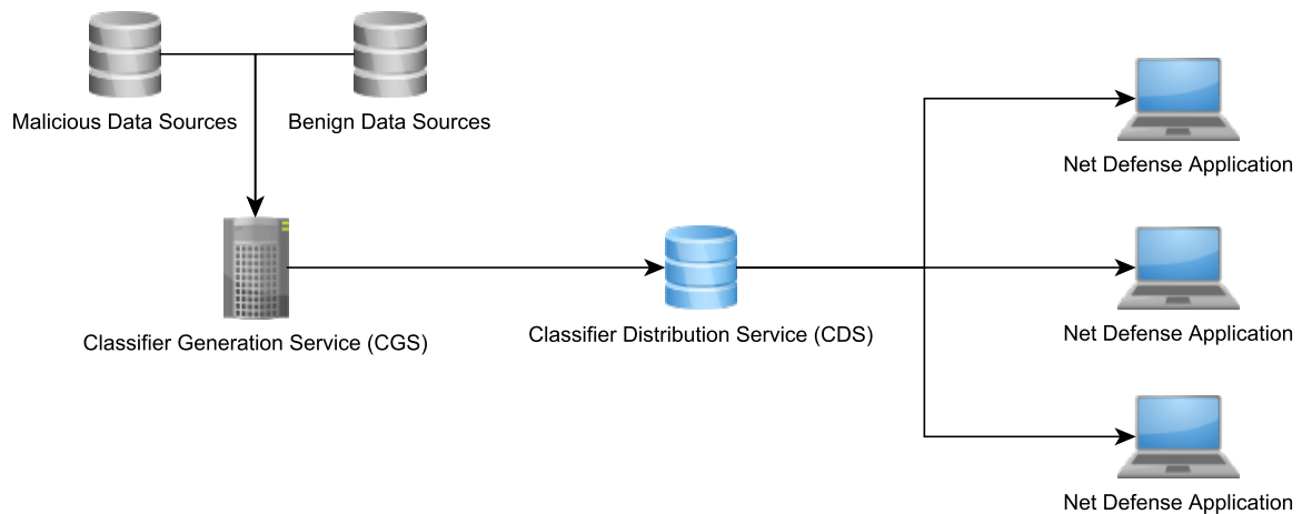
Figure 4.1: High-level infrastructure layout.
