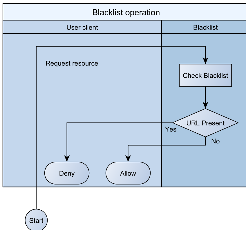
Figure 2.3: Blackhole list transaction.
