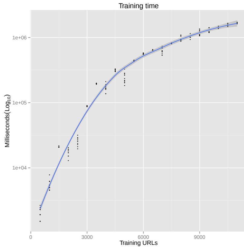
(c) Training time.
