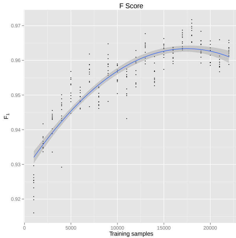
(b) F 1 score. Peaking at dataset #18.
