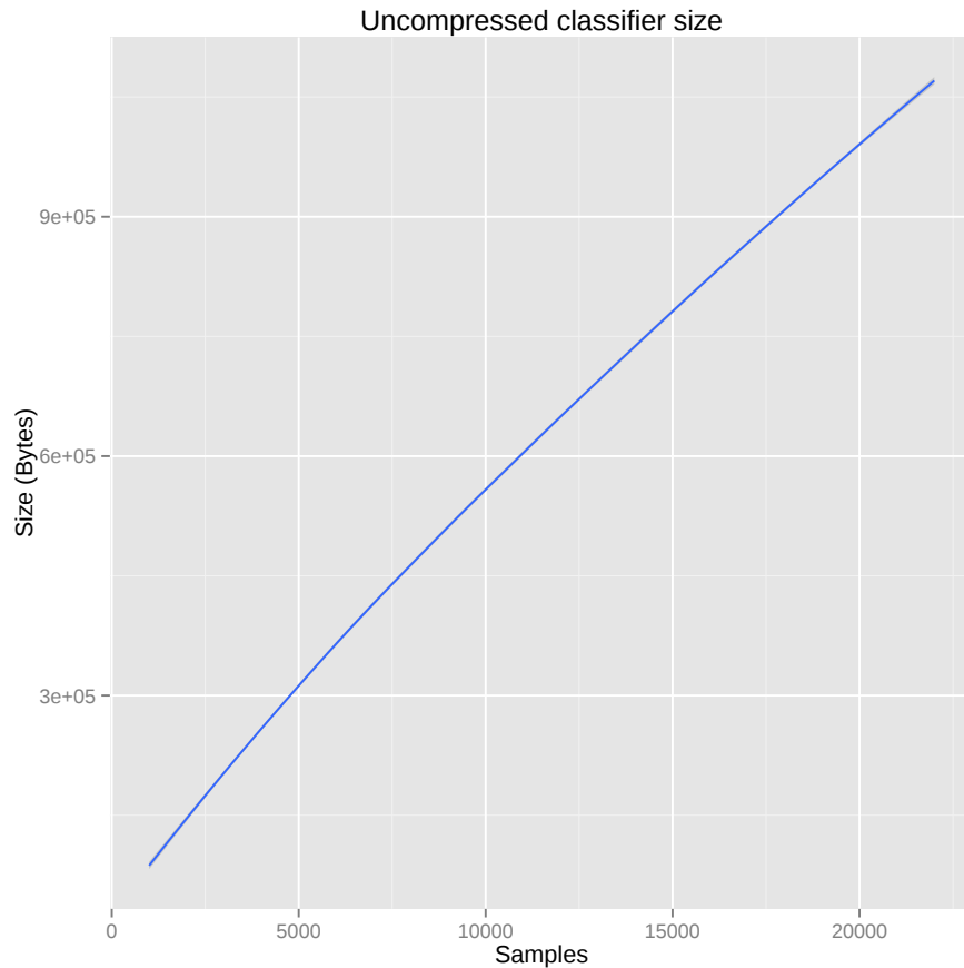
Figure 5.5: Uncompressed size of classifiers based on the number of training samples used.
