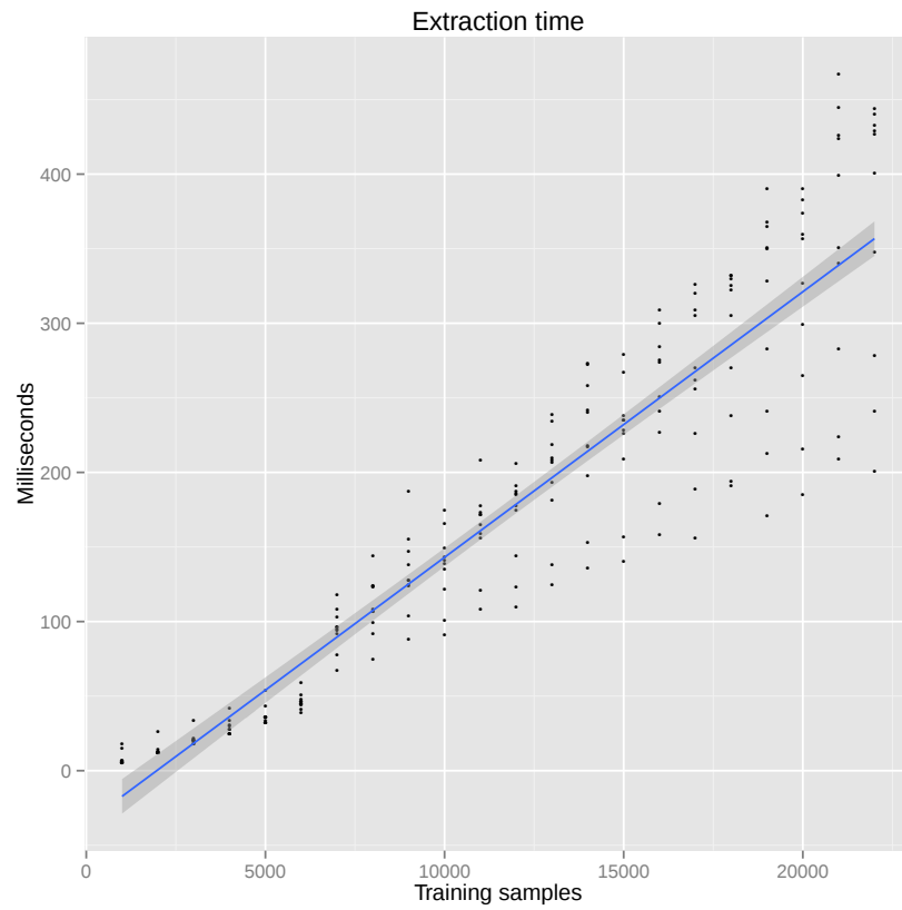
(a) Extraction time.
