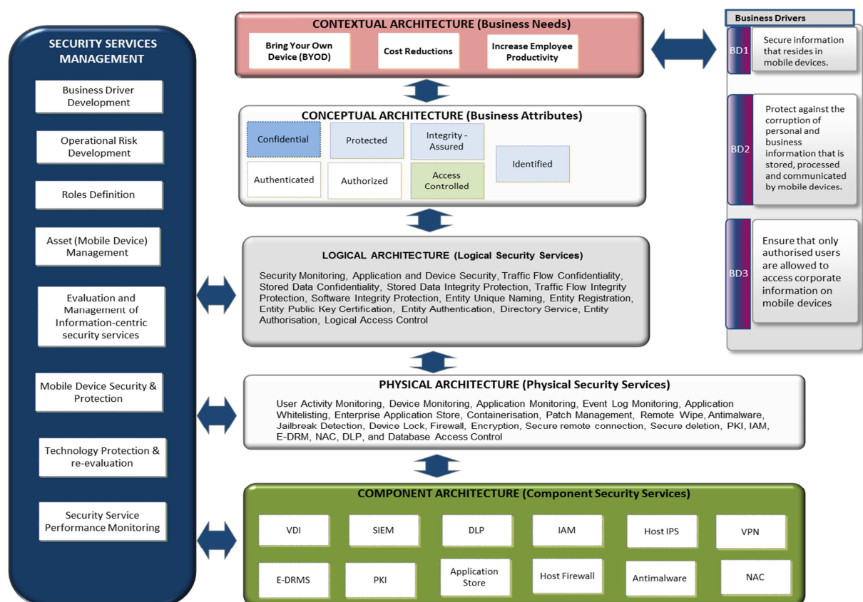
Figure 3-1: Utopian Reference Architecture Framework Based on SABSA
