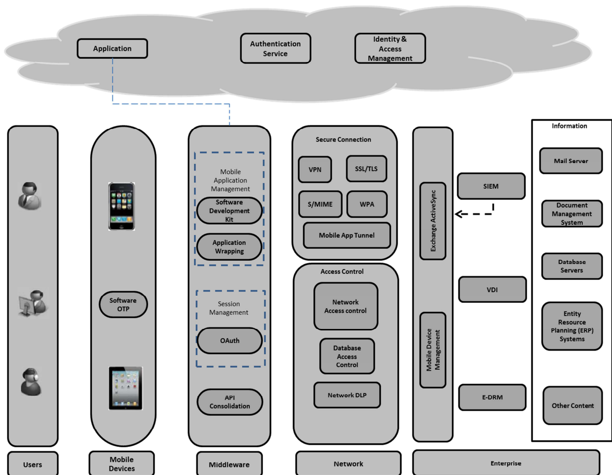
Figure 5-4: Derived Mobile Security Architecture Model
