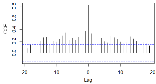
Cross-correlation correlogram of sensor 196-a vs. 196-b using daily ICMP packet count
