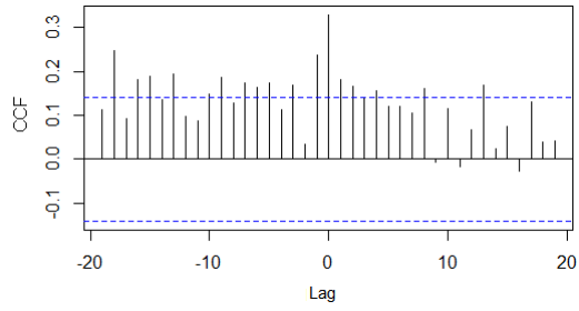
Cross-correlation correlogram of sensor 146-a vs. 196-b using daily ICMP packet count
