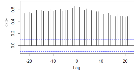
Cross-correlation correlogram of sensor 155-a vs. 196-c using daily ICMP packet count
