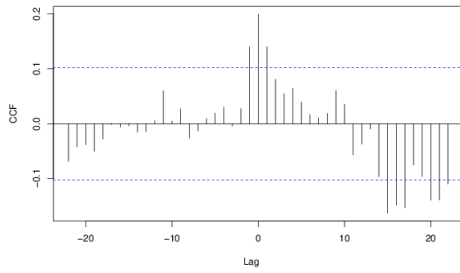
Cross-correlation correlogram of sensor 196-a vs. 155-a using daily packet count
