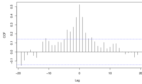
Cross-correlation correlogram of sensor 196-a vs. 196-b using daily packet count
