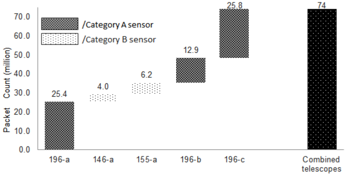
Figure 3.3: Packet count per network telescope sensor between 20 May 2011 and 20 May 2012
