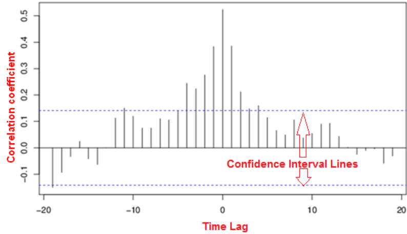
Figure 5.1: Correlogram example
