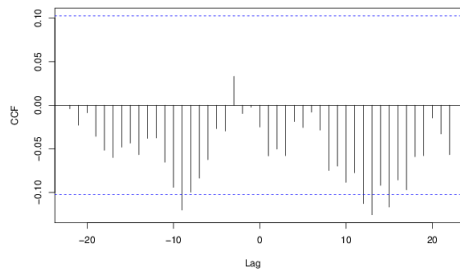
Cross-correlation correlogram of sensor 146-a vs. 196-c using daily packet count
