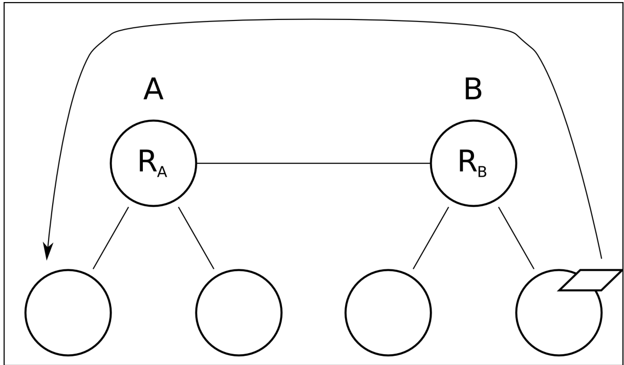
Figure 5.3: Simulating Routing
