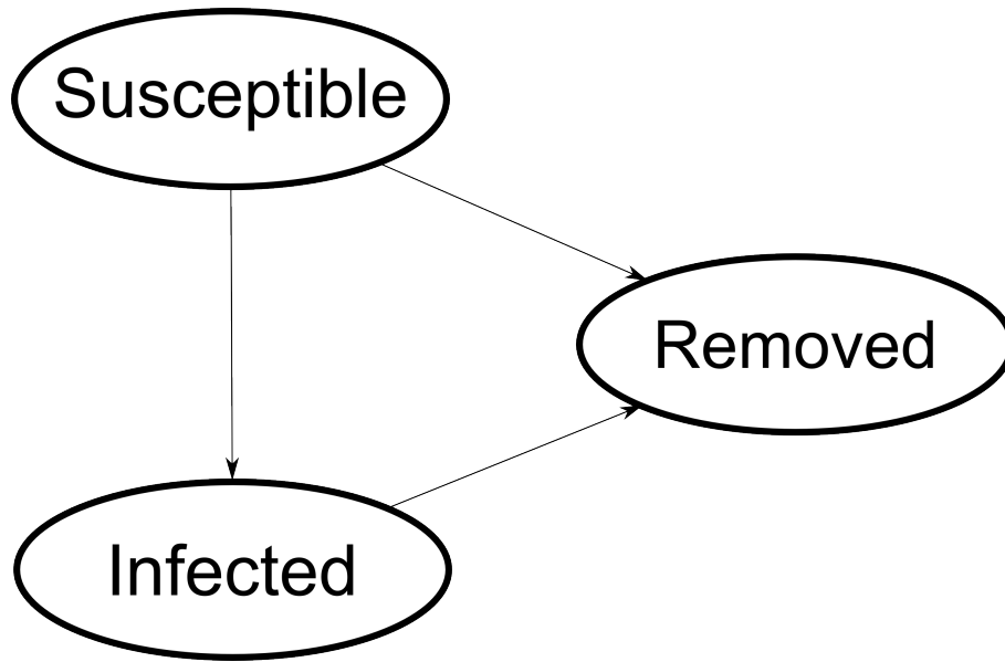
Figure 2.2: Susceptible-Infected-Removed model
