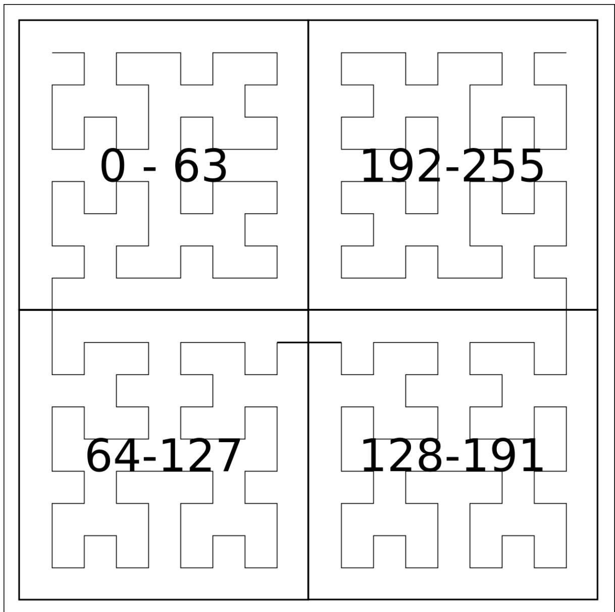
Figure 6.1: Order 4 Hilbert Curve
