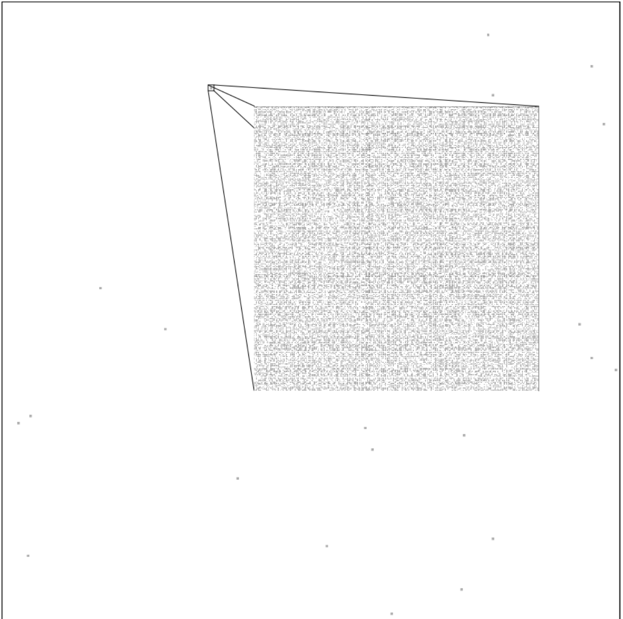
Figure 6.10: Welchia Hilbert with Magnification
