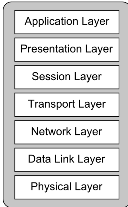
Figure 2.1: OSI Stack
