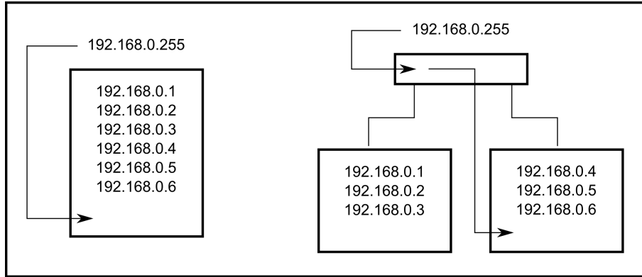
Figure 4.1: Distributed Memory Allocation System
