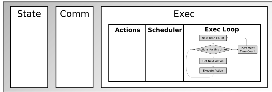
Figure 3.6: Execution Component of Simulator (Main Execution Loop)
