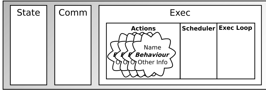
Figure 3.4: Execution Component of Simulator (Action Subcomponent)
