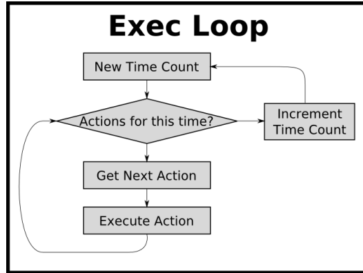
Figure 3.7: Main Execution Loop
