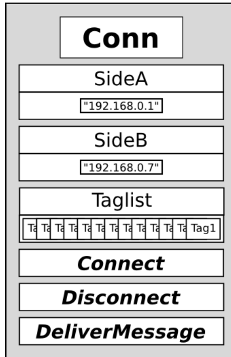
Figure 3.9: Connection Module Diagram
