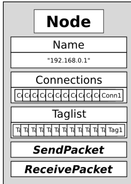
Figure 3.8: Node Module Diagram
