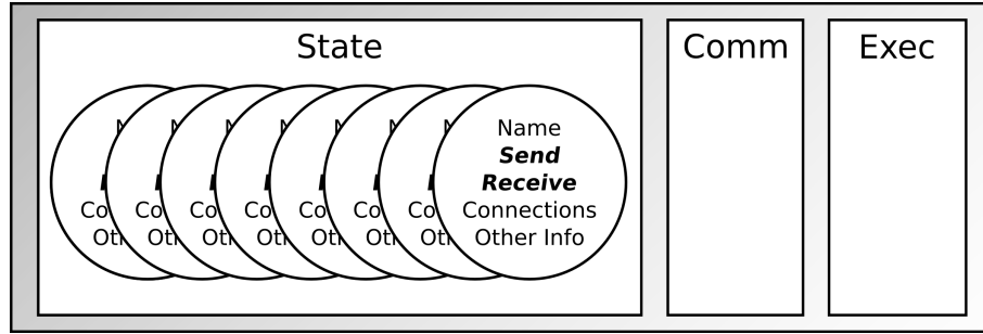
Figure 3.2: State Component of Simulator
