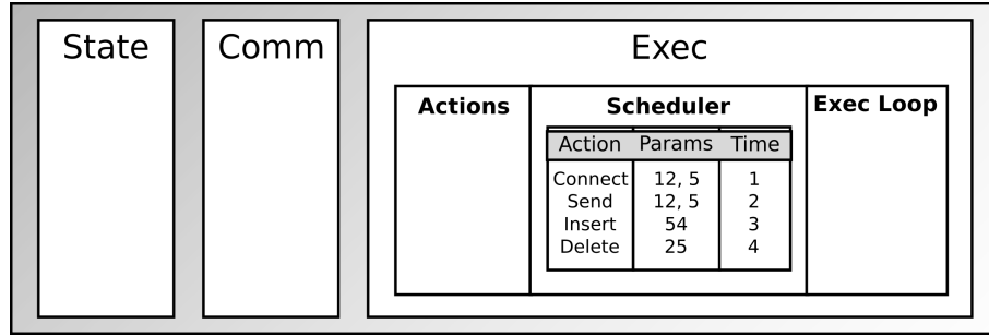
Figure 3.5: Execution Component of Simulator (Scheduler Subcomponent)
