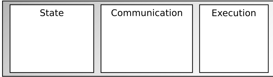
Figure 3.1: Simulator Subcomponents
