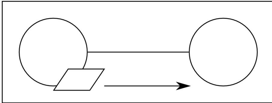
Figure 5.2: Simulating Connectivity
